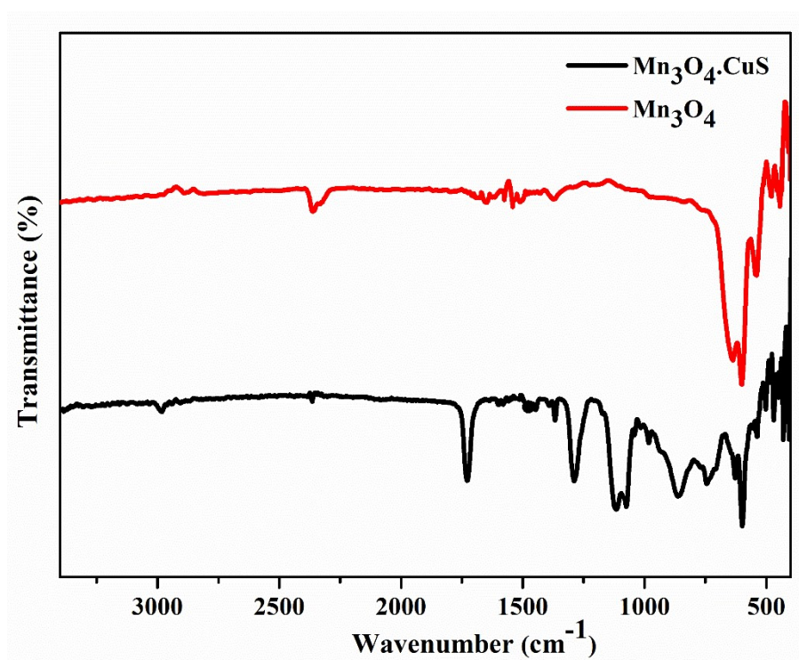
Figure S1. FTIR Spectroscopy of Mn 3 O 4 and Mn 3 O 4 ·CuS Nanocomposites.
