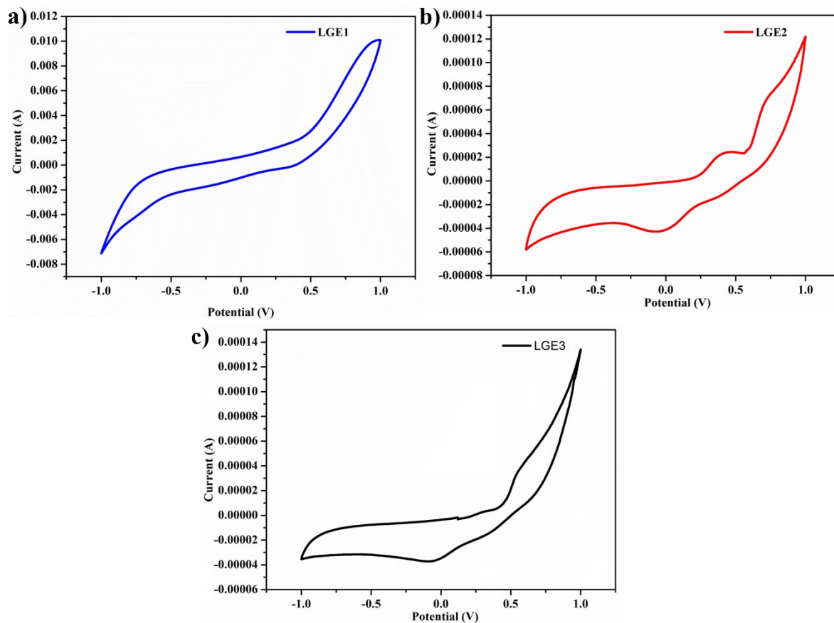
Figure S4. Cyclic Voltammetry spectrum of a) LGE1 b) LGE2 c) LGE3.
