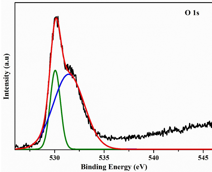
Figure S2a. XPS image of O1s.
