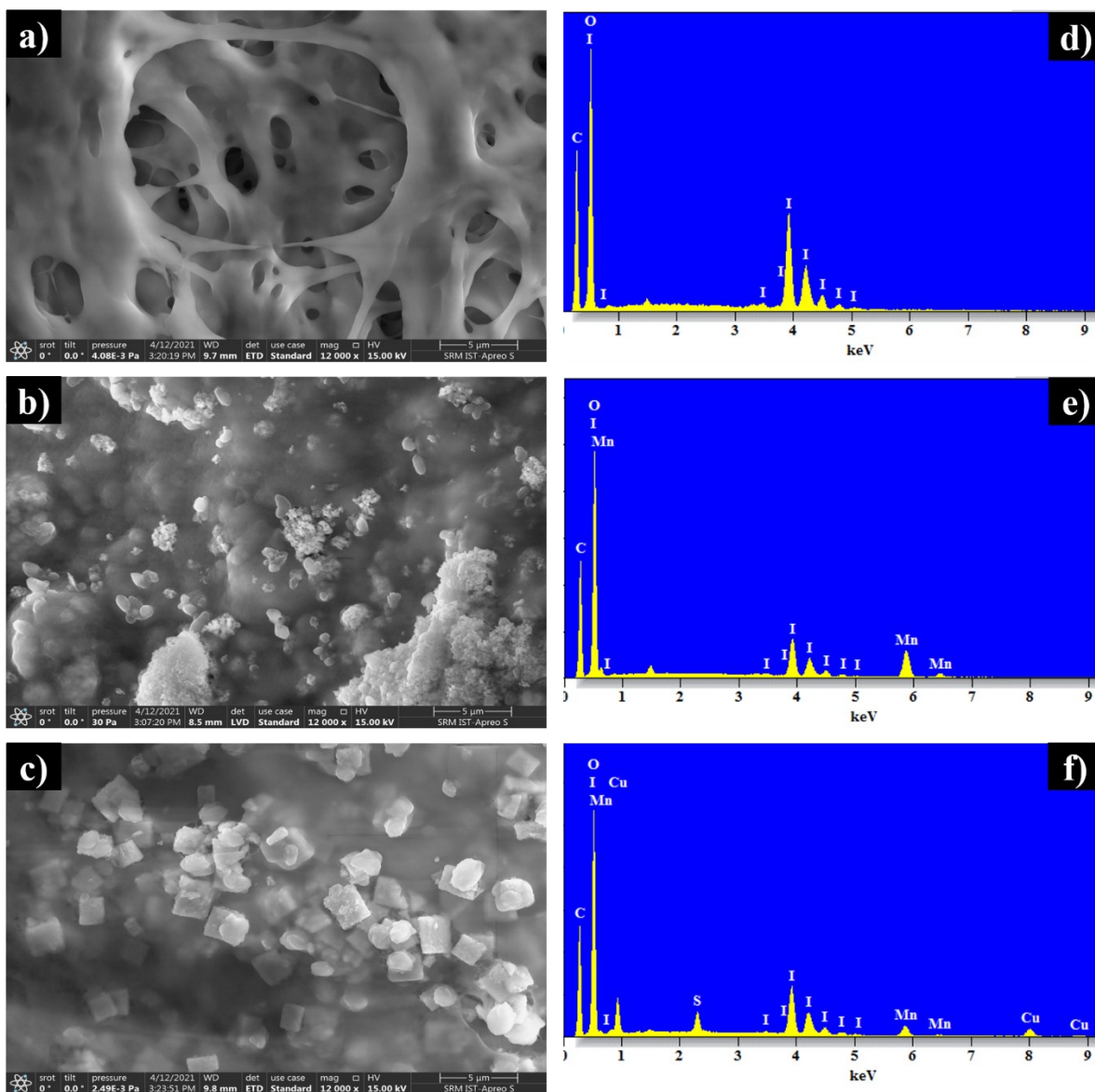
Figure S3. SEM images of a) LGE1 b) LGE2 c) LGE3, EDX images of d) LGE1 e) LGE2 f) LGE3.
