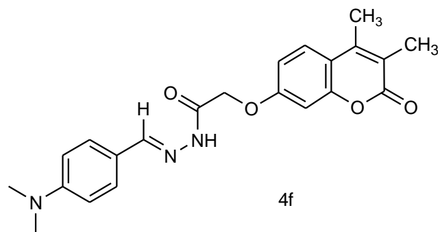
2-((3,4-dimethyl-2-oxo-2H-chromen-7-yl)oxy)-N'-(4-(dimethylamino)benzylidene)acetohydrazide
