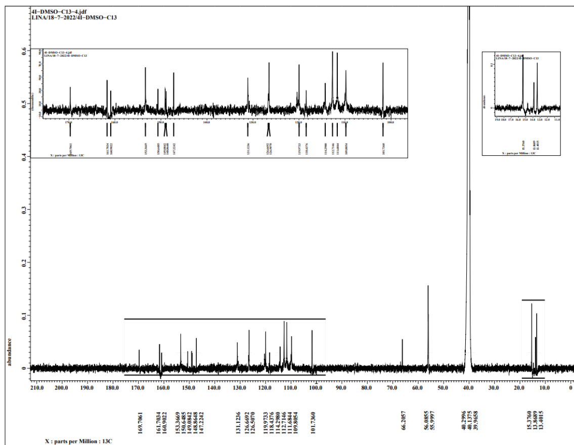
N'-(1-(3,4-dimethoxyphenyl)ethylidene)-2-((3,4-dimethyl-2-oxo-2H-chromen-7-yl)oxy)acetohydrazide
