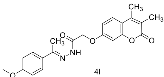
2-((3,4-dimethyl-2-oxo-2H-chromen-7-yl)oxy)-N'-(1-(4-methoxyphenyl)ethylidene)acetohydrazide
