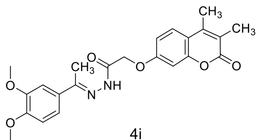
N'-(1-(3,4-dimethoxyphenyl)ethylidene)-2-((3,4-dimethyl-2-oxo-2H-chromen-7-yl)oxy)acetohydrazide
