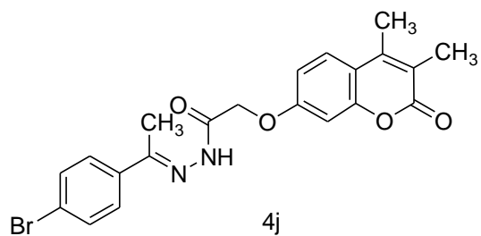
N'-(1-(4-bromophenyl)ethylidene)-2-((3,4-dimethyl-2-oxo-2H-chromen-7-yl)oxy)acetohydrazide
