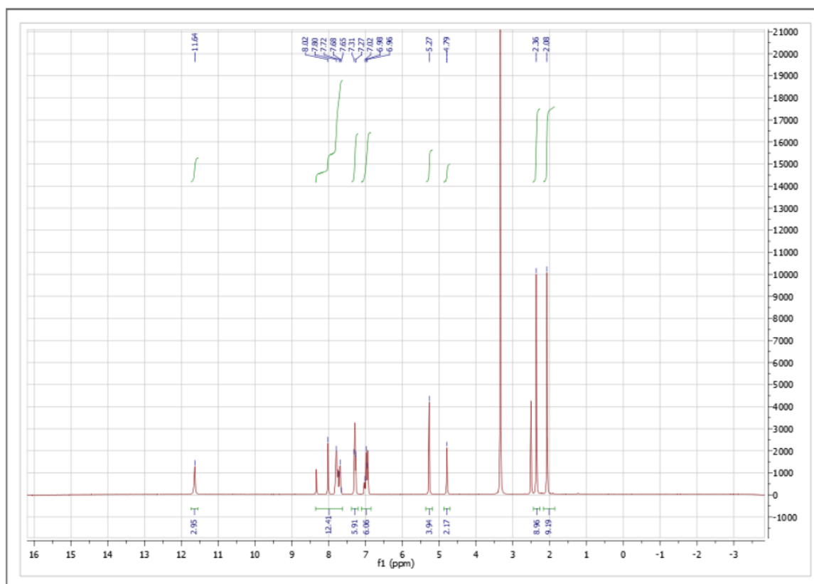
2-((3,4-dimethyl-2-oxo-2H-chromen-7-yl)oxy)-N'-(4-fluorobenzylidene)acetohydrazide
