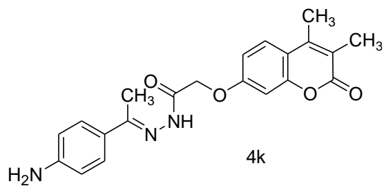
N'-(1-(4-aminophenyl)ethylidene)-2-((3,4-dimethyl-2-oxo-2H-chromen-7-yl)oxy)acetohydrazide
