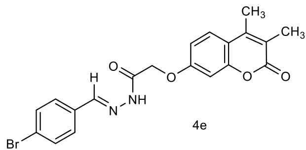
N'-(4-bromobenzylidene)-2-((3,4-dimethyl-2-oxo-2H-chromen-7-yl)oxy)acetohydrazide
