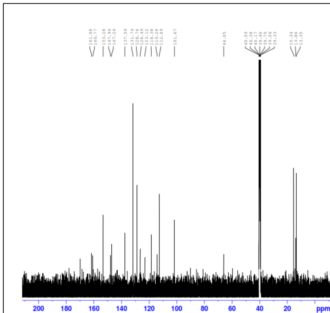
N'-(1-(4-bromophenyl)ethylidene)-2-((3,4-dimethyl-2-oxo-2H-chromen-7-yl)oxy)acetohydrazide
