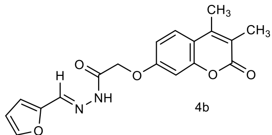
2-((3,4-dimethyl-2-oxo-2H-chromen-7-yl)oxy)-N'-(furan-2-ylmethylene)acetohydrazide
