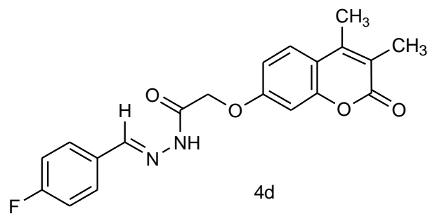
2-((3,4-dimethyl-2-oxo-2H-chromen-7-yl)oxy)-N'-(4-fluorobenzylidene)acetohydrazide
