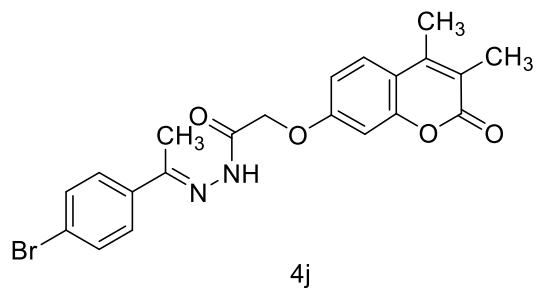
N'-(1-(4-bromophenyl)ethylidene)-2-((3,4-dimethyl-2-oxo-2H-chromen-7-yl)oxy)acetohydrazide
