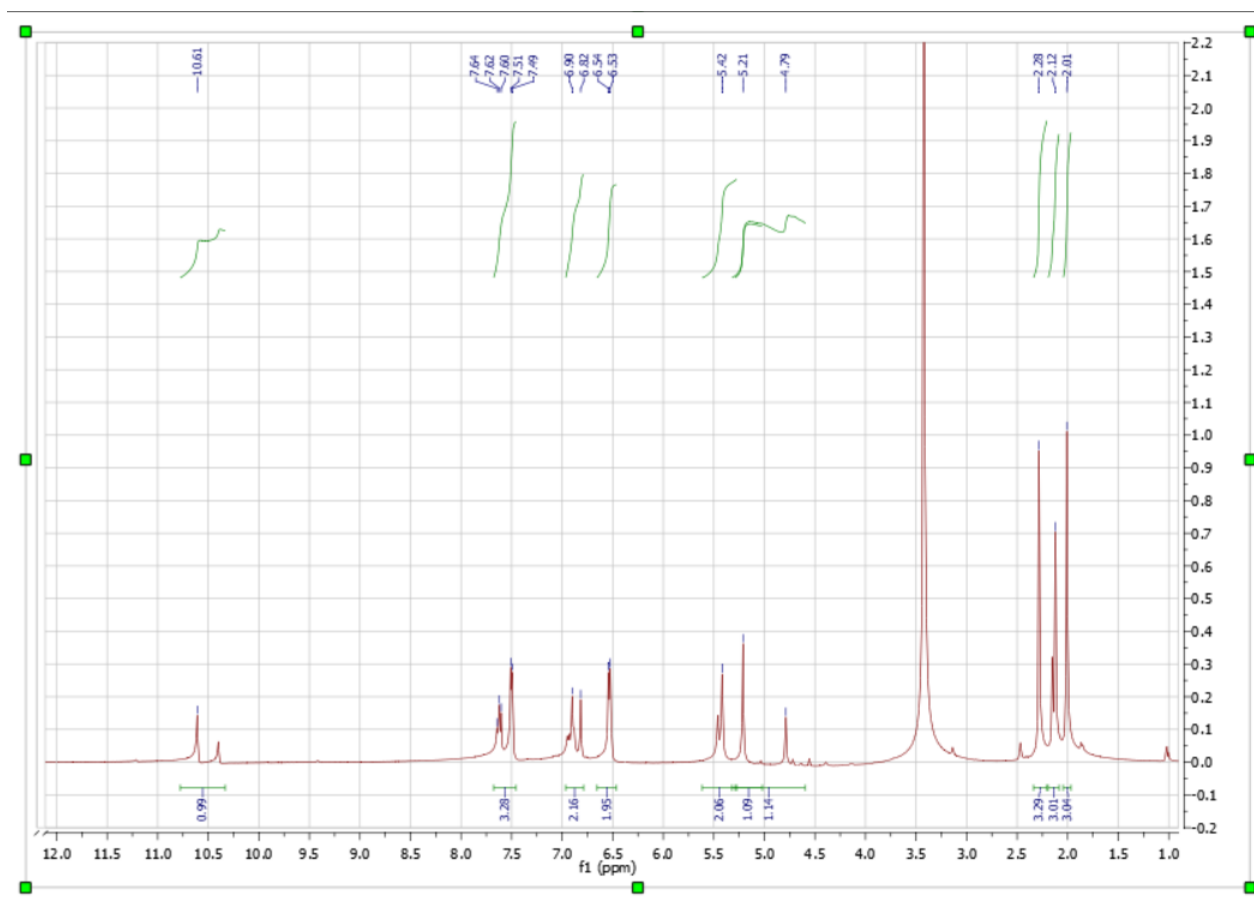
N'-(1-(4-aminophenyl)ethylidene)-2-((3,4-dimethyl-2-oxo-2H-chromen-7-yl)oxy)acetohydrazide
