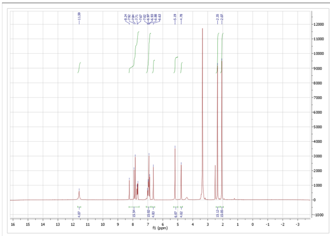
2-((3,4-dimethyl-2-oxo-2H-chromen-7-yl)oxy)-N'-(furan-2-ylmethylene)acetohydrazide
