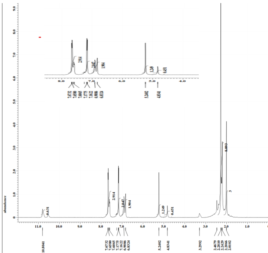
2-((3,4-dimethyl-2-oxo-2H-chromen-7-yl)oxy)-N'-(1-(p-tolyl)ethylidene)acetohydrazide
