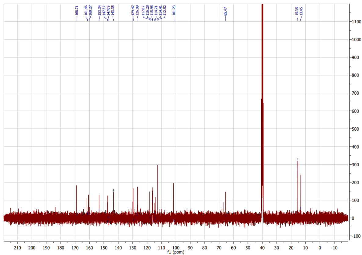
N'-(4-bromobenzylidene)-2-((3,4-dimethyl-2-oxo-2H-chromen-7-yl)oxy)acetohydrazide
