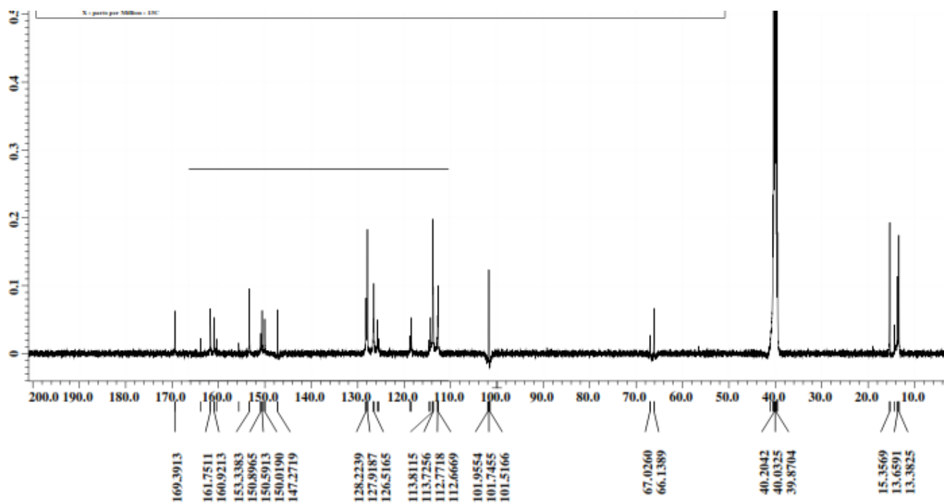
N'-(1-(4-aminophenyl)ethylidene)-2-((3,4-dimethyl-2-oxo-2H-chromen-7-yl)oxy)acetohydrazide
