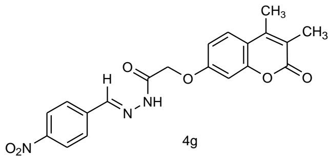
2-((3,4-dimethyl-2-oxo-2H-chromen-7-yl)oxy)-N'-(4-nitrobenzylidene)acetohydrazide
