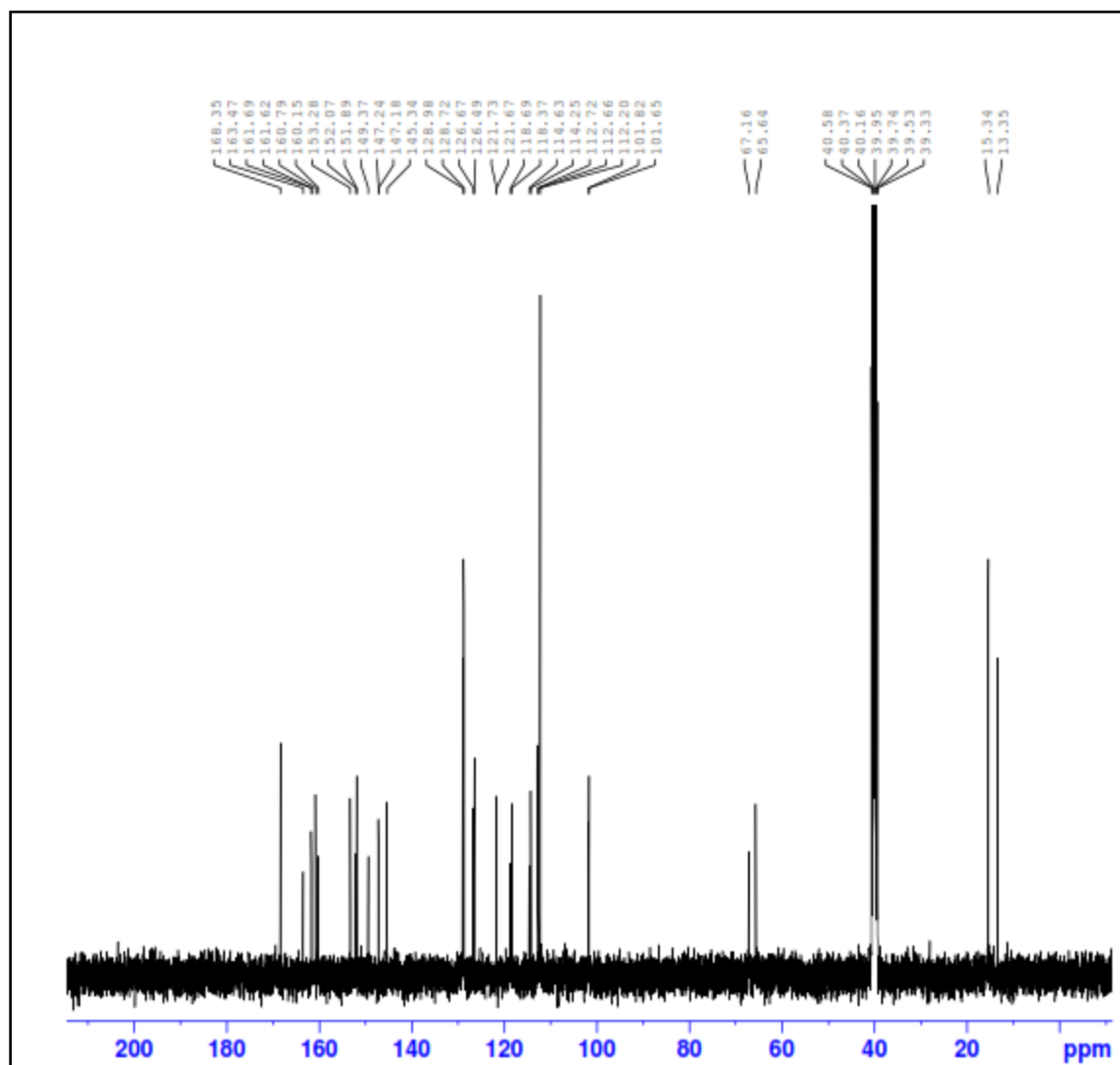
2-((3,4-dimethyl-2-oxo-2H-chromen-7-yl)oxy)-N'-(4-(dimethylamino)benzylidene)acetohydrazide
