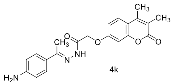
N'-(1-(4-aminophenyl)ethylidene)-2-((3,4-dimethyl-2-oxo-2H-chromen-7-yl)oxy)acetohydrazide
