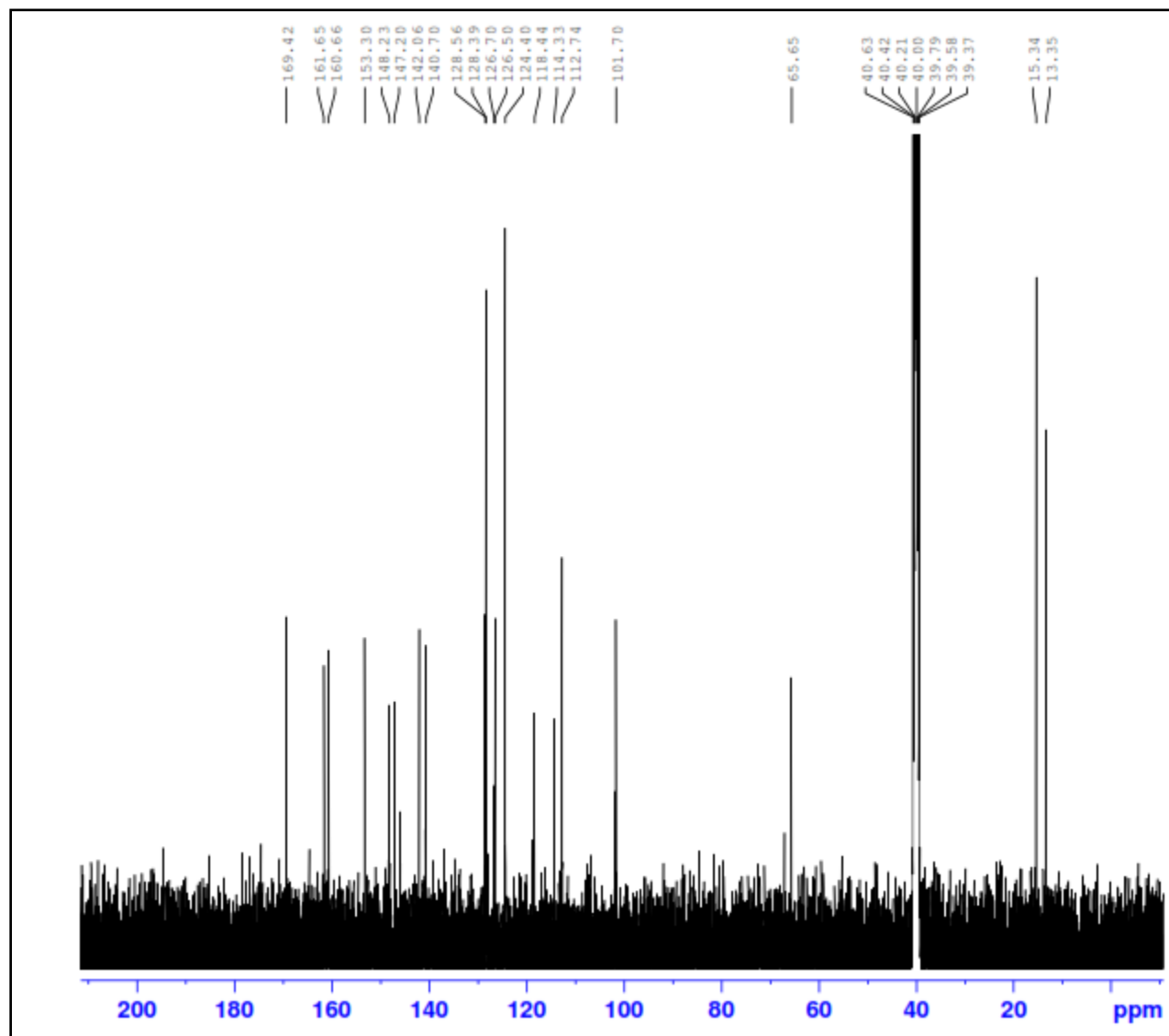
2-((3,4-dimethyl-2-oxo-2H-chromen-7-yl)oxy)-N'-(4-nitrobenzylidene)acetohydrazide
