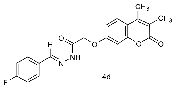
2-((3,4-dimethyl-2-oxo-2H-chromen-7-yl)oxy)-N'-(4-fluorobenzylidene)acetohydrazide
