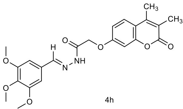
2-((3,4-dimethyl-2-oxo-2H-chromen-7-yl)oxy)-N'-(3,4,5-trimethoxybenzylidene)acetohydrazi
