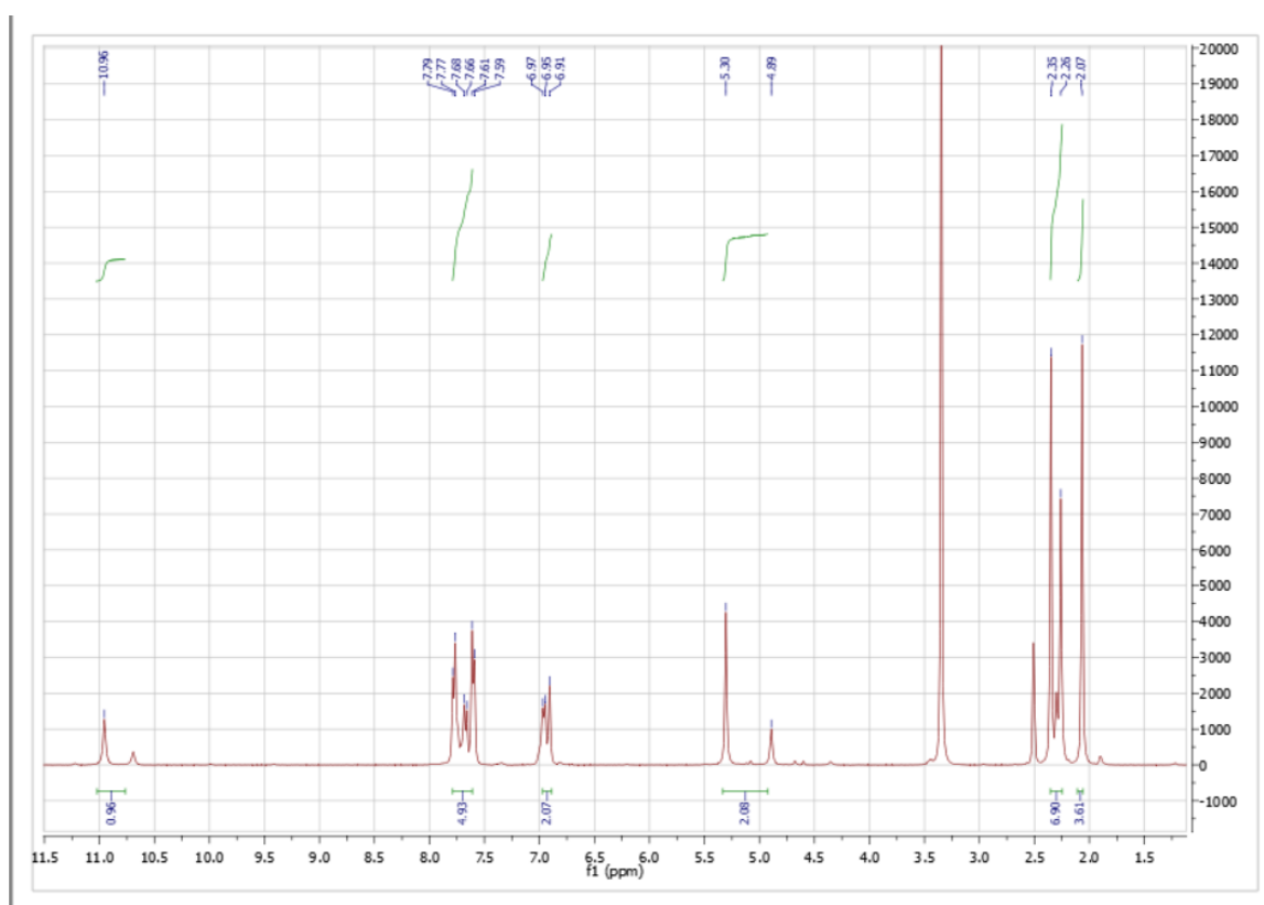
N'-(1-(4-bromophenyl)ethylidene)-2-((3,4-dimethyl-2-oxo-2H-chromen-7-yl)oxy)acetohydrazide
