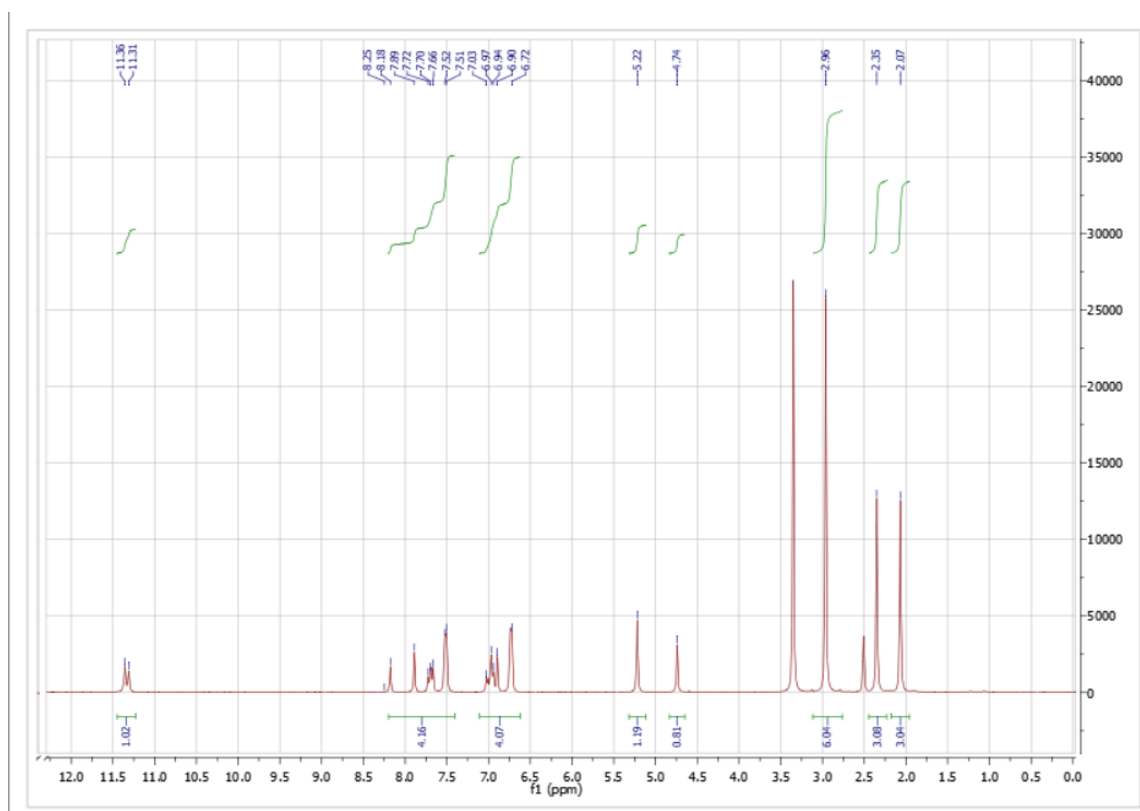
2-((3,4-dimethyl-2-oxo-2H-chromen-7-yl)oxy)-N'-(4-(dimethylamino)benzylidene)acetohydrazide
