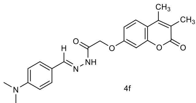
2-((3,4-dimethyl-2-oxo-2H-chromen-7-yl)oxy)-N'-(4-(dimethylamino)benzylidene)acetohydrazide
