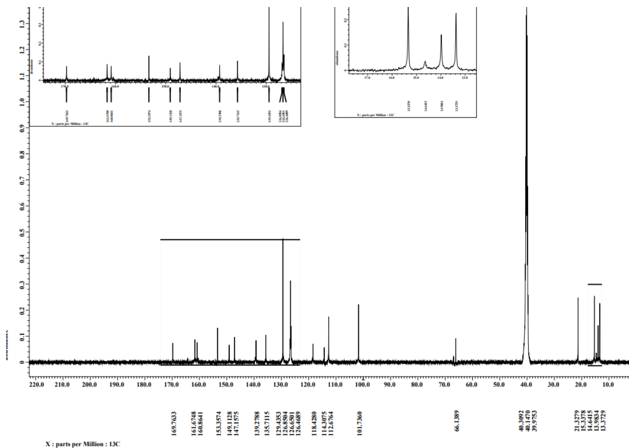
2-((3,4-dimethyl-2-oxo-2H-chromen-7-yl)oxy)-N'-(1-(p-tolyl)ethylidene)acetohydrazide
