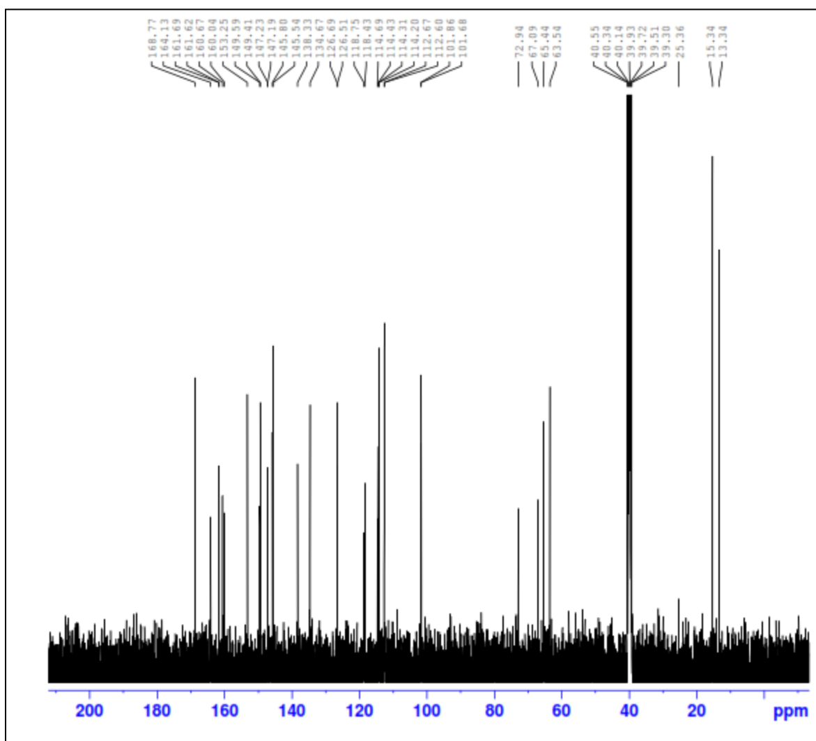
2-((3,4-dimethyl-2-oxo-2H-chromen-7-yl)oxy)-N'-(furan-2-ylmethylene)acetohydrazide
