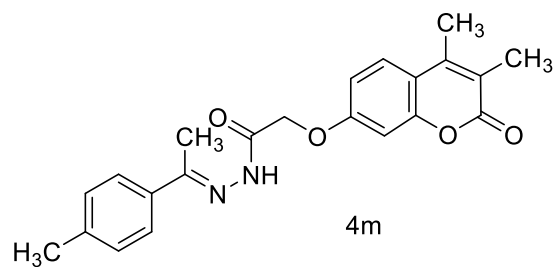
2-((3,4-dimethyl-2-oxo-2H-chromen-7-yl)oxy)-N'-(1-(p-tolyl)ethylidene)acetohydrazide
