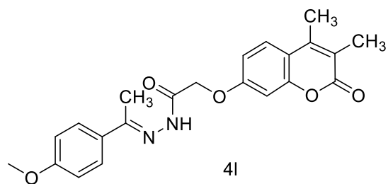
2-((3,4-dimethyl-2-oxo-2H-chromen-7-yl)oxy)-N'-(1-(4-methoxyphenyl)ethylidene)acetohydrazide
