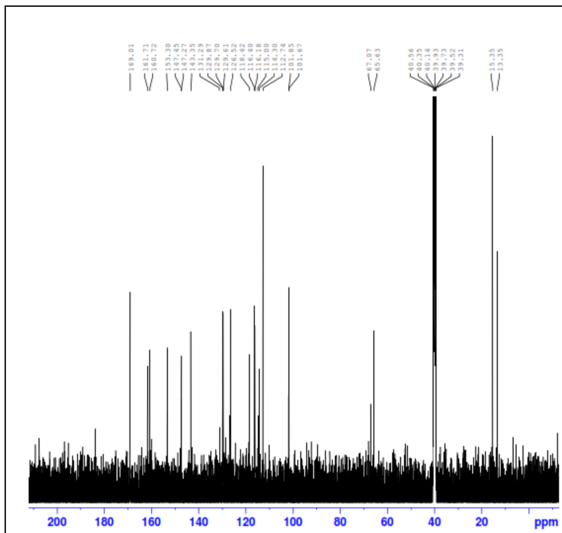
2-((3,4-dimethyl-2-oxo-2H-chromen-7-yl)oxy)-N'-(4-fluorobenzylidene)acetohydrazide
