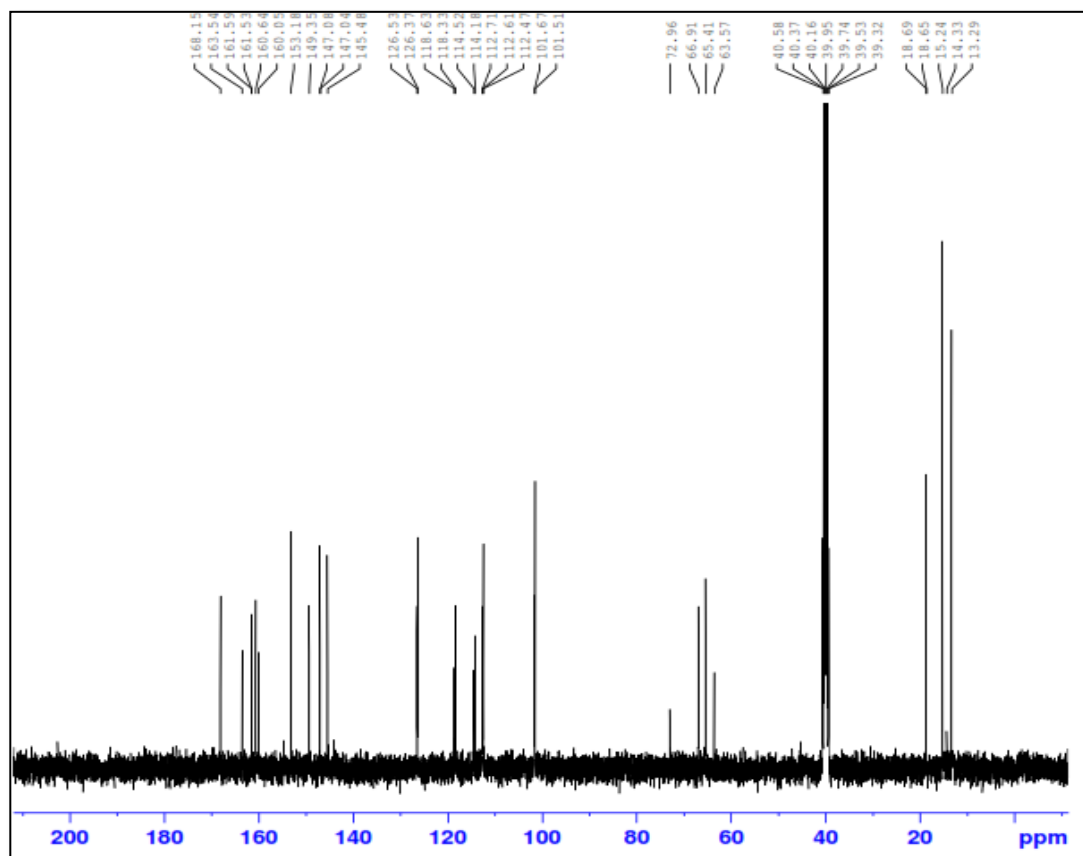
2-((3,4-dimethyl-2-oxo-2H-chromen-7-yl)oxy)-N'-ethylideneacetohydrazide
