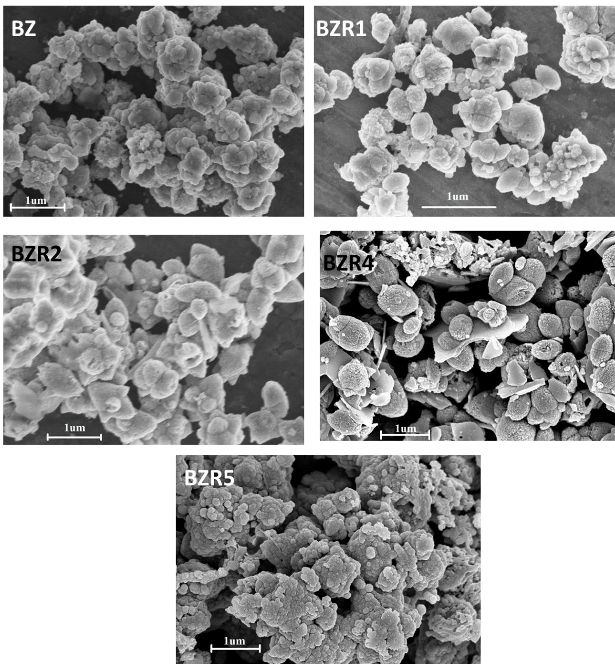
ESI-Fig. S1: FESEM images of BZ, BZR1, BZR2, BZR3, BZR4 and BZR5
