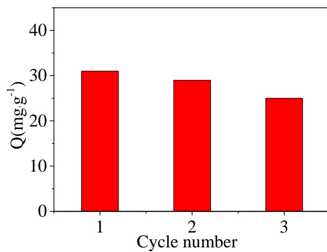
Fig. S2. Reusability of PA-HPEI-OACF.
