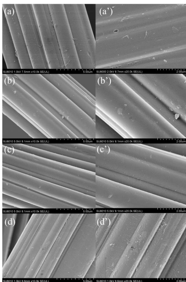
Fig. S1. SEM images of adsorbents (a, a': ACF; b, b': OACF; c, c': HPEI-OACF; d, d': PA-HPEI-OACF).
