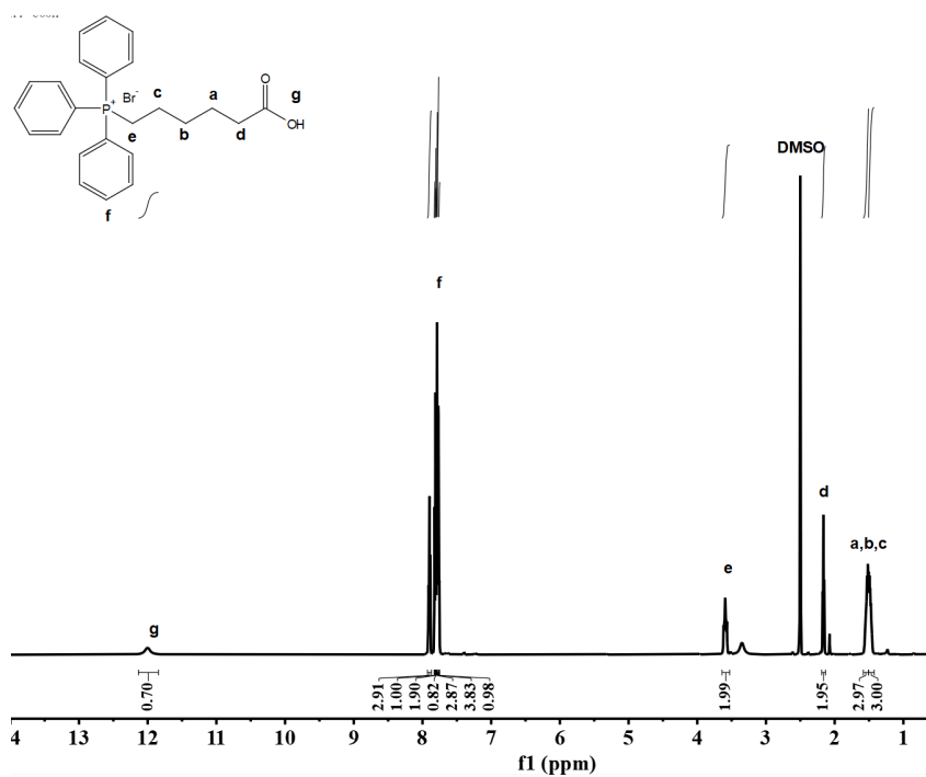
Fig. S1 1 H NMR spectrum of TPP-COOH.
