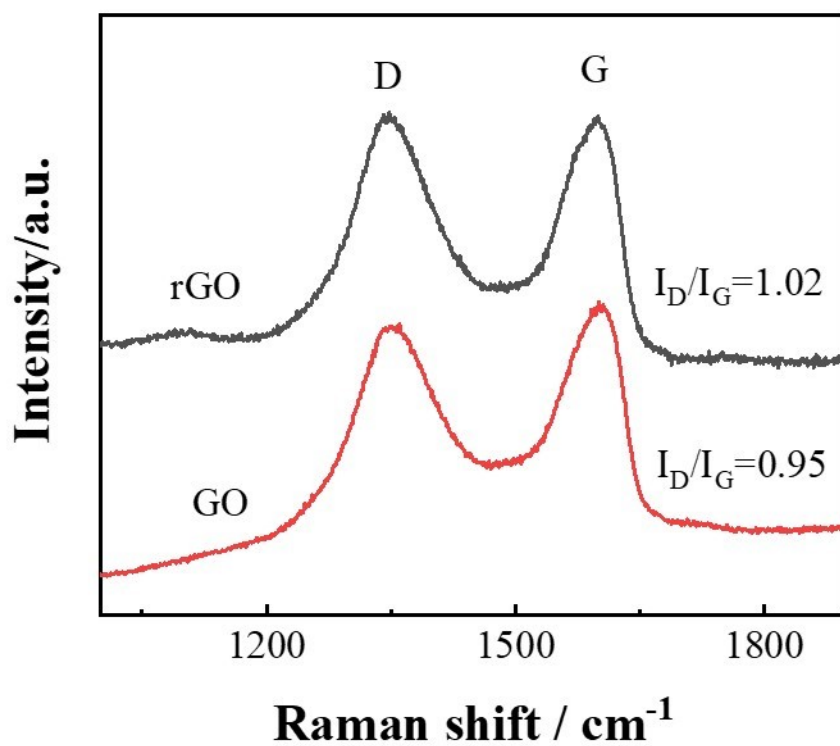
Fig. S2. Raman spectra of GO and rGO.
