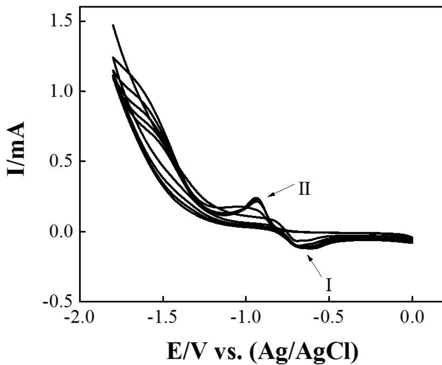
Fig. S1. CVs for the electrochemical reduction of FTO in 10 mM of PBS solution (pH 7.0)
