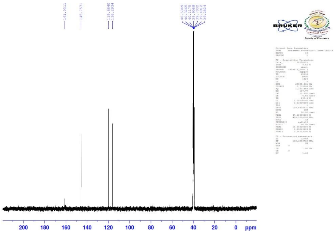
Fig. S4. 13 C NMR spectra of Triazinone (9) Product in DMSO.
