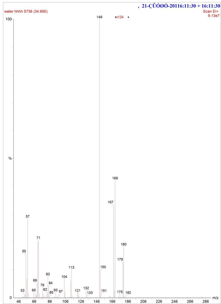
Fig. S5. GC/MS spectra of Triazinone (9) Product.
