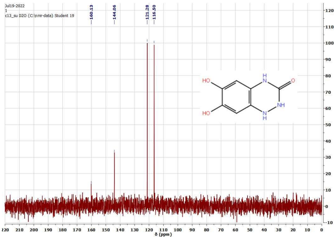
Fig. S2. ^{13}\text{C} NMR spectra of Triazinone (9) Product in \text{D}_2\text{O} .
