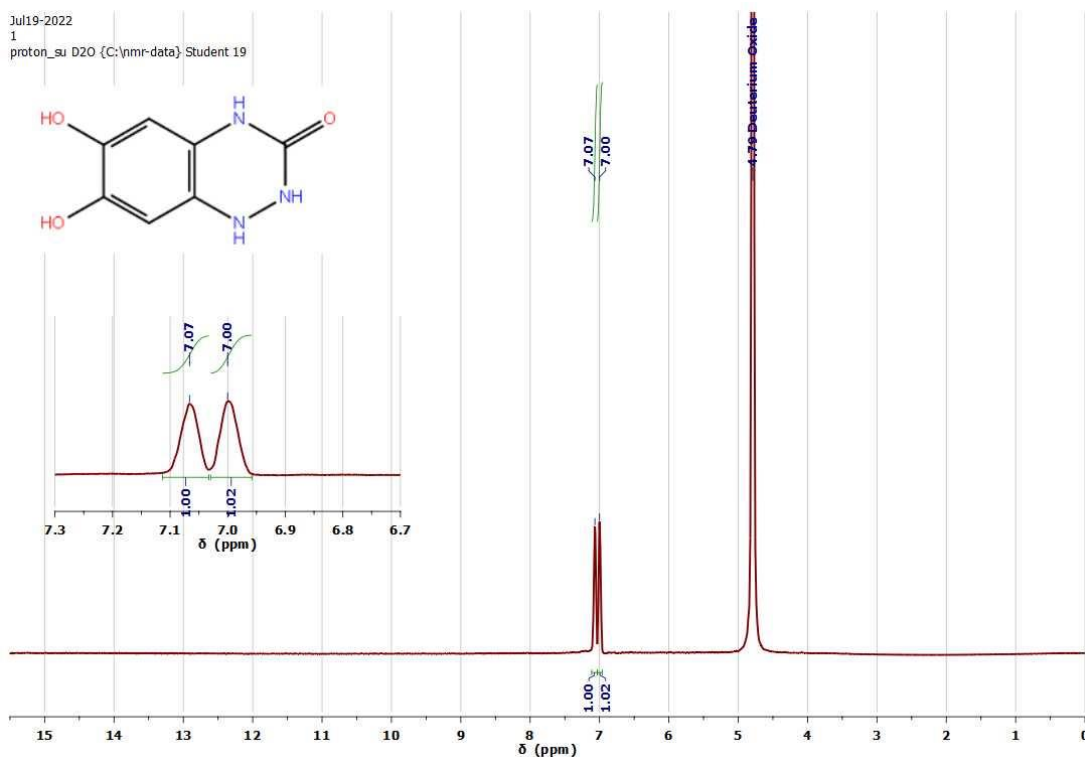
Fig. S1. 1 H NMR spectra of Triazinone (9) Product in D 2 O.
