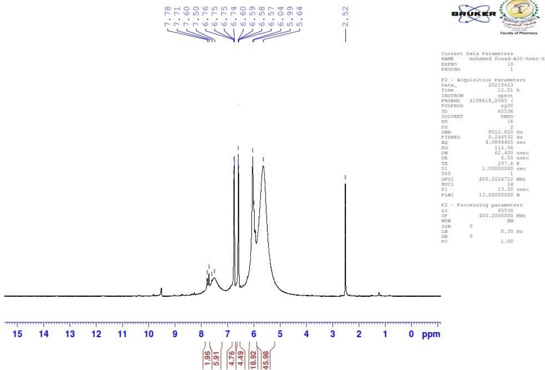
Fig. S3. 1 H NMR spectra of Triazinone (9) Product in DMSO.
