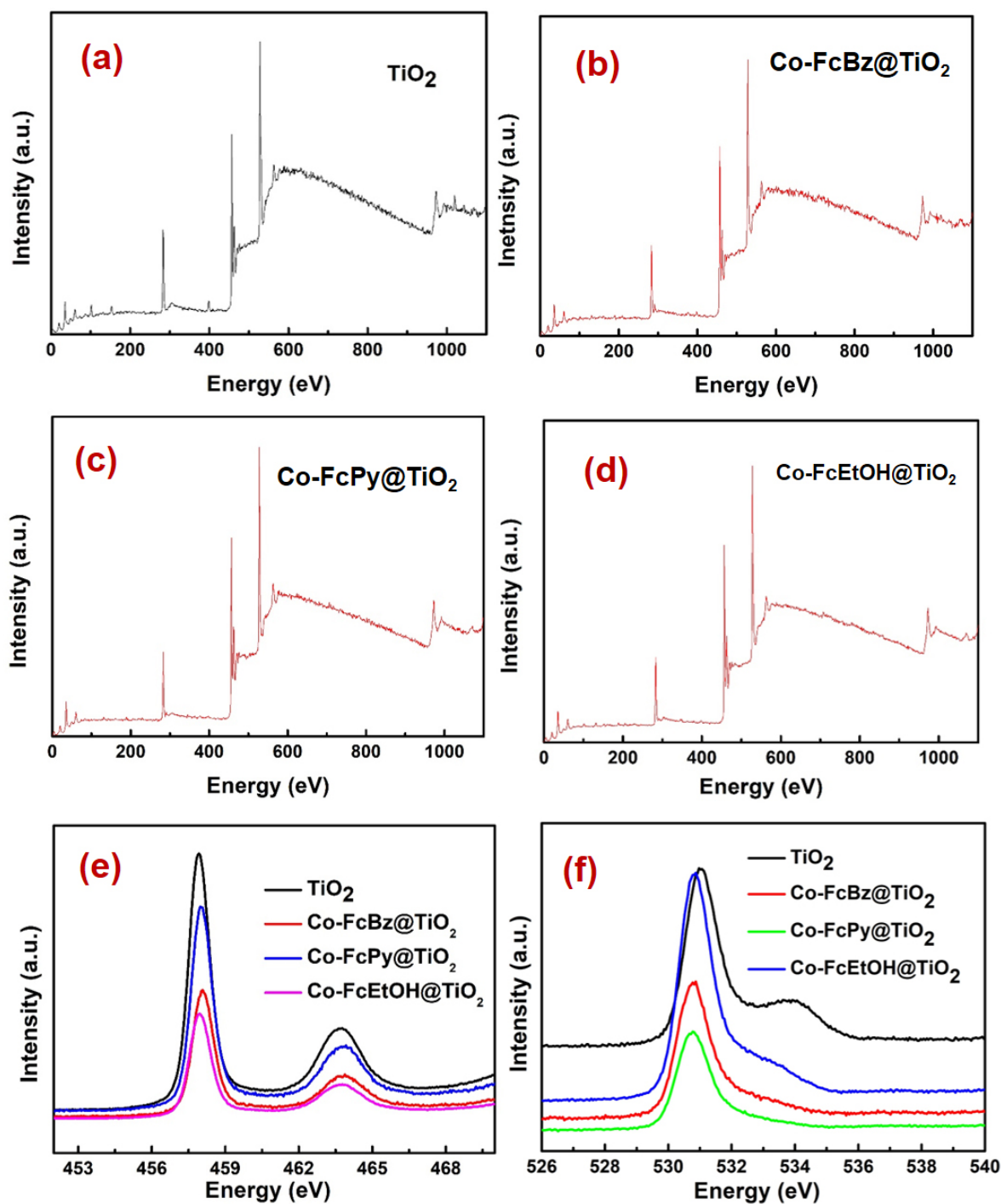
Fig. S2 (a)-(d) Complete XPS profiles for \text{TiO}_2 and sensitizers adsorbed over \text{TiO}_2 ; (e) XPS for \text{Ti}2p for \text{TiO}_2 and sensitizers adsorbed over \text{TiO}_2 ; (f) XPS for \text{O}2p for \text{TiO}_2 and sensitizers adsorbed over \text{TiO}_2 .
