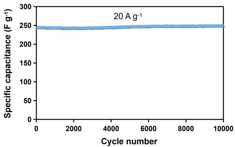
Fig. S2 Cycling stability of PUHPC-700 at 20 A g -1
