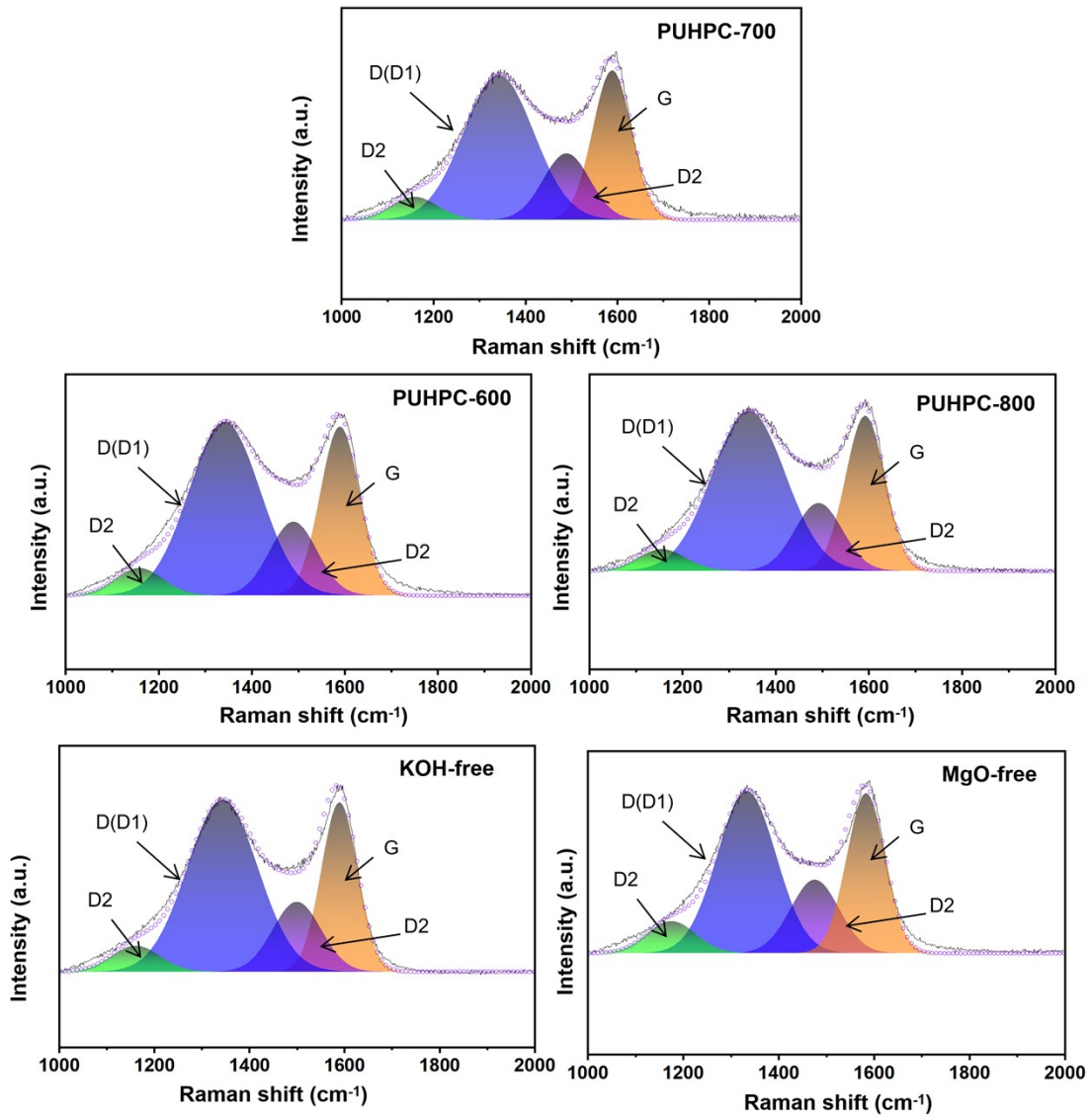
Fig. S1 The Raman fitting result of sample
