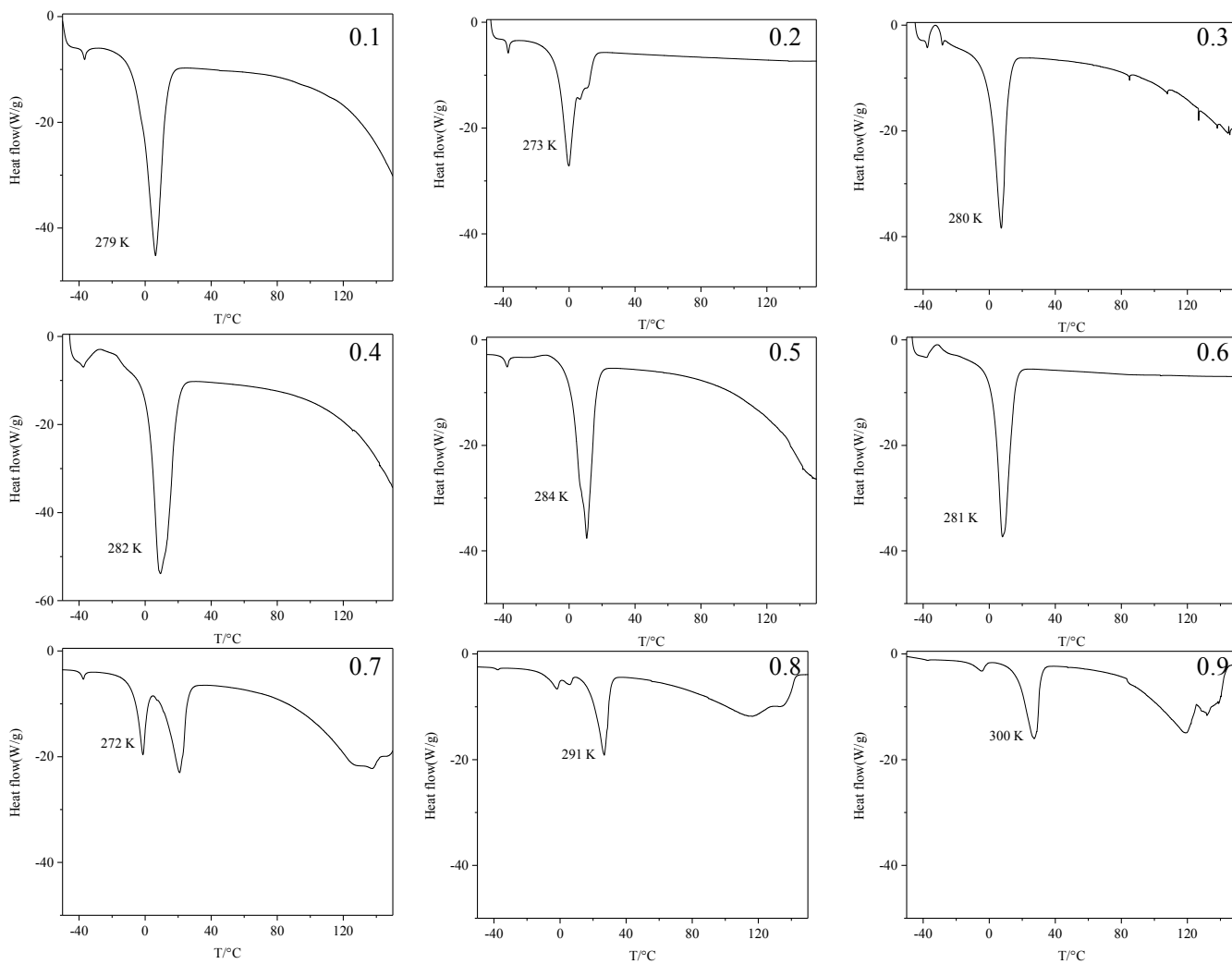
Figure S1. DSC curves of 3-bromobenzonitrile-levulinic acid system with different levulinic acid mole fractions.
