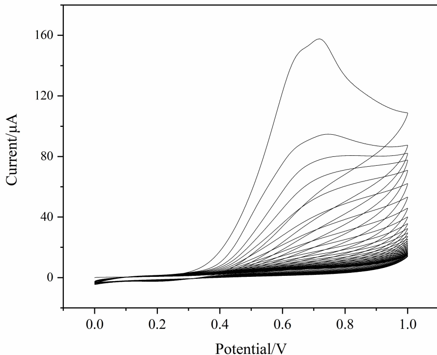
Fig. S1. Cyclic voltammogram curve of electropolymerization.
