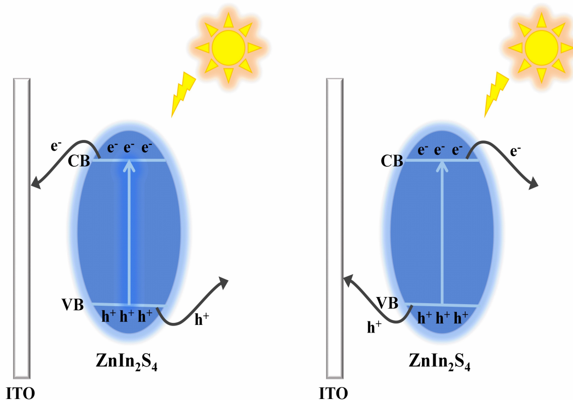
Fig. S3. The possible electron-transfer mechanism of \text{ZnIn}_2\text{S}_4 at 0.2 V and -0.3 V.
