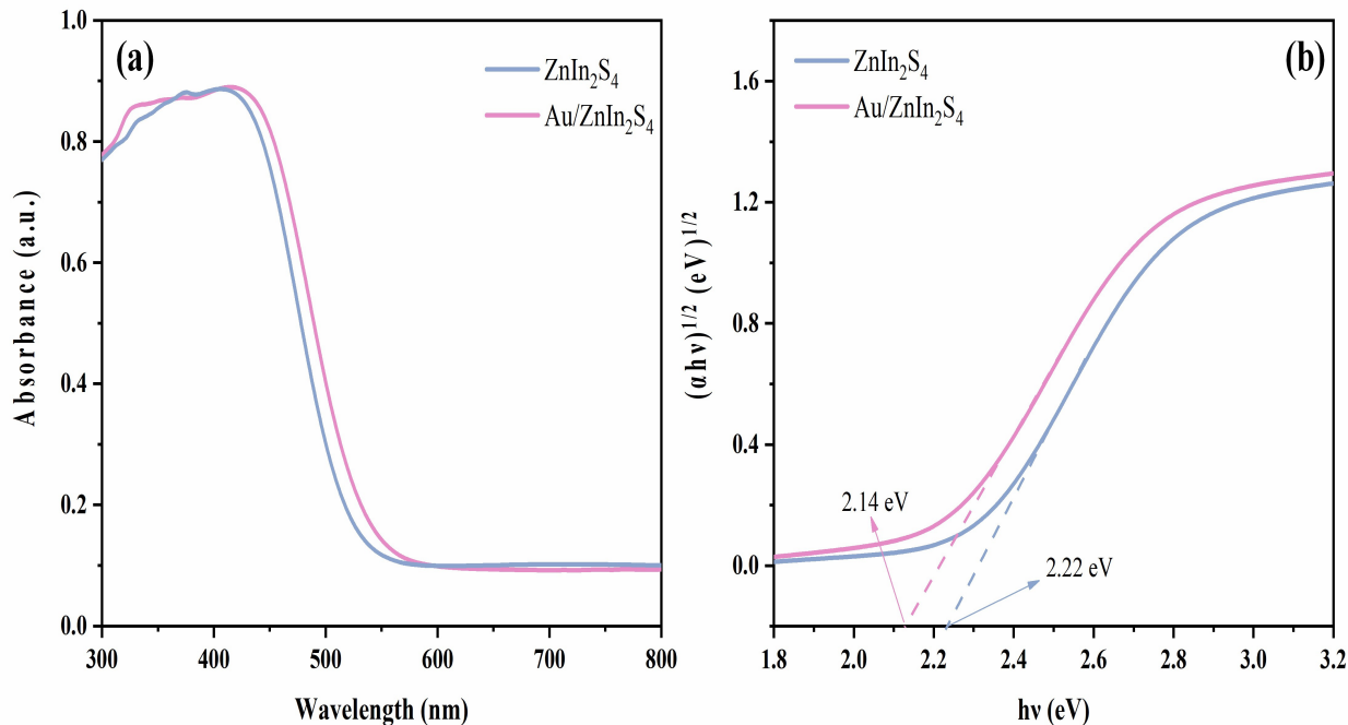
Fig. S4. UV-vis diffuse reflectance spectra (a) of ZnIn 2 S 4 and Au/ ZnIn 2 S 4 ; the band-gap energies (b) of ZnIn 2 S 4 and Au/ ZnIn 2 S 4 samples.
