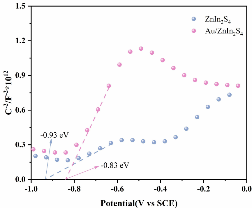
Fig. S5. M-S plots of ZnIn_2S_4 and Au/ZnIn_2S_4 samples.
