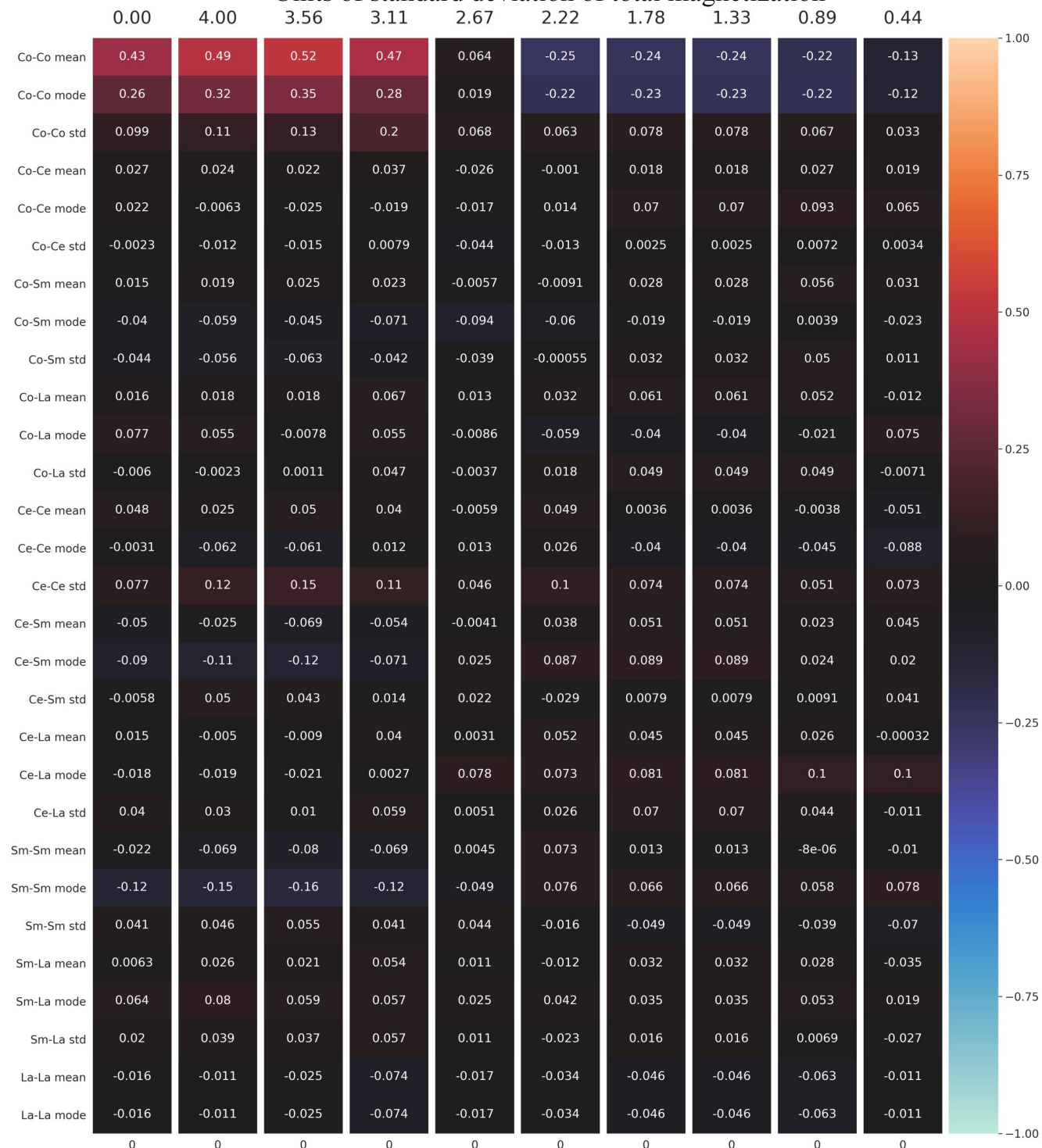
Units of standard deviation of total magnetization
