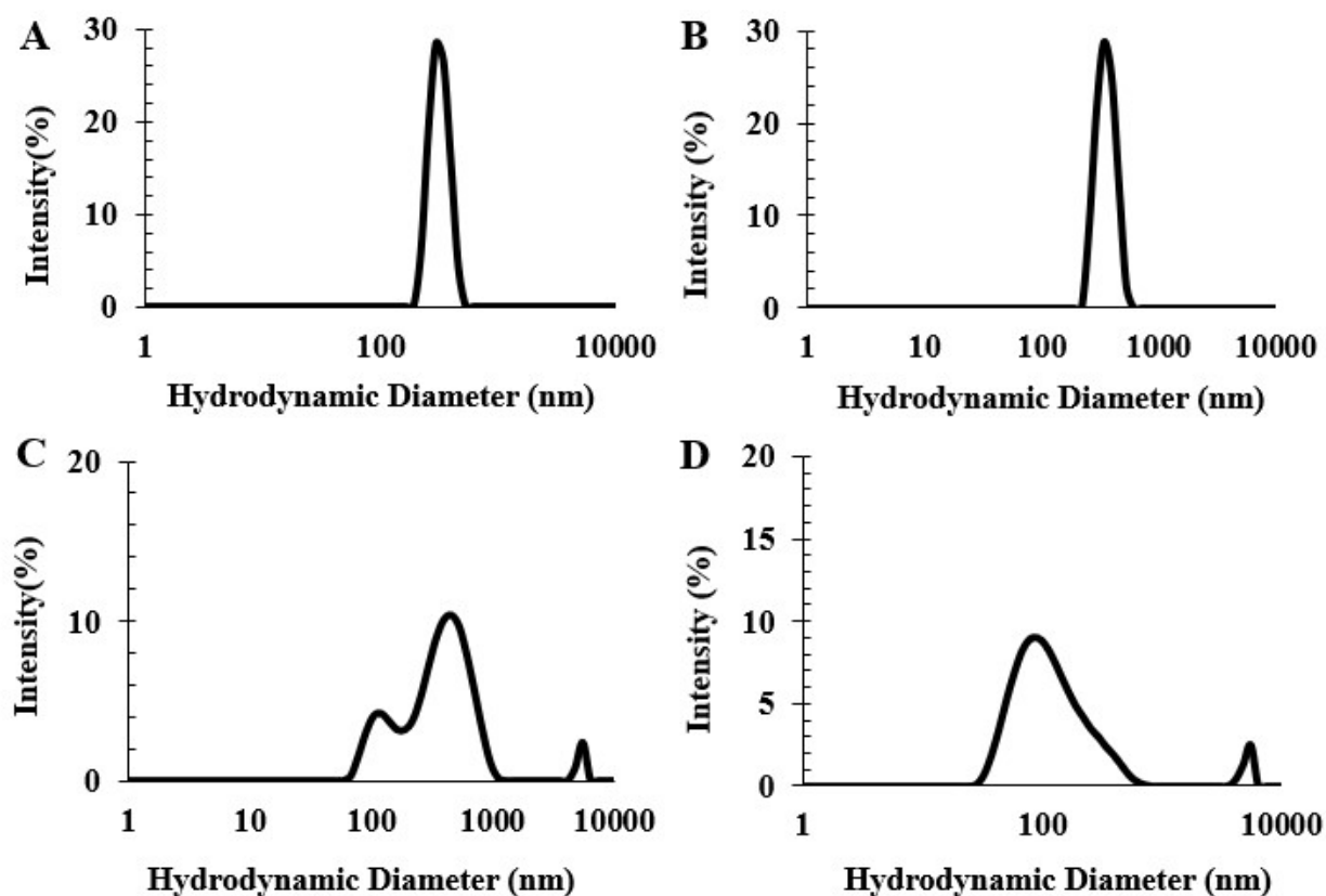
Figure S1. Representative stability curves (from n=3) show that IL-LDBC's have a shelf-life in solution up to 3 weeks. Dynamic Light Scattering (DLS) hydrodynamic diameter measurements of A) IL-LDBC's during the first week of synthesis, B.) 2 weeks after synthesis, C.) 3 weeks after synthesis, and D.) 4 weeks after synthesis.
