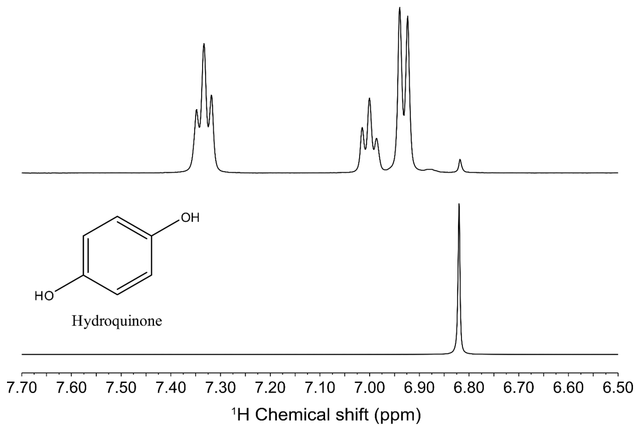
Figure S2: Comparison of chemical shift of Phenol + P25 after 24hrs illumination and hydroquinone standard (Alfa Aesar #L02558 ).
