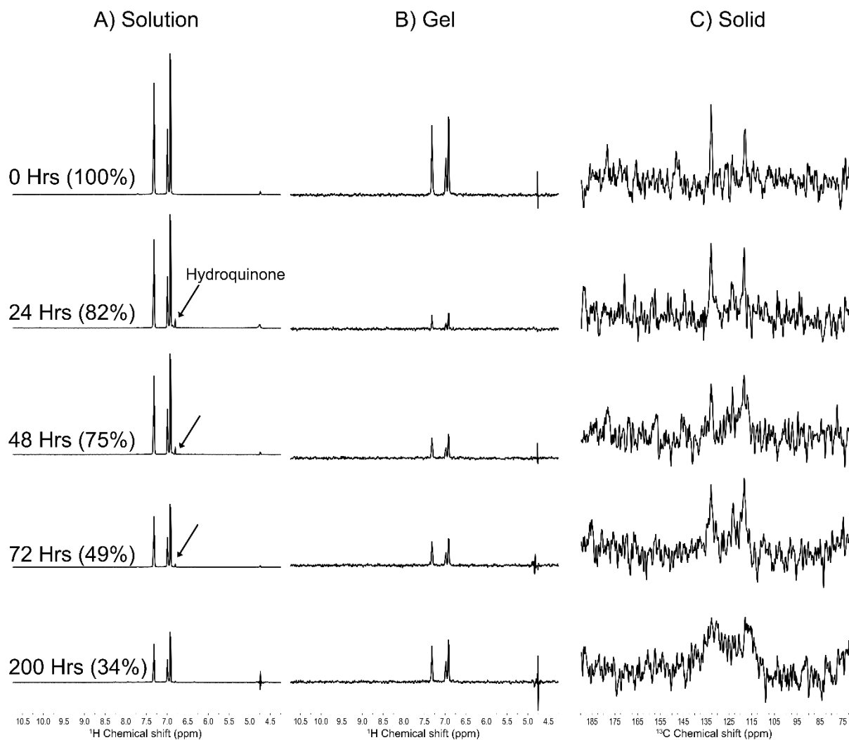
Figure S1: Extended NMR spectrum of figure 3 showing full aromatic region.
