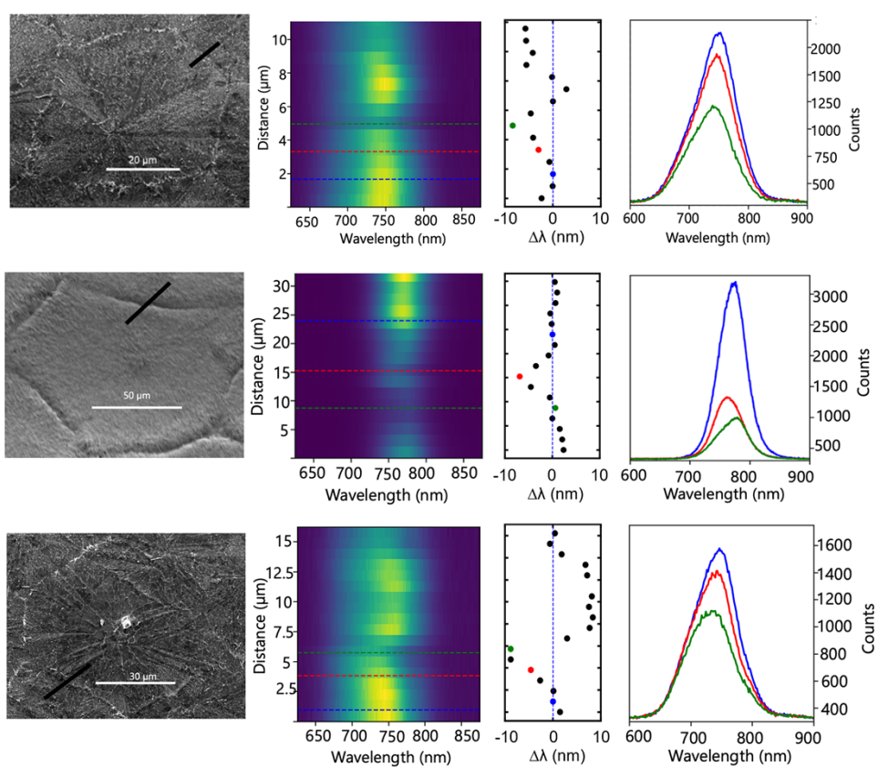
Figure S1. Scanning electron microscope images (left column) with corresponding CL spectra as function of the linescan (black) for three different hybrid perovskite samples fabricated at three different times. Spectral shifts (nm) with respect to the grain centre (blue point). Representative spectra from grain centre (blue), edge (red), and boundary (green).
