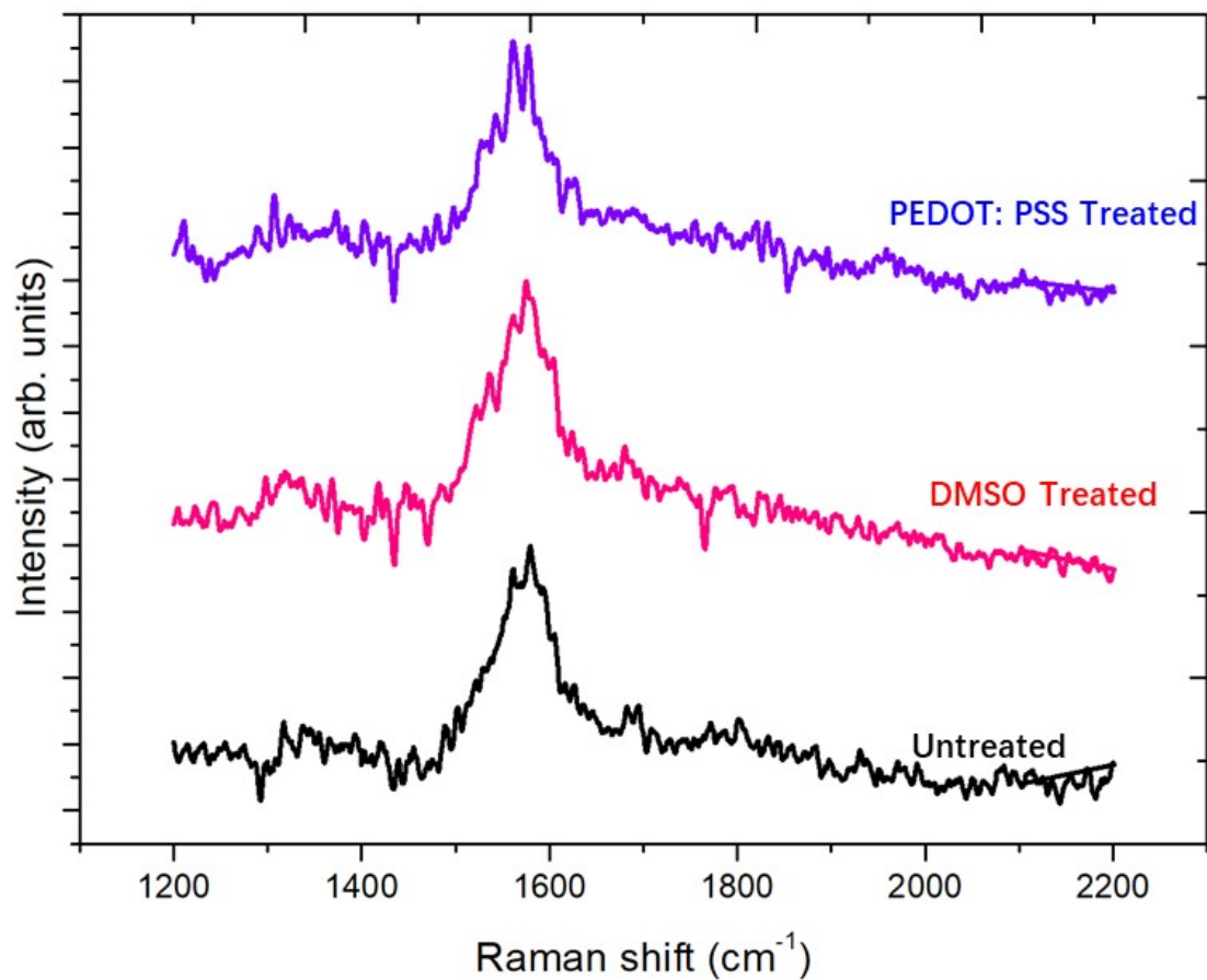
Figure S3. Visible Raman spectra of untreated CNT emitter (black), DMSO treated CNT emitter (red) and PEDOT: PSS treated CNT (blue)
