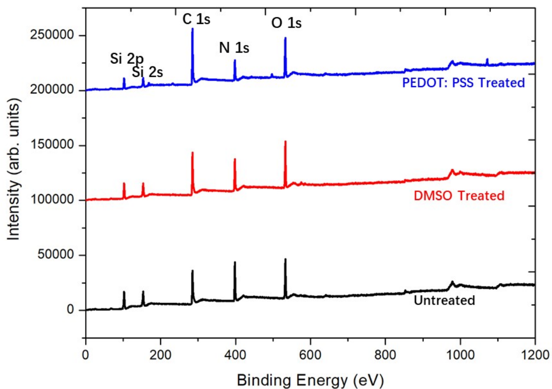
Figure S2. XPS spectra of untreated CNT emitter (black), DMSO treated CNT emitter (red) and PEDOT: PSS treated CNT (blue)
