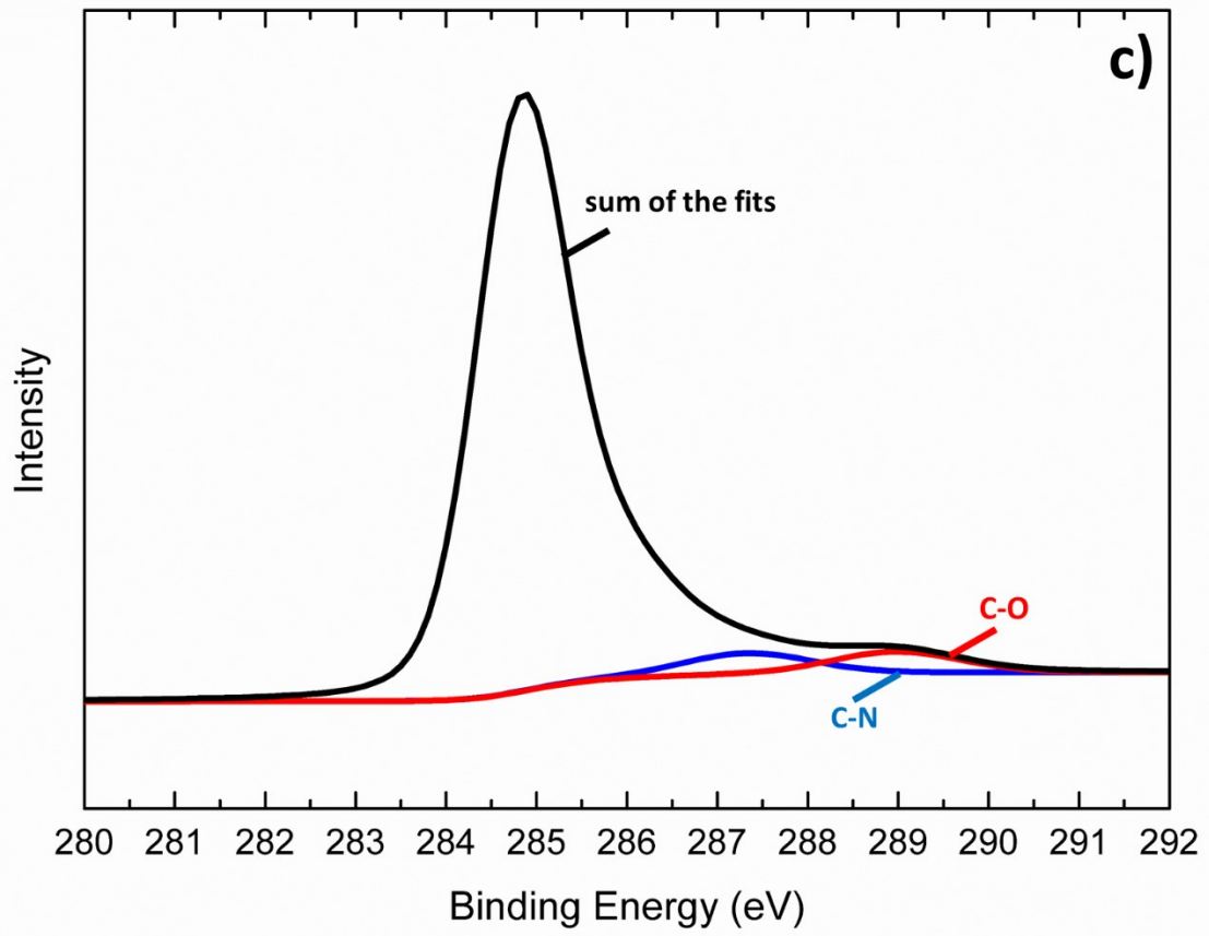
Figure S1. the C 1s XPS spectra of CNT emitters. a) without treatment, b) with DMSO treatment, c) with PEDOT: PSS treatment.
