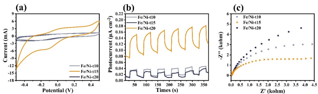
Figure 5s. (a) CV curves, (b) photocurrent response, (c) Nyquist plots of different photocatalyst samples of Fe/Ni-t10、Fe/Ni-t15(Fe/Ni-T120) and Fe/Ni-t20.
