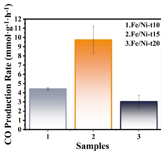
Figure 4s. CO production rate of Fe/Ni-t10、Fe/Ni-t15(Fe/Ni-T120) and Fe/Ni-t20.
