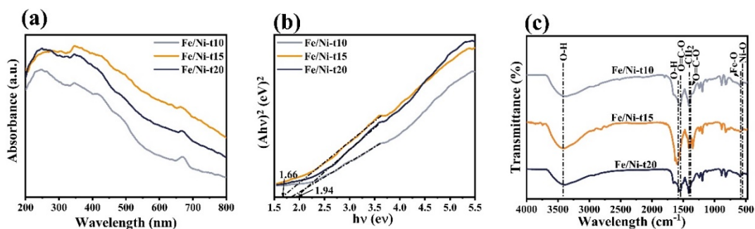
Figure 3s. (a) UV-vis DRS spectra, (b) Tauc plots, (c) FT-IR spectra of Fe/Ni-t10, Fe/Ni-t15(Fe/Ni-T120) and Fe/Ni-t20.
