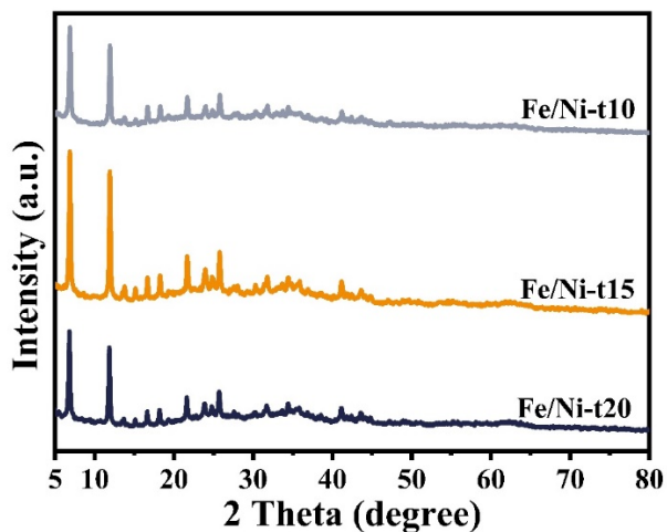
Figure 1s. XRD of Fe/Ni-t10, Fe/Ni-t15(Fe/Ni-T120), Fe/Ni-t20.
