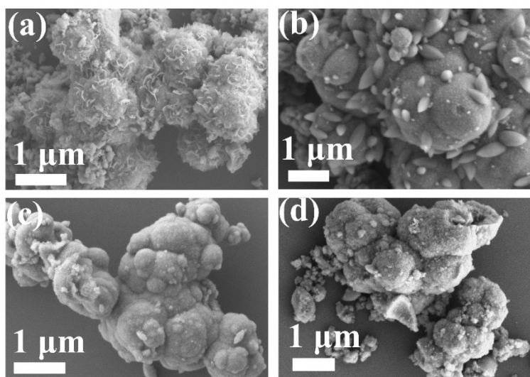
Figure 2s.(a) SEM images of Fe/Ni-t10, (b) Fe/Ni-t15(Fe/Ni-T120), (c)Fe/Ni-t20, (d) Photocatalytic Fe/Ni- t15(Fe/Ni-T120).
