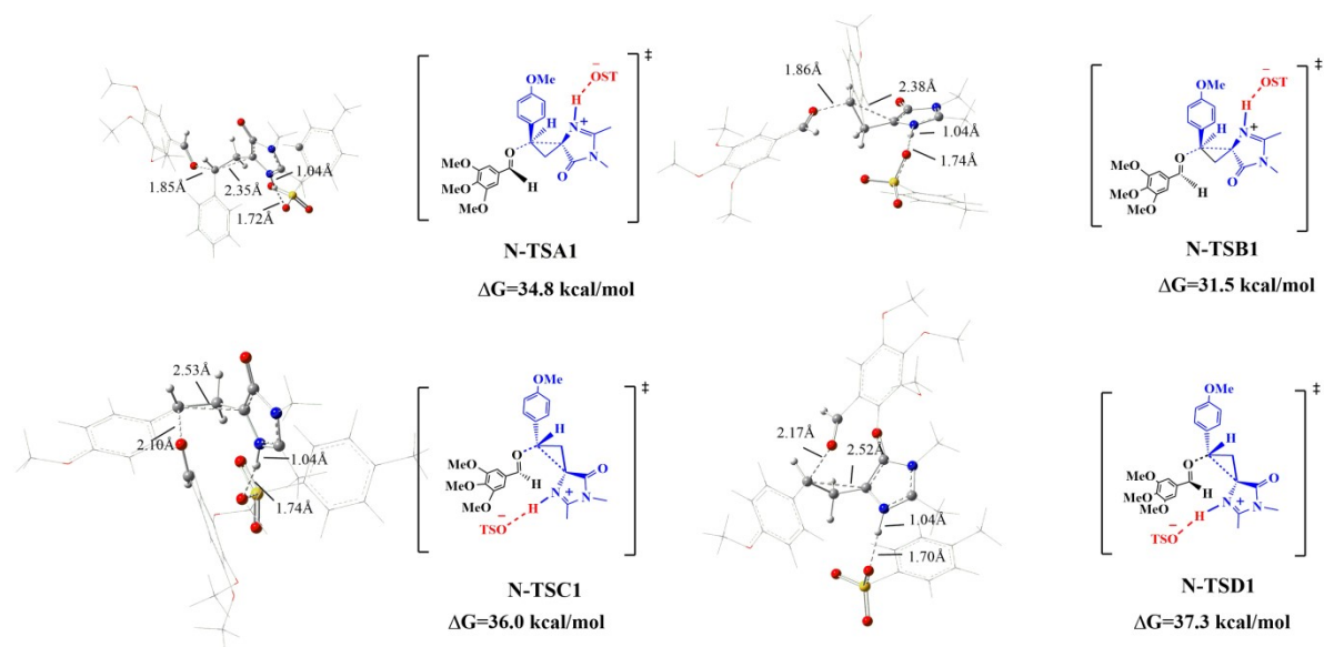
Figure S1. Optimized structures and Gibbs free energy barriers of the transition states of the rate-determining steps of paths A, B, C and D in reaction between aldehyde 2a and ion-pair complex 1a-TsOH-N (in dichloromethane, 273.15 K, energies are given in kcal/mol).
