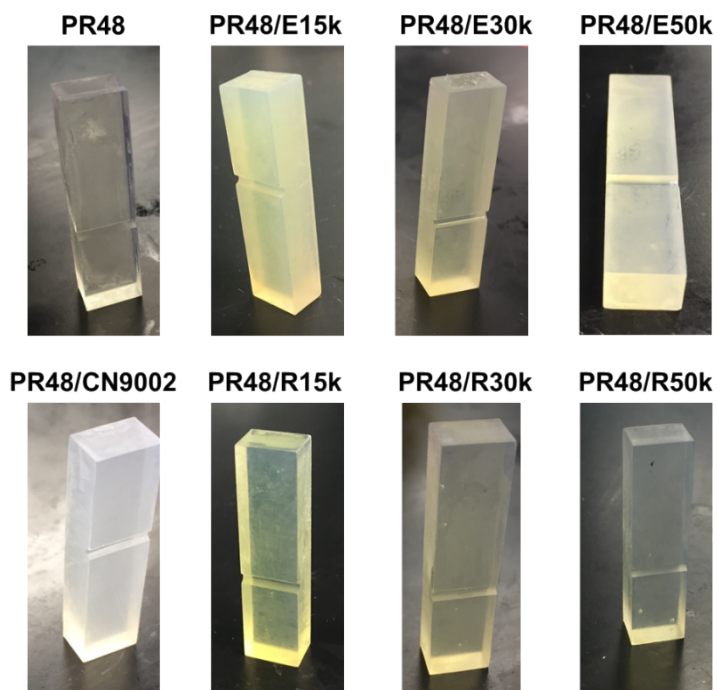
Figure S1. Photographs of 3D printed object after UV post-curing.
