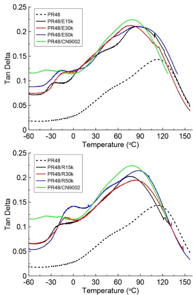
Figure S2. Tan( \delta ) profiles as a function of temperature for PR48 systems modified with a) end-functionalized and b) random-functionalized oligomers. The system modified with CN9002 system is also included. Samples are photopolymerized at 20 mW/cm 2 for 10 min using 0.5 wt % TPO.
