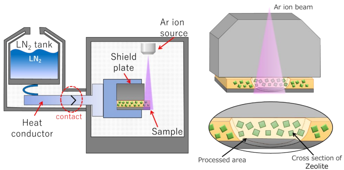
Figure S2. Schematic presentation for preparation of samples technology.
