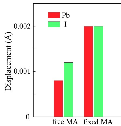
Figure S1. The simulated root-mean-square displacements of Pb and I atoms in the MAPbI 3 perovskite with free and fixed MA cations.
