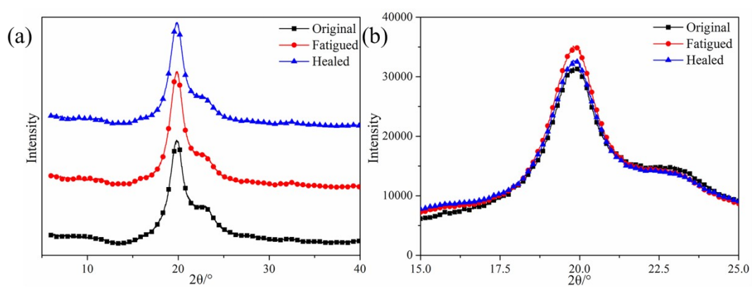
Figure S3 (a) and (b) XRD patterns of original, fatigued and healed PH2T1F
