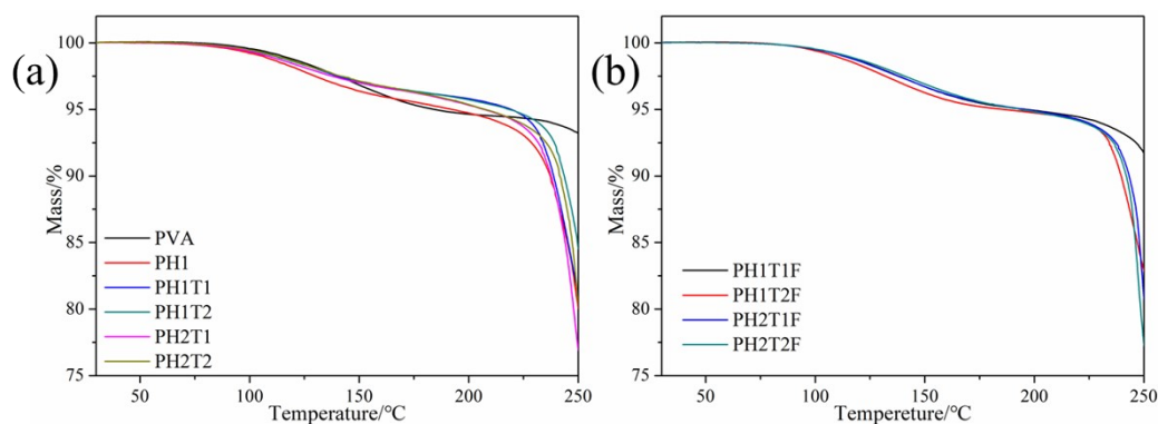
Figure S1 TGA curves PVA and PVA based SMPs
