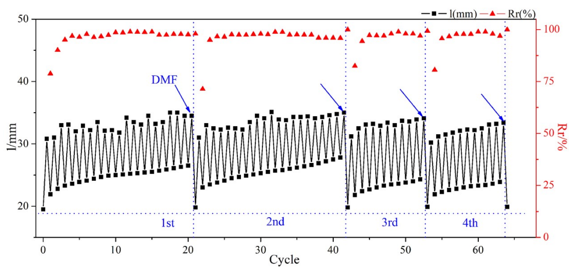
Figure S4 Fatigue-healing behavior of cross-linked EVOH
