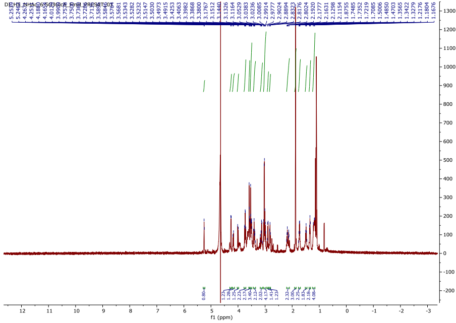
gHSQC ( \text{D}_2\text{O} , 500 MHz) of 5
