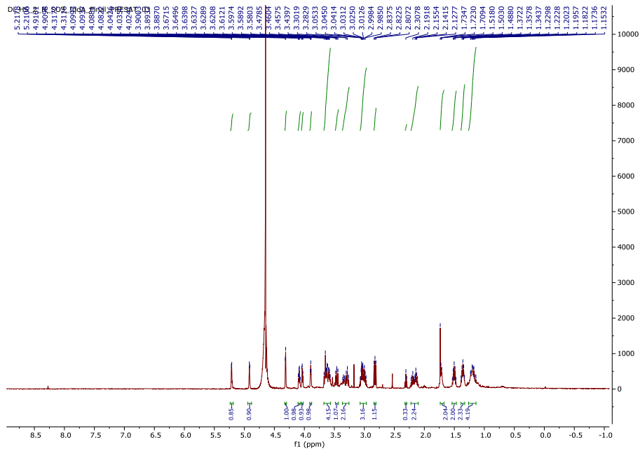
^1\text{H-NMR} ( \text{D}_2\text{O} , 500 MHz) of 12
