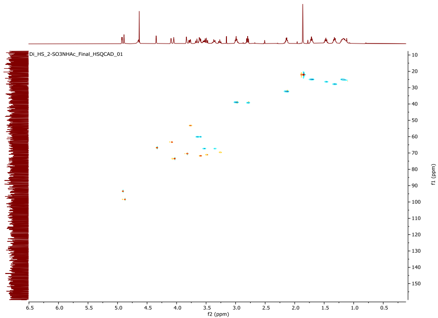
gHSQC (D 2 O, 500 MHz) of 11
