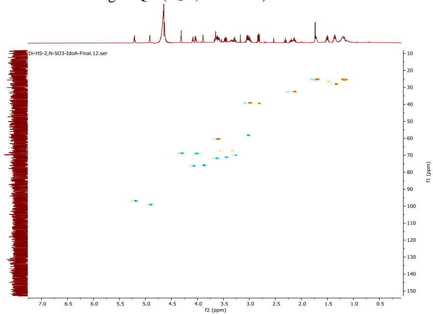
gHSQC ( \text{D}_2\text{O} , 500 MHz) of 12
