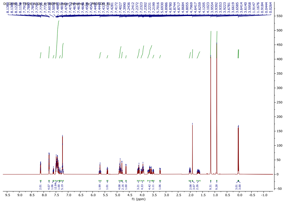
13 C-NMR (CDCl 3 , 126 MHz) of 25
