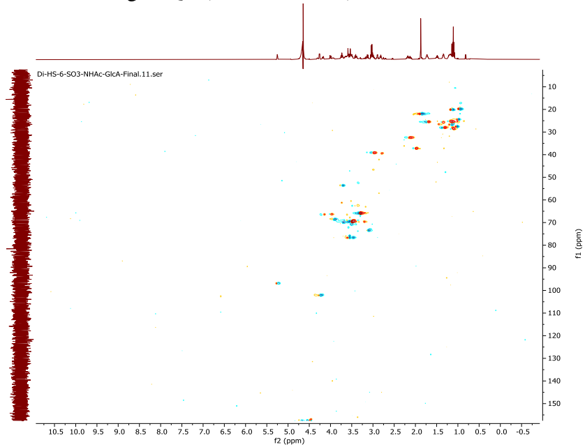
gHSQC ( \text{D}_2\text{O} , 500 MHz) of 5
