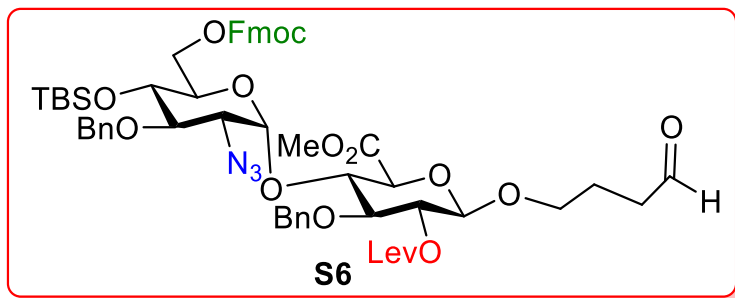
1 H-NMR (CDCl 3 , 500 MHz) of S6
