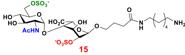
1 H-NMR (D 2 O, 500 MHz) of 15
