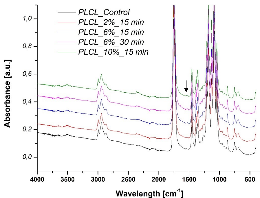
Figure S1. ATR-FTIR spectra of PLCL_Control and chosen PLCL samples after aminolysis with marked amide II peak.
