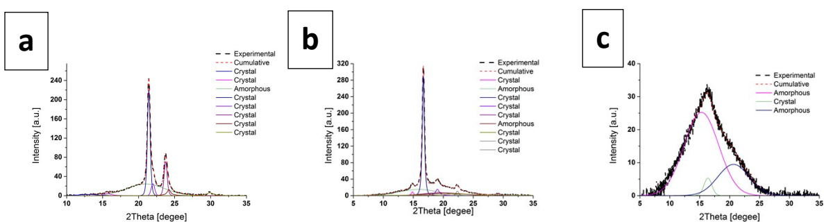
Figure S2. WAXS scattering profiles of: a) PCL_Control, b) PLCL_Control and c) PLLA_Control with fitting.
