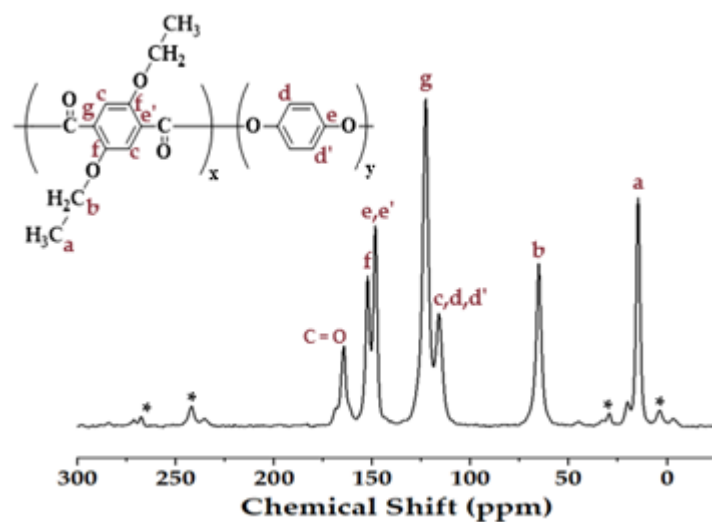
Supplement-Figure 3. ^{13}\text{C} -NMR chemical shifts of TLCP at room temperature. In the chemical formula, x:y=1:1 . The spinning sidebands are marked with asterisks.
