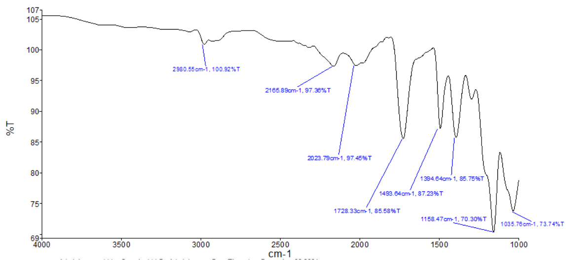
Supplement-Figure 1. FT-IR spectrum of TLCP at room temperature. In the chemical formula, x:y=1:1.
