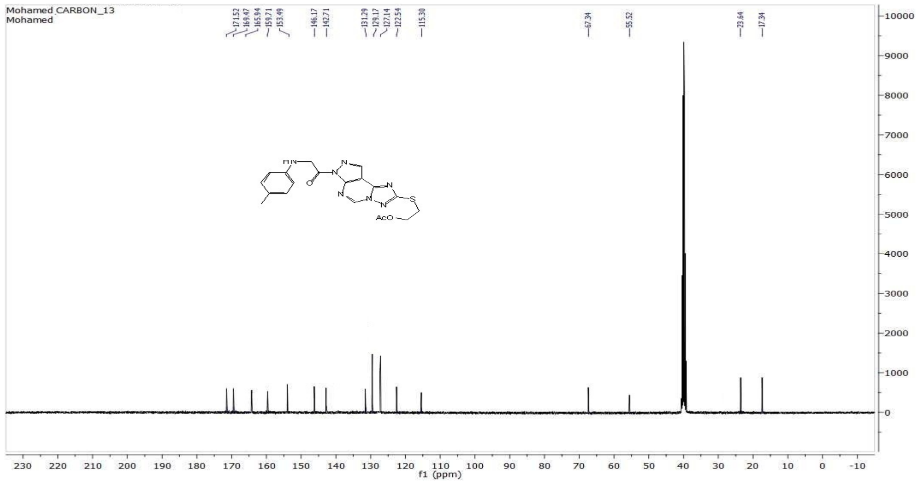
C 13 -NMR FOR COMP. 13
