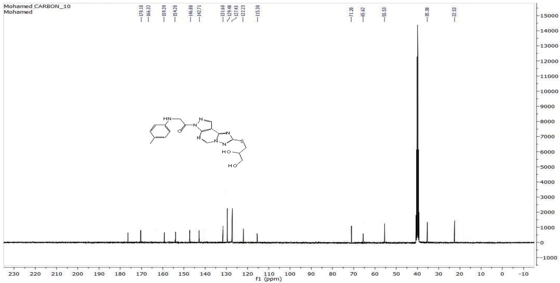
C^{13} -NMR FOR COMP. 10
