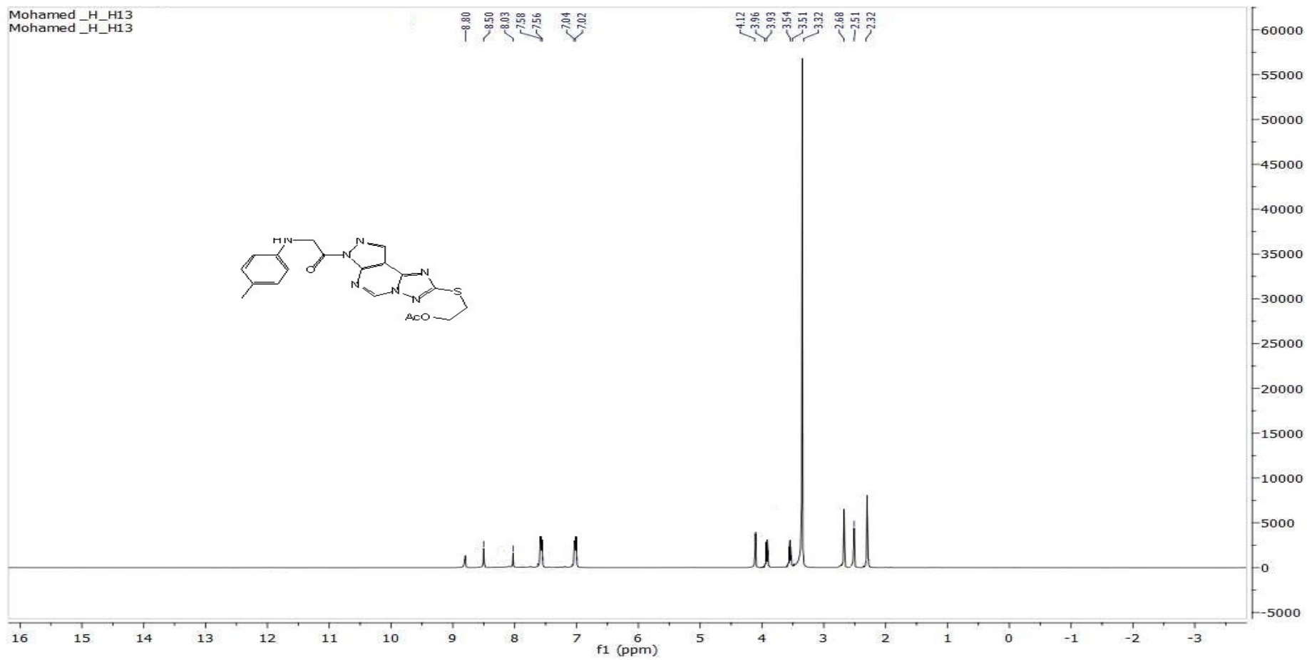
1 H-NMR FOR COMP. 13
