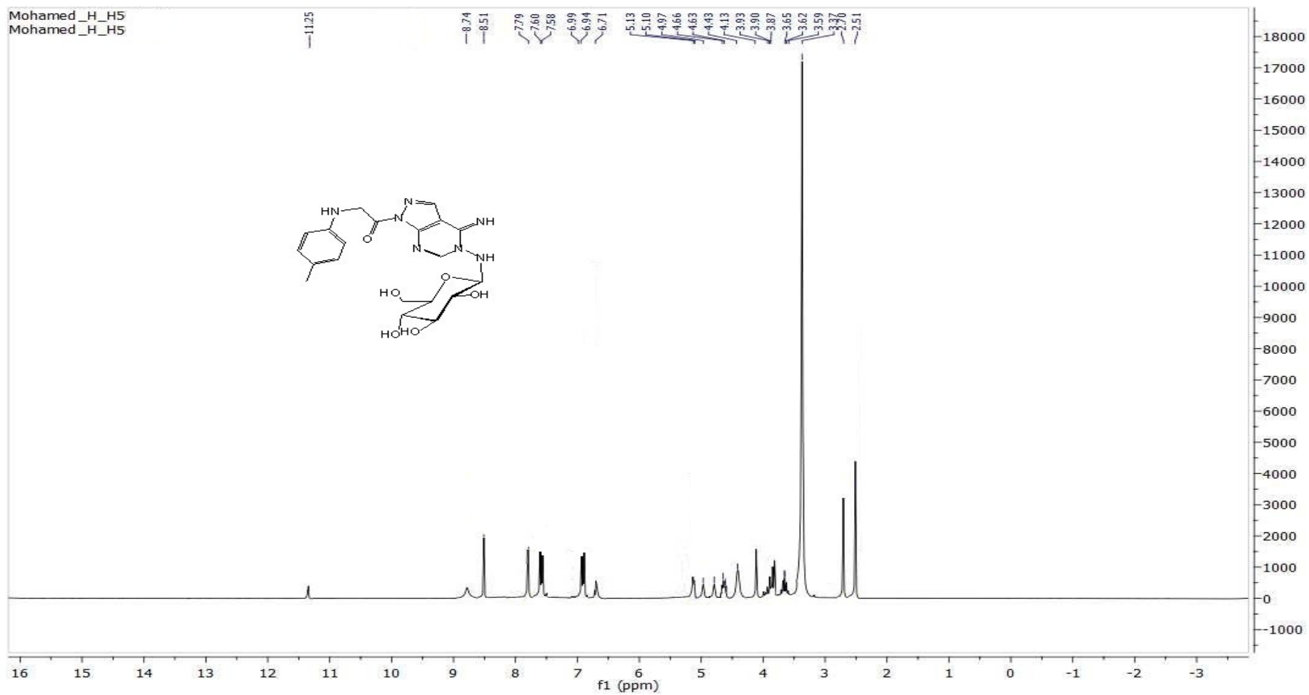
^1\text{H-NMR} FOR COMP. 5
