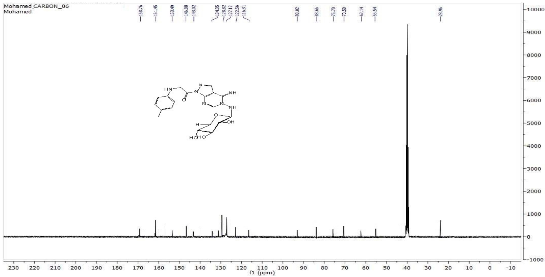
C^{13} -NMR FOR COMP. 6
