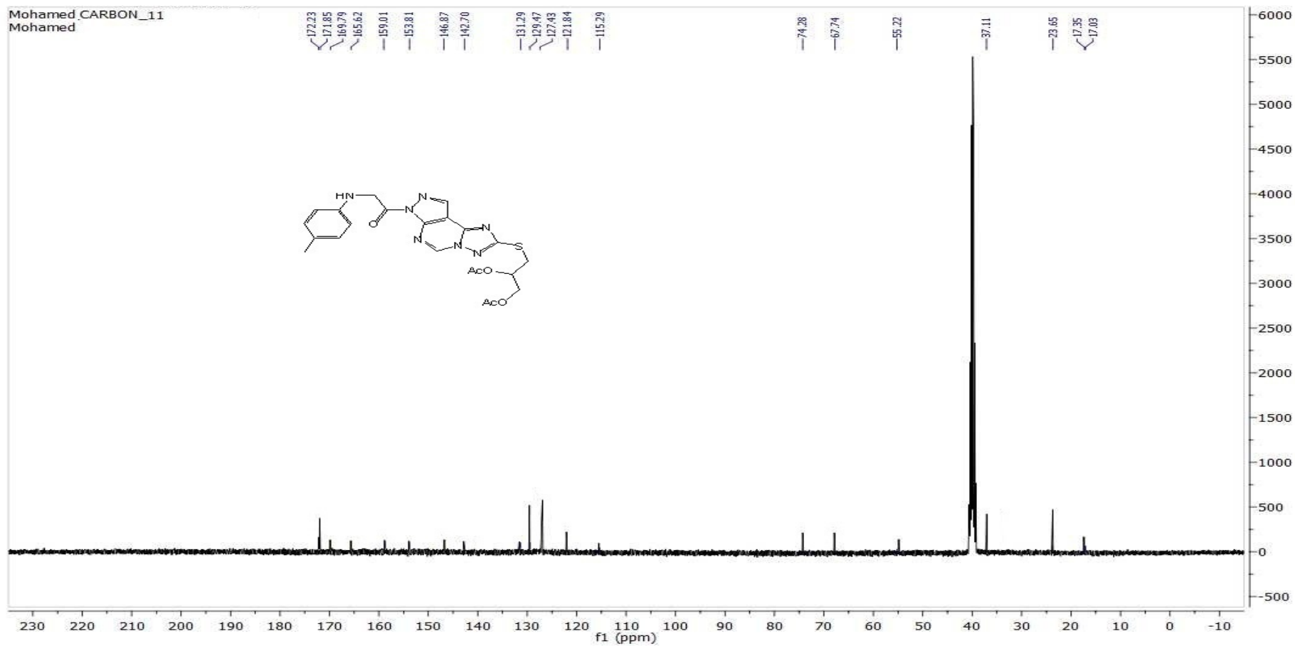
C 13 -NMR FOR COMP. 11
