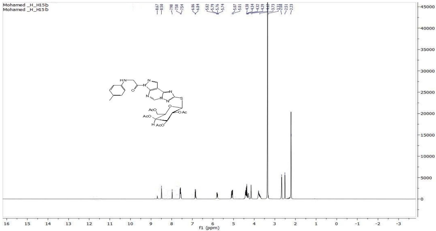
1 H-NMR FOR COMP. 15
