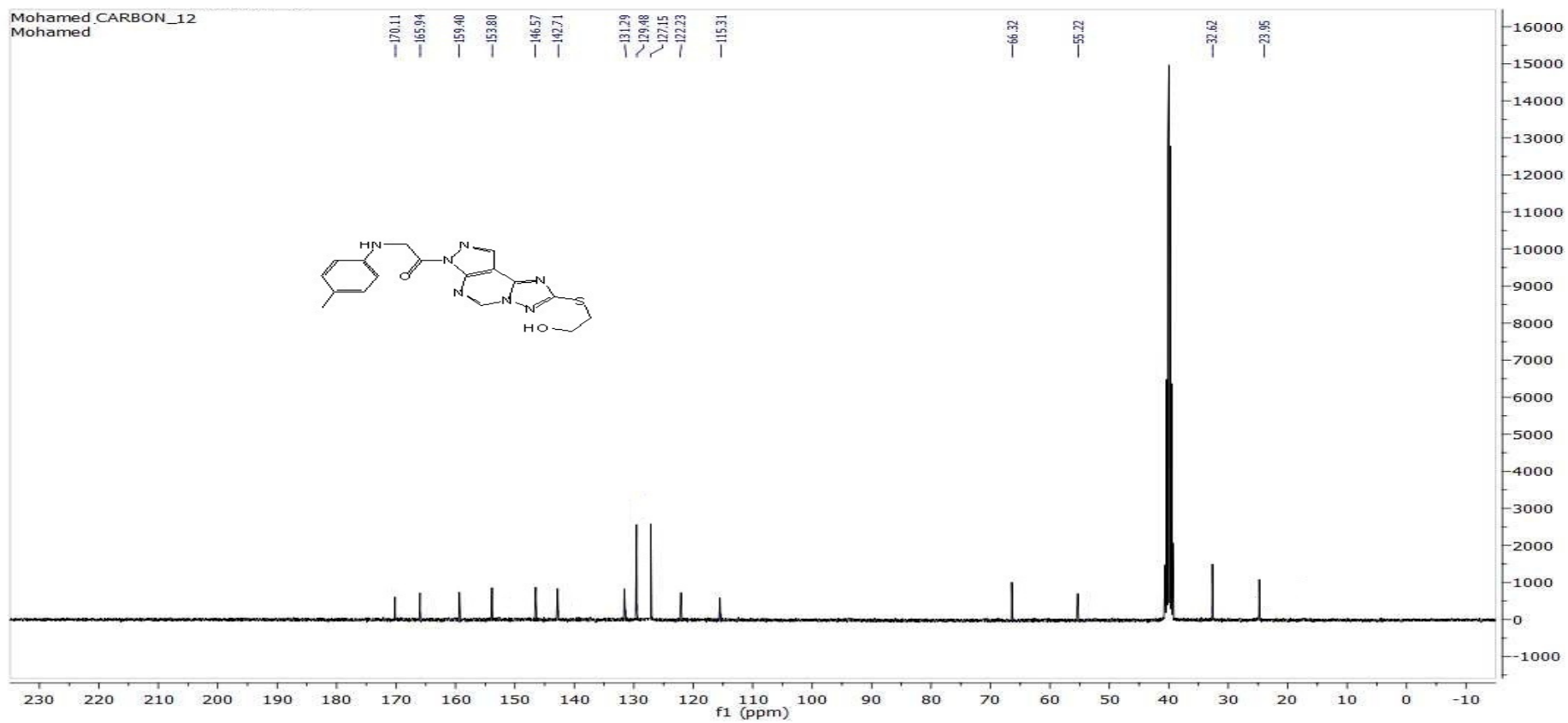
C^{13} -NMR FOR COMP. 12
