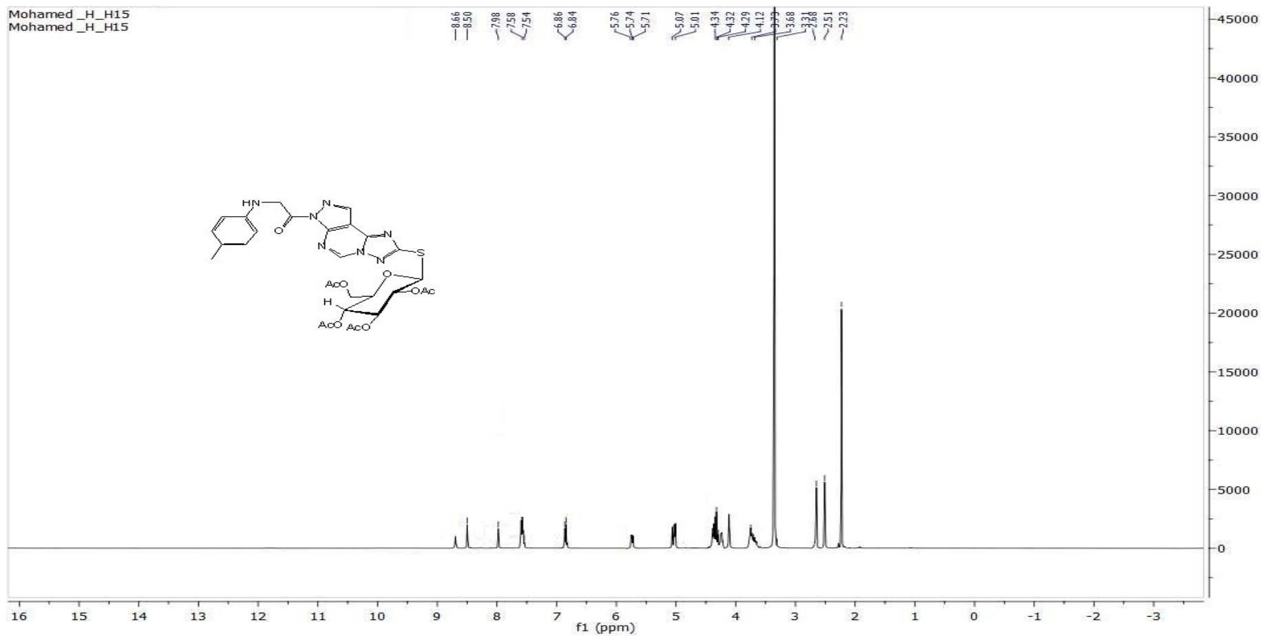
1 H-NMR FOR COMP. 14
