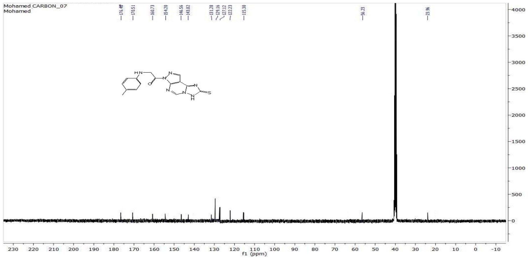
C 13 -NMR FOR COMP. 7
