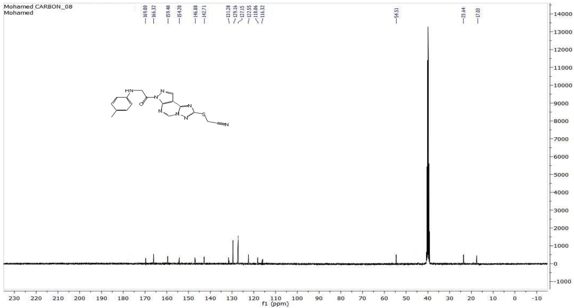
C^{13} -NMR FOR COMP. 8
