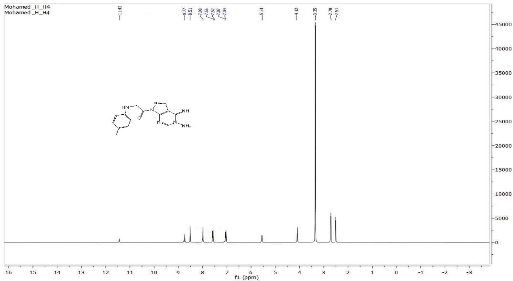
1 H-NMR FOR COMP. 4
