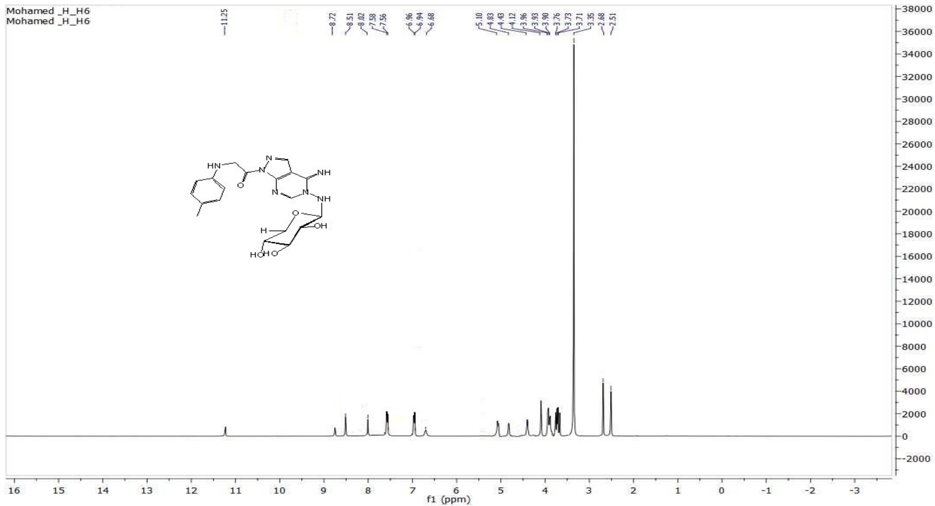
^1\text{H-NMR} FOR COMP. 6
