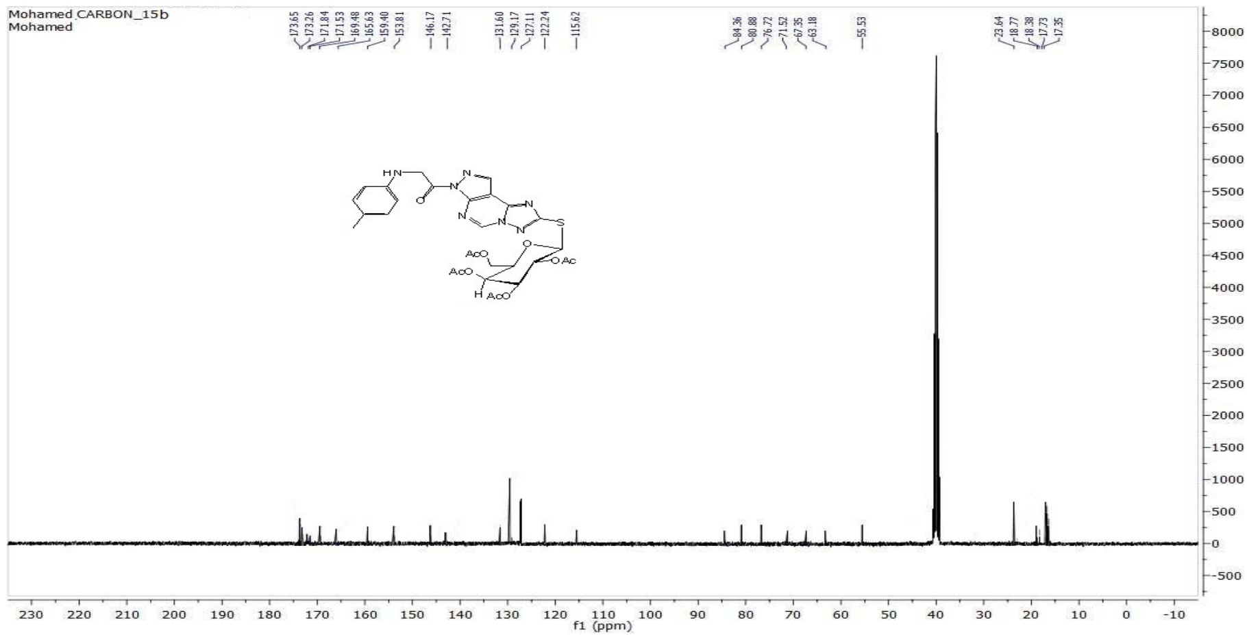
C^{13} -NMR FOR COMP. 15
