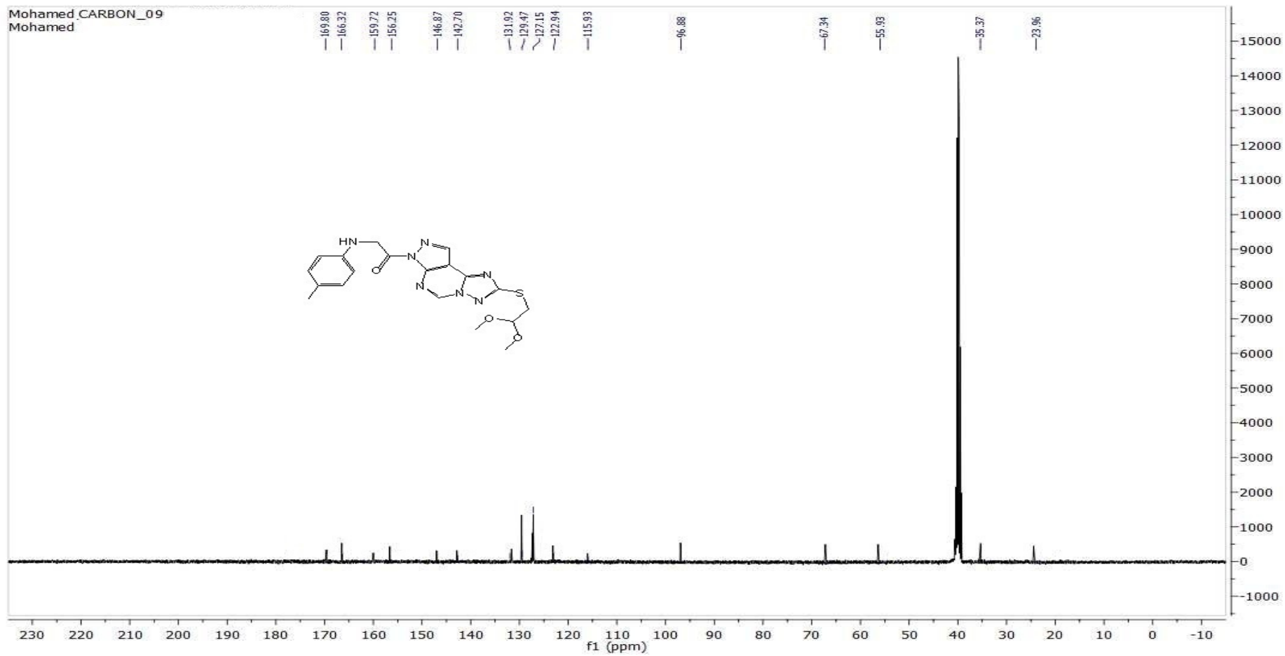
C 13 -NMR FOR COMP. 9
