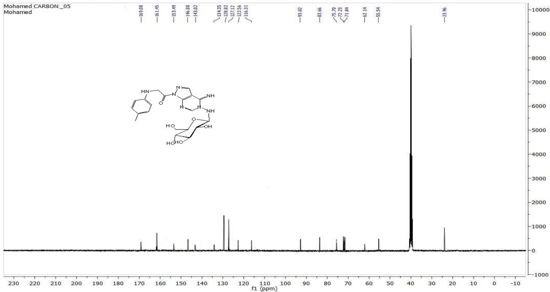
C^{13} -NMR FOR COMP. 5
