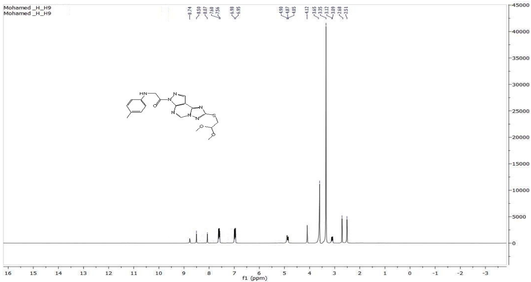
1 H-NMR FOR COMP. 9
