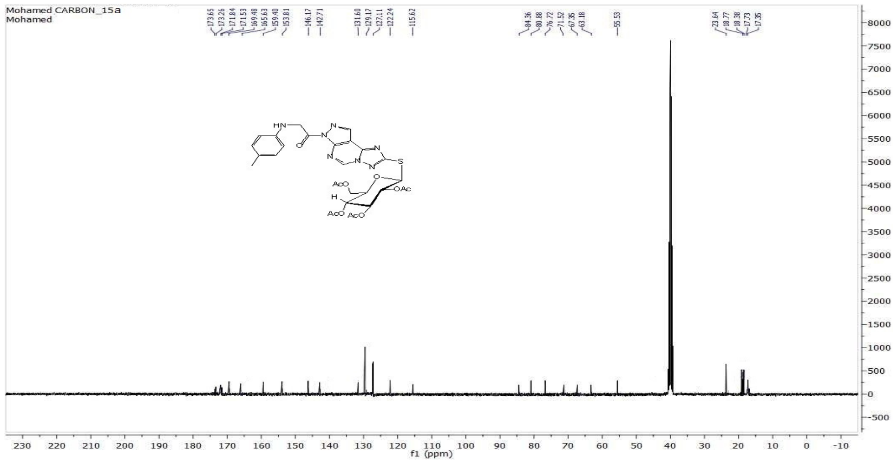
C^{13} -NMR FOR COMP. 14
