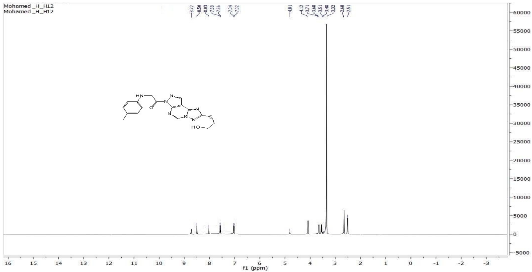
^1\text{H-NMR} FOR COMP. 12
