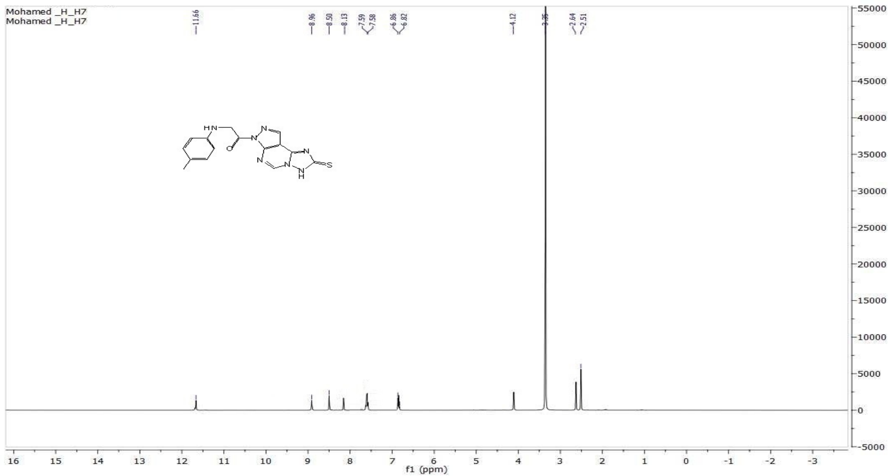
1 H-NMR FOR COMP. 7
