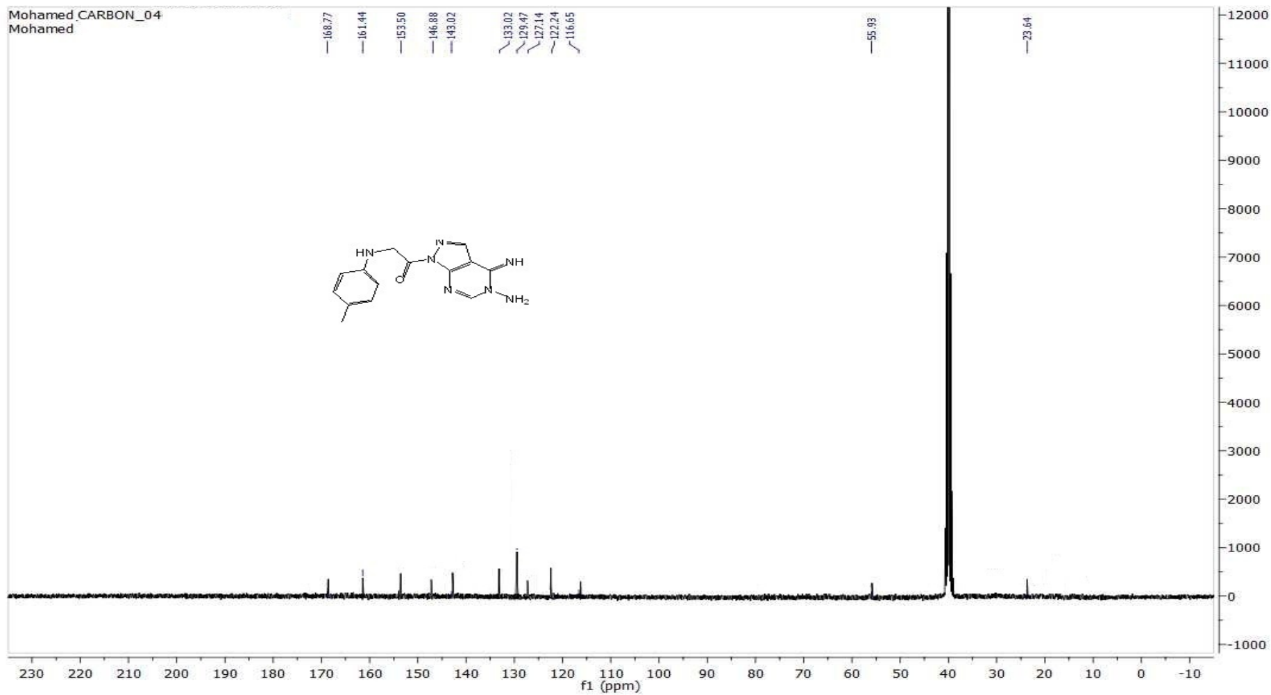
C 13 -NMR FOR COMP. 4
