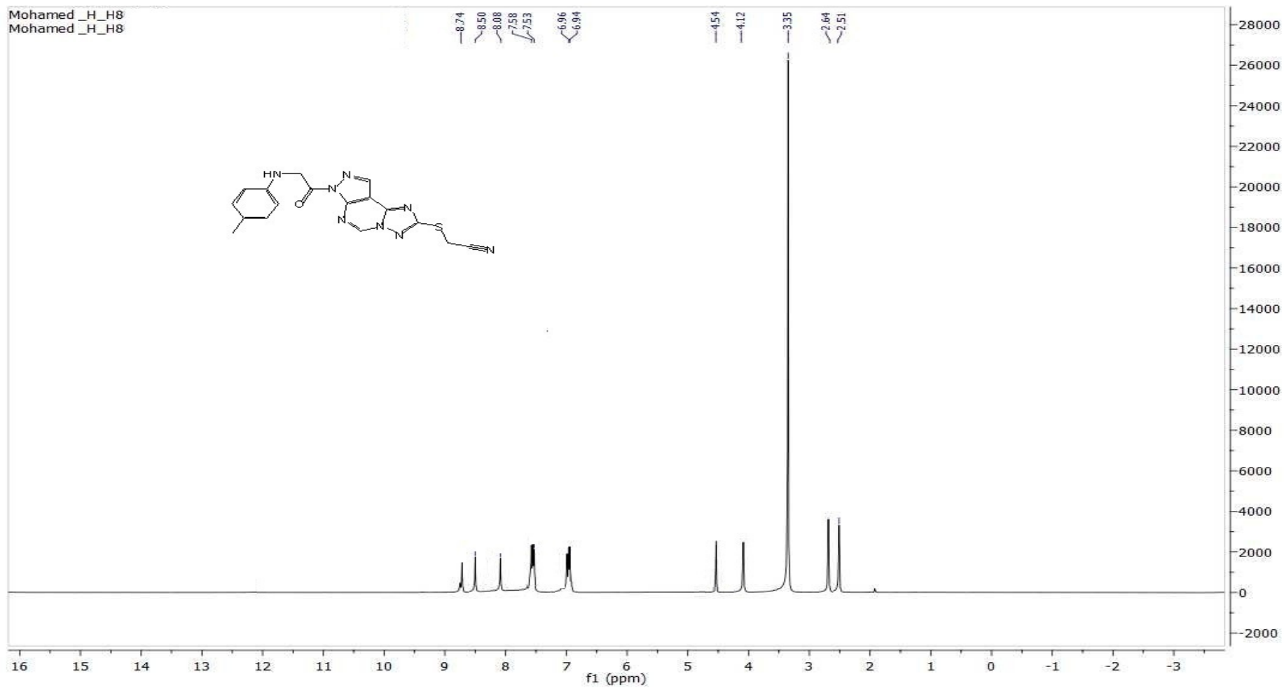
1 H-NMR FOR COMP. 8
