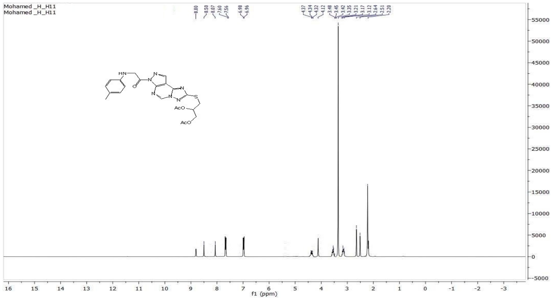
^1\text{H-NMR} FOR COMP. 11
