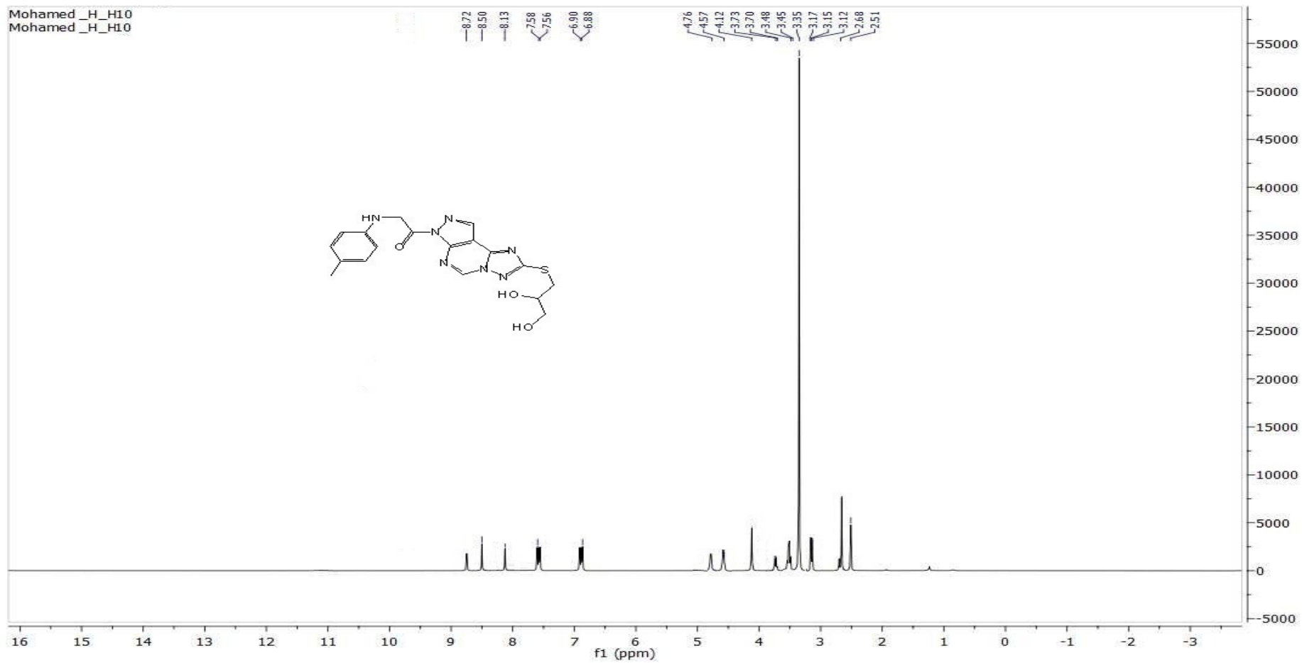
^1\text{H-NMR} FOR COMP. 10
