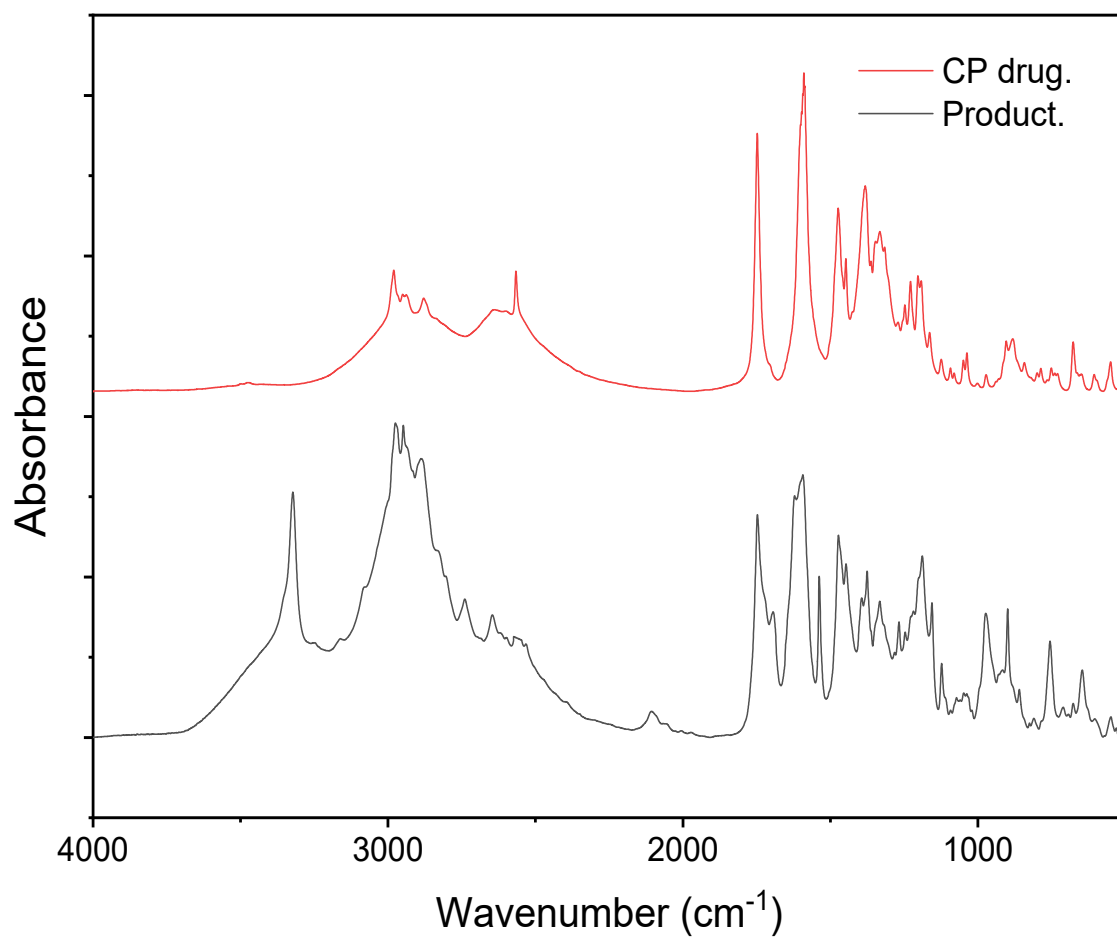
ESI, 1†: The confirmational FTIR spectra of pure CP drug and the developed product.
