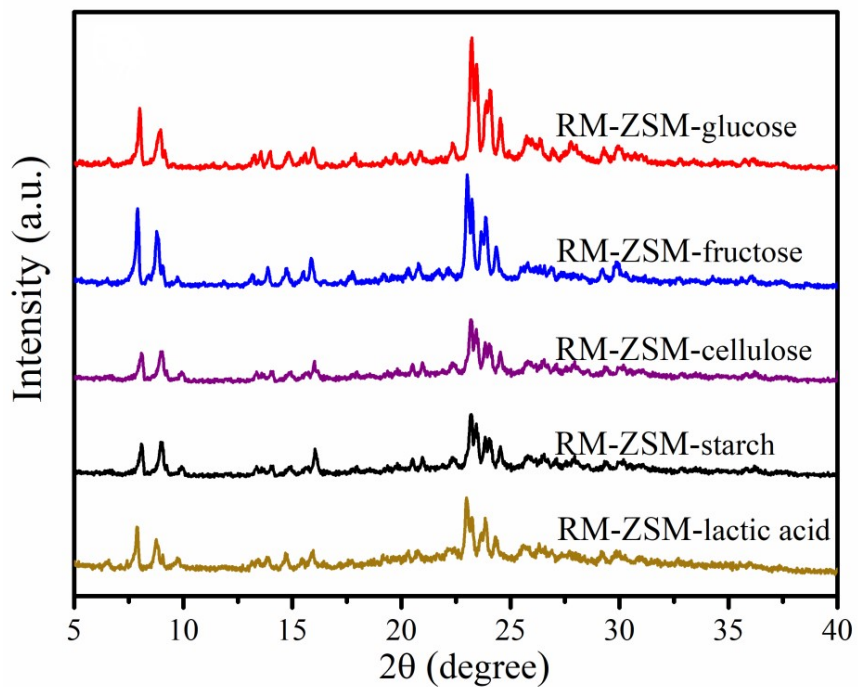
Fig.A.1. XRD patterns of RM-ZSM zeolites from adding different kinds of saccharides.
