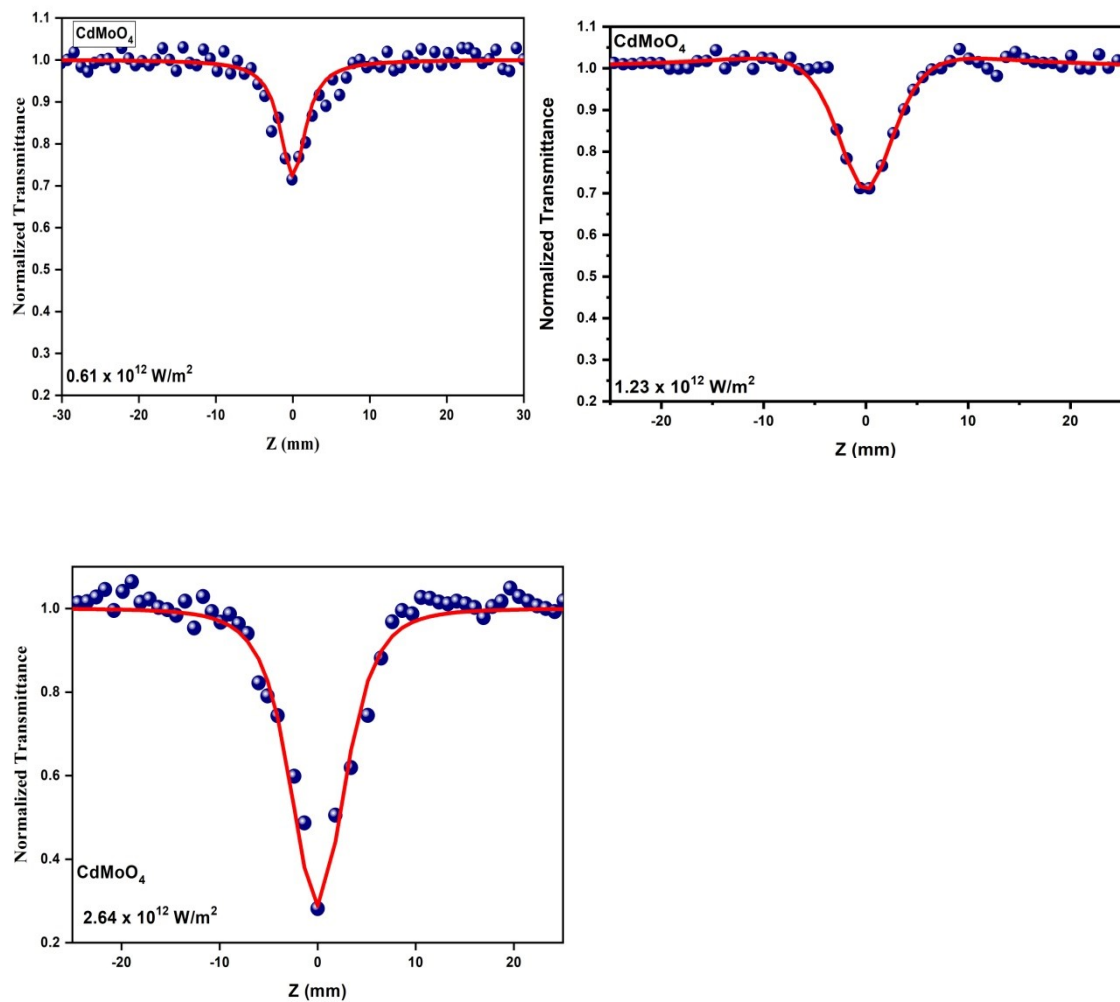
Fig. 1 Intensity dependent open aperture Z-scan graph for pure CdMoO 4 nanostructures
