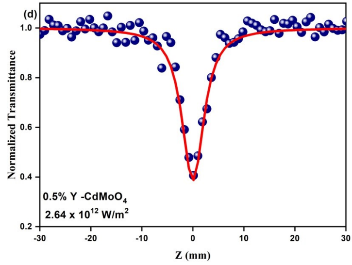
Fig. 2 Intensity dependent open aperture Z-scan graph for 0.5 % Y 3+ doped CdMoO 4 nanostructures
