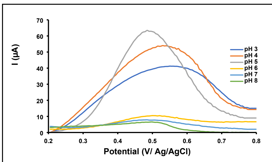
Supplementary 2. DPASV voltammogram of 0.1 μM Ni(II) on Ni-IPANI/CPE-Bi electrode at various pH
