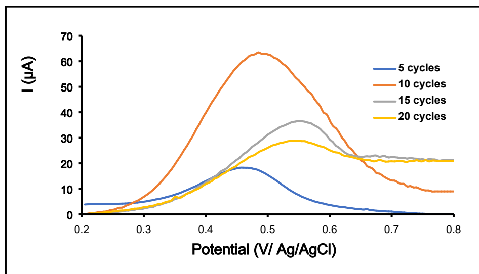
Supplementary 1. DPASV voltammogram of 0.1 μM Ni(II) on Ni-IPANI/CPE-Bi electrode at various scanning cycle
