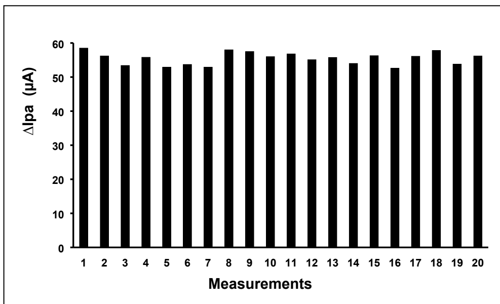
Supplementary 4. Peak current response of 1 \mu M Ni(II) on Ni-IPANI/CPE-Bi electrode for 20 repetitive measurements
