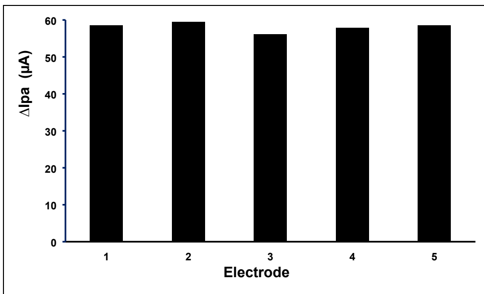
Supplementary 3. Peak current response of 1 \mu M Ni(II) on five different Ni-IPANI/CPE-Bi electrode
