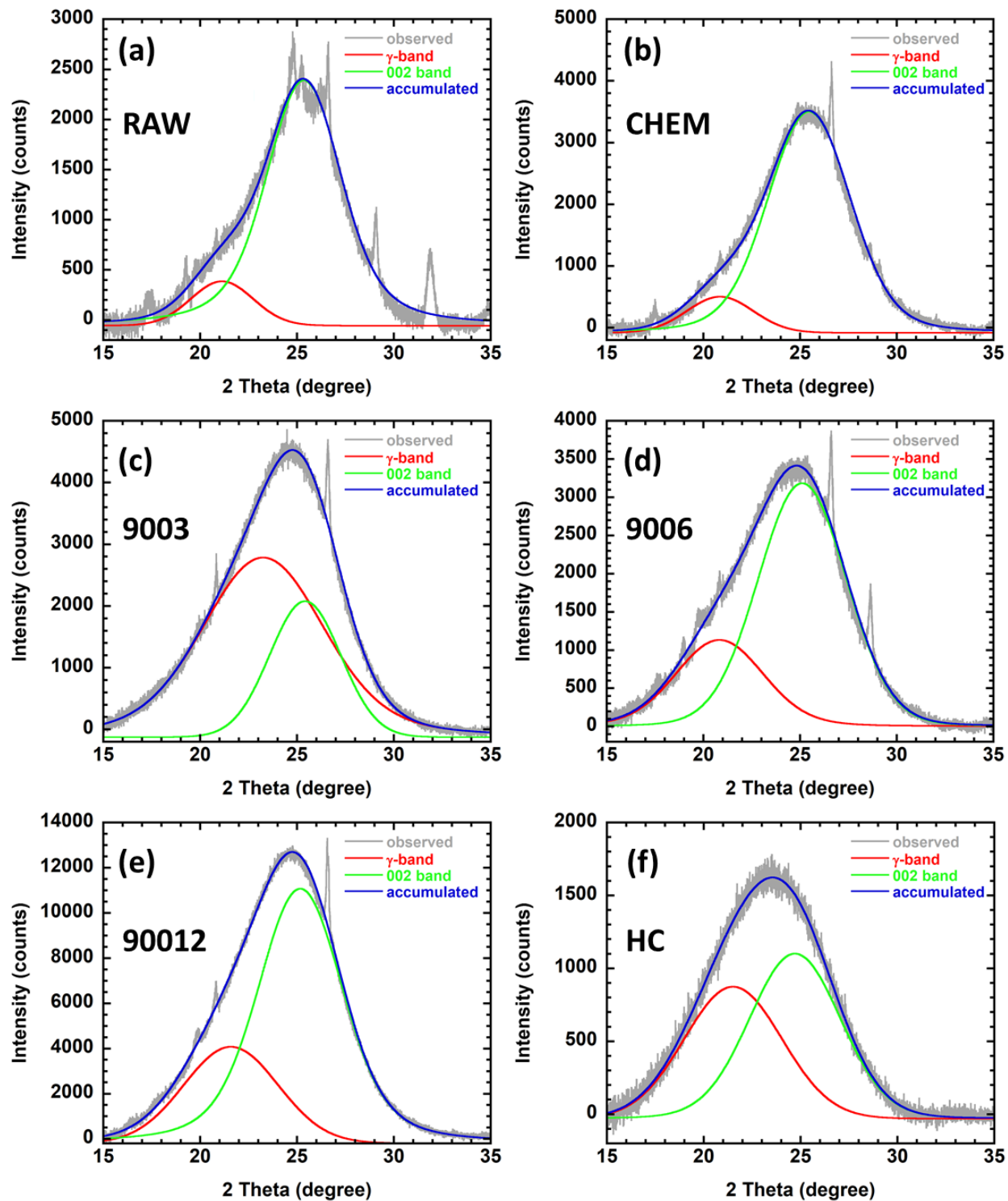
Figure S1. The XRD fitting of (a) RAW, (b) CHEM, (c) 9003, (d) 9006, (e) 90012, and (f) HC samples.
