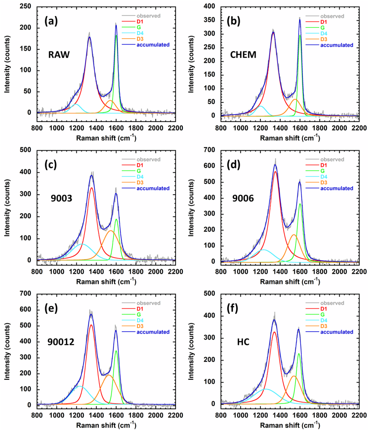
Figure S2. The Raman fitting of (a) RAW, (b) CHEM, (c) 9003, (d) 9006, (e) 90012, and (f) HC samples.
