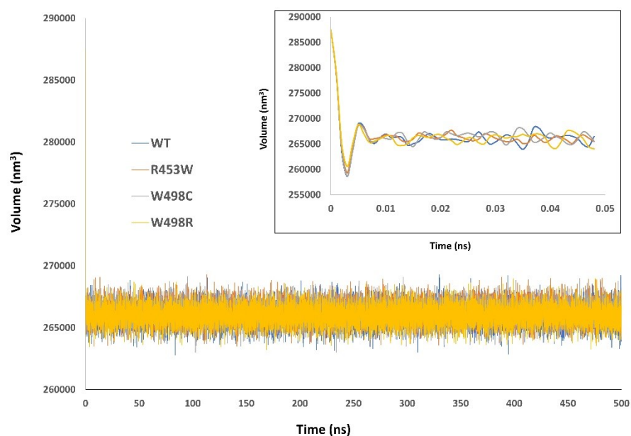
Supplementary Figure 1. Alteration of the volume of the periodic box during MD simulation with time are shown here for the wild type and the mutant Ig fold lamin A proteins. The inset shows volume change with time in the beginning of production run.
