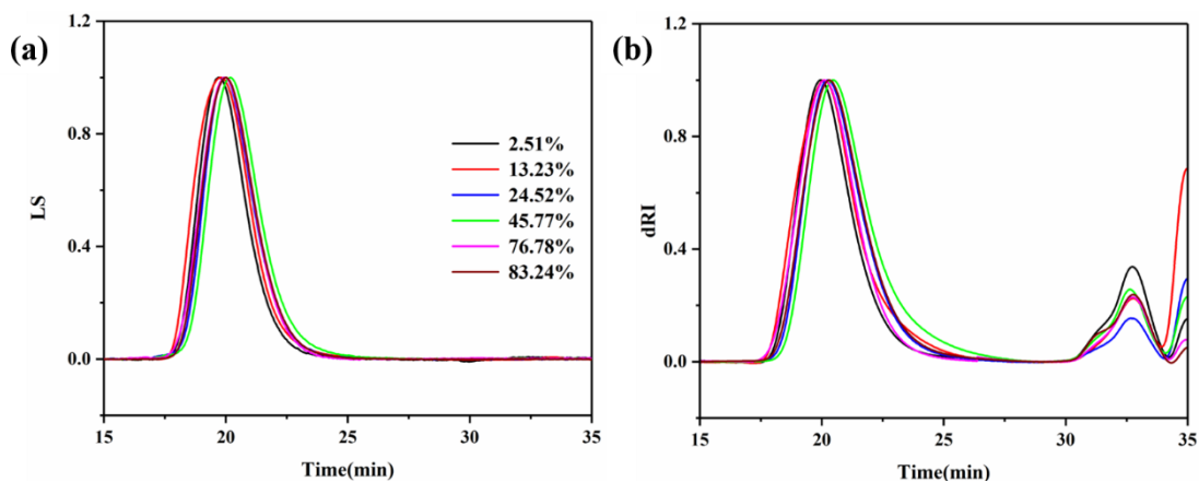
Fig. S2 MGPC Curves of bulk polymers of MMA with 6% pre-dissolved HWM-PMMA at different conversion, (a) LS, (b) dRI
