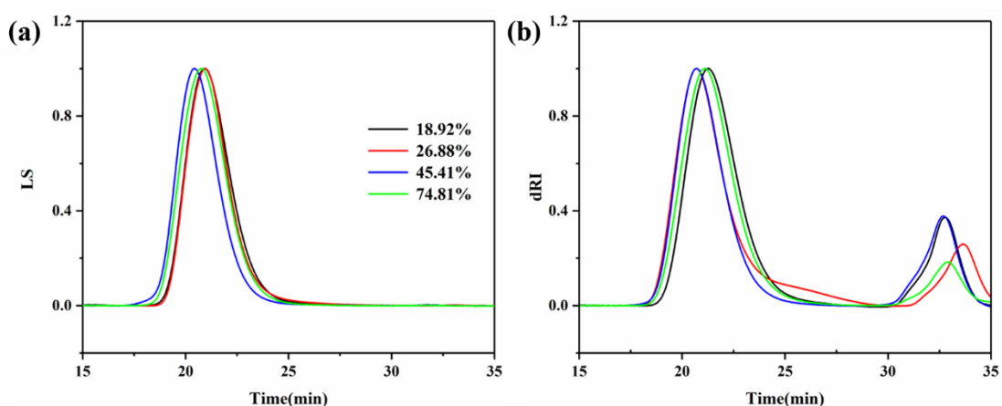
Fig. S1 MGPC Curves of bulk polymers of pure MMA at different conversion, (a) LS, (b) dRI
