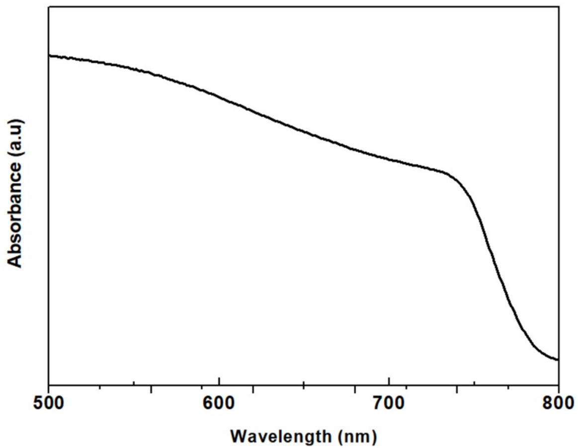
Fig. S3 Absorption spectra of the cell with the structure of ITO/ETL/Perovskite.
