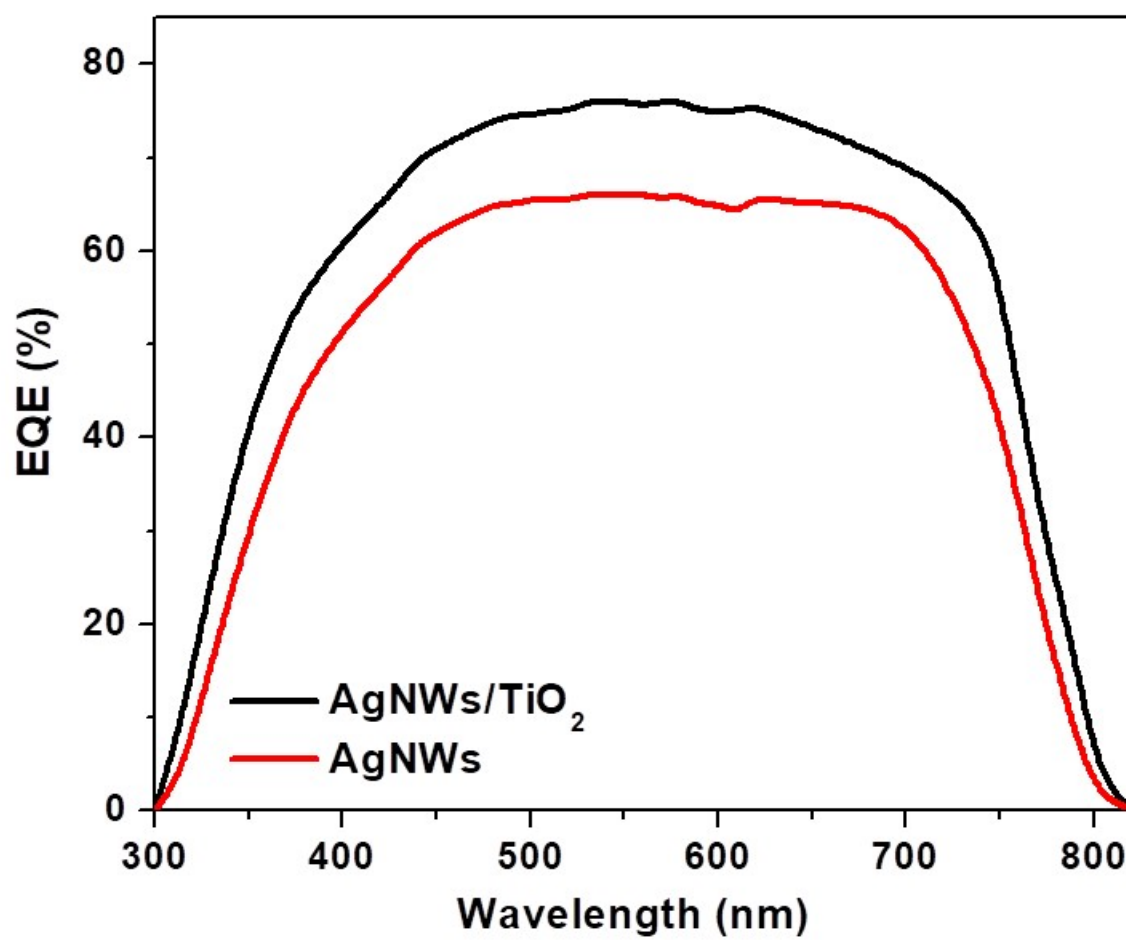
Fig. S2 EQE characteristics of the devices based on AgNWs and AgNWs/TiO 2 hybrid electrode.
