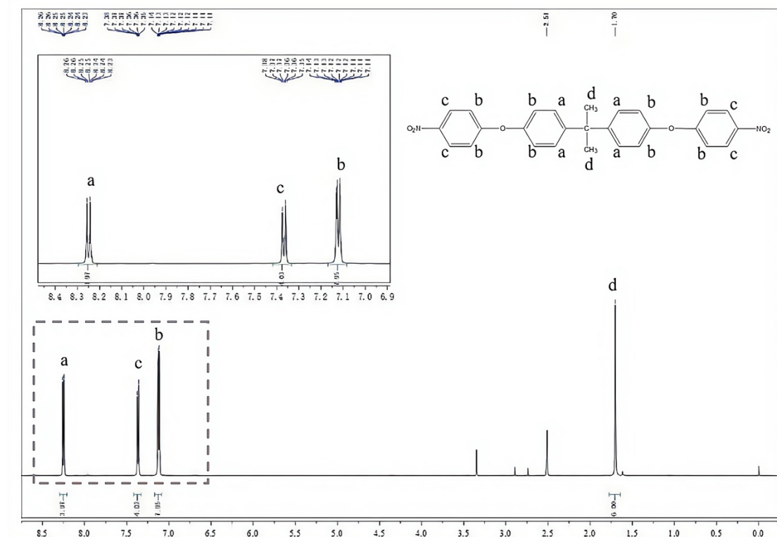
Figure S1. 1 H NMR spectrum of diamine monomer
