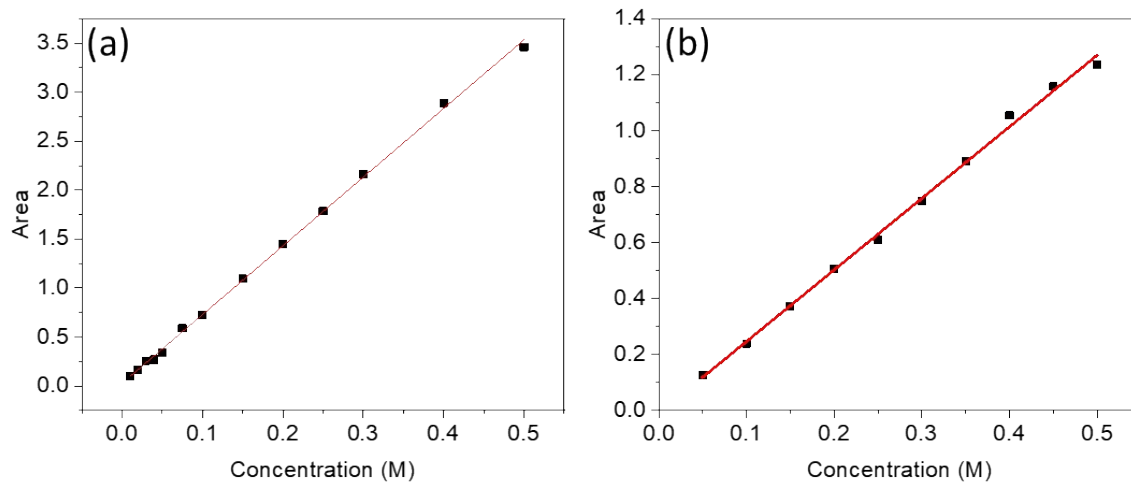
Figure S1: (a) Plot of C=C IR absorbance of PC vs concentration (b) Plot of C=C IR absorbance of PCP vs concentration
