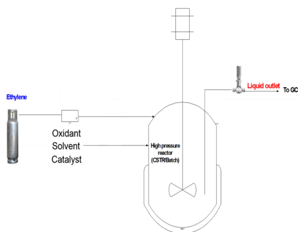
Fig S1. Schematic diagram of the reactor for the production of EO
