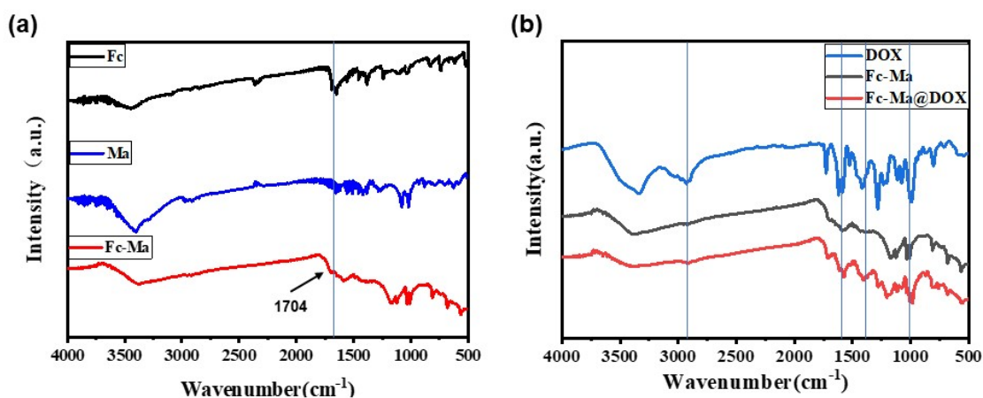
Figure S2. (a) FTIR spectra of prepared precursors and corresponding Fc-Ma; (b) FTIR spectra of Fc-Ma, DOX, and Fc-Ma-DOX.
