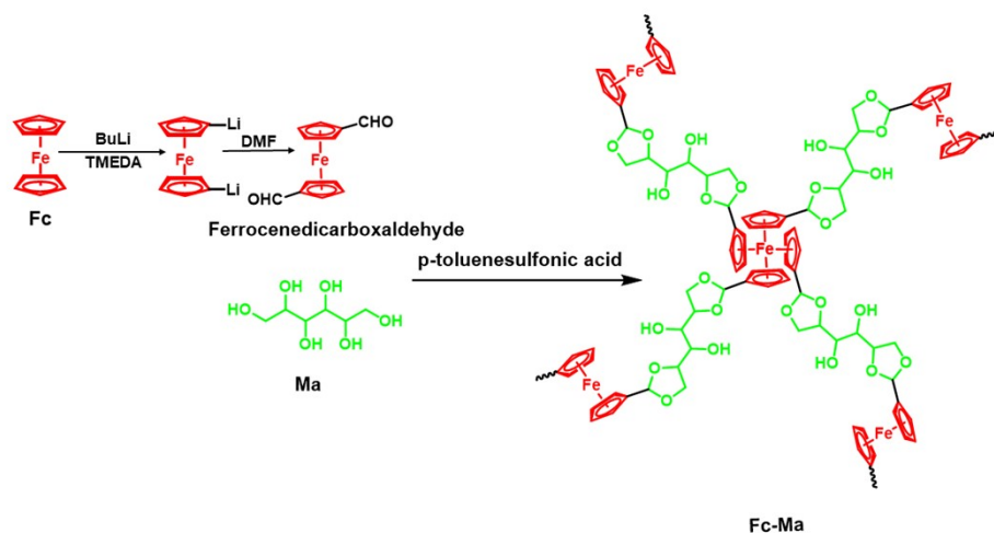
Figure S1. Synthesis of the Fc-Ma.
