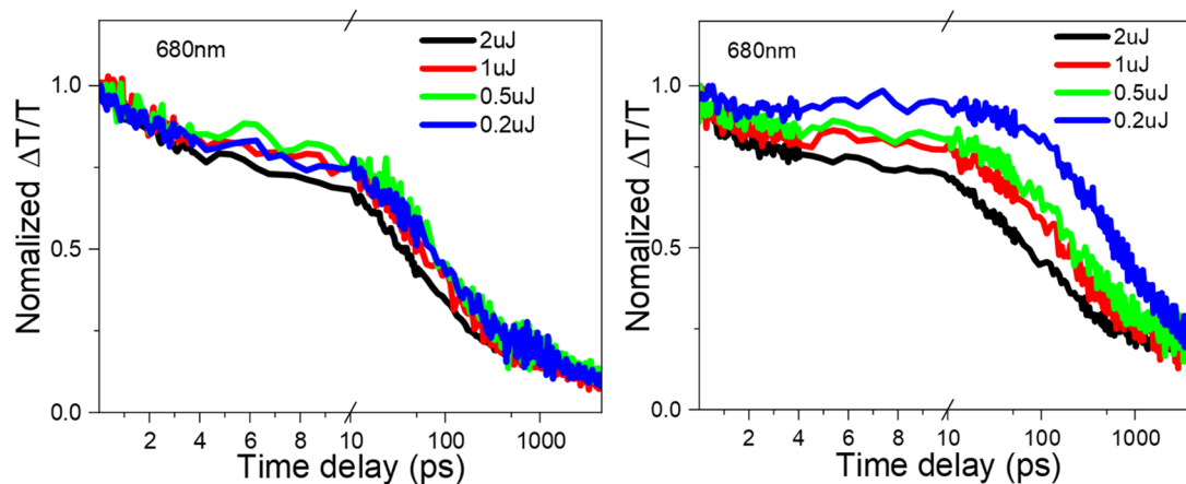
Figure S8. Normalized kinetic decay curves at 680 nm at different excitation fluences of EH-Fla (a) and TIPS-Fla (b) in the film.
