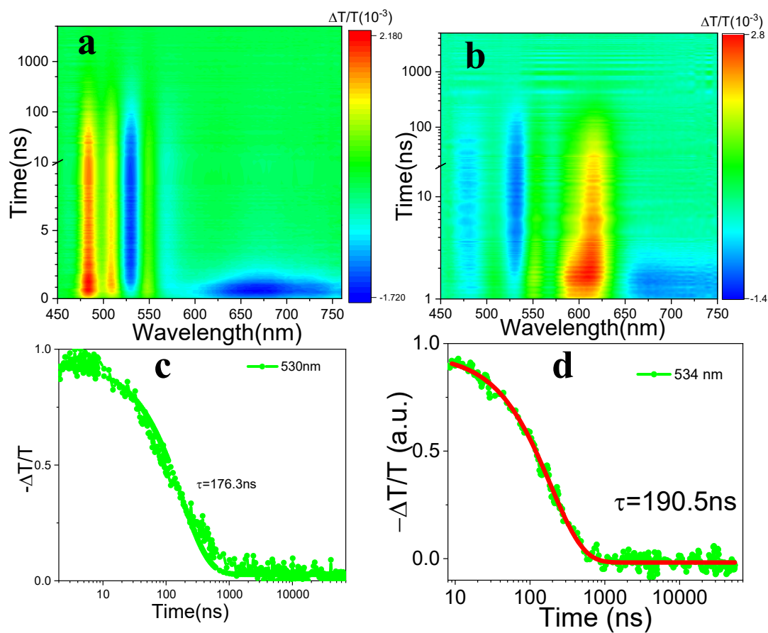
Figure S14. Raw ns-TA spectra of EH-Fla (a) and TIPS-Fla (b) films excited at 365 nm, and the corresponding decay kinetics of EH-Fla at 530 nm and TIPS-Fla at 534 nm.
