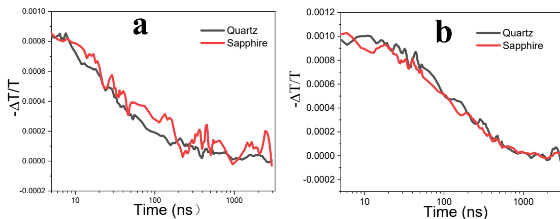
Figure S18. Kinetic curves of EH-Fla (a) and TIPS-Fla (b) on quartz and sapphire substrates from ns-TA spectra.
