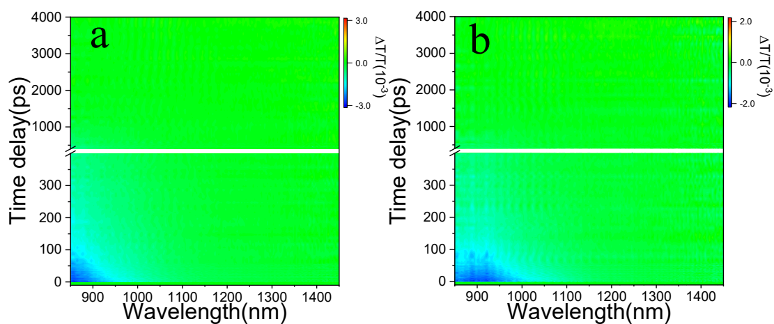
Figure S9. Near-infrared region fs-TA spectra of EH-Fla (a) and TIPS-Fla (b).
