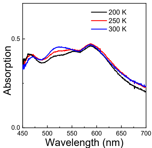
Figure S12. Absorption spectra of TIPS-Fla at different temperatures.
