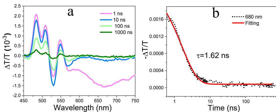
Figure S15. The ns-TA spectra of EH-Fla at different delay times and decay kinetics of at 680 nm.
