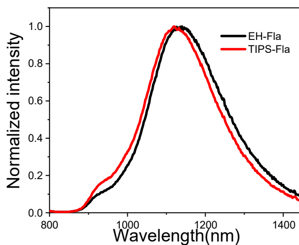
Figure S5. Phosphorescence spectra of EH-Fla and TIPS-Fla in argon-saturated Methyl-tetrahydrofuran containing MeI (10 mM) at 77 K.
