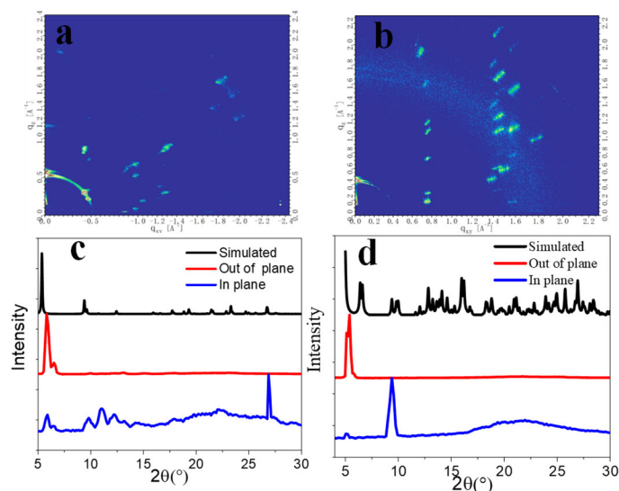
Figure S1. Comparison of the in-plane and out-of-plane line cuts from GIWAXS with simulated powder patterns (black lines) of EH-Fla (a, c) and TIPS-Fla (b, d).
