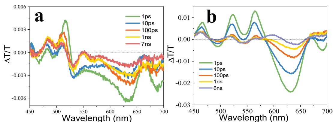
Figure S16. Fs-TA spectra of EH-Fla (a) and TIPS-Fla (b) film doped \text{PdPc}(\text{OBu})_8 excited at 720 nm.
