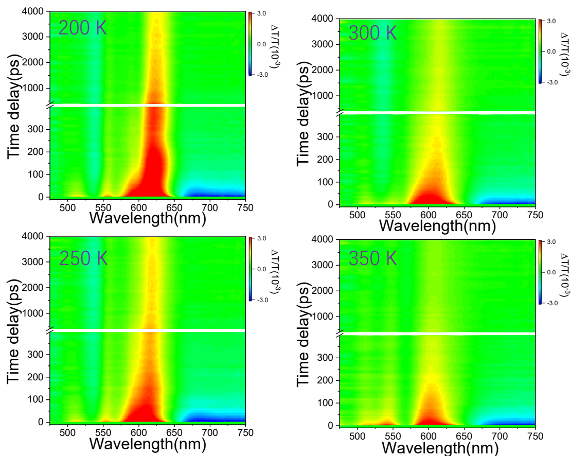
Figure S10. The fs-TA spectra of TIPS-Fla at different temperatures.
