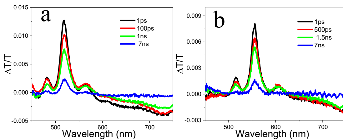
Figure S6. Fs-TA spectra of EH-Fla (a) and TIPS-Fla (b) excited at 400 nm in dilute dichloromethane solutions.
