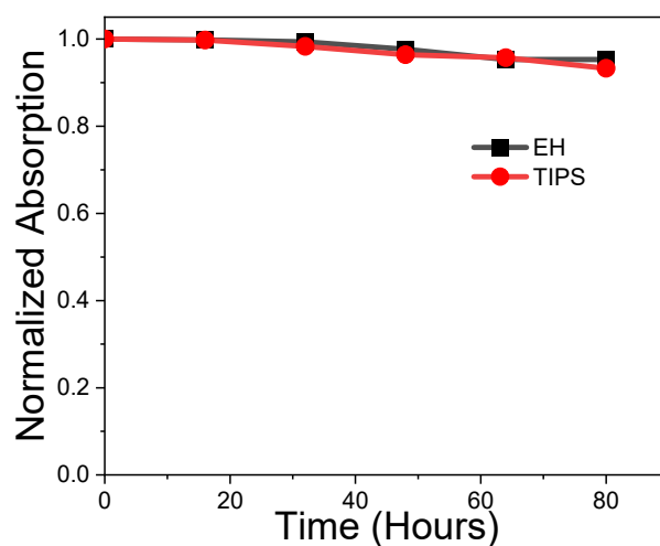
Figure S3. Normalized intensity of the \lambda_{\text{max}} of the steady-state absorption spectra of EH-Fla and TIPS-Fla thin films under 365 nm 18 W UV lamp irradiation.
