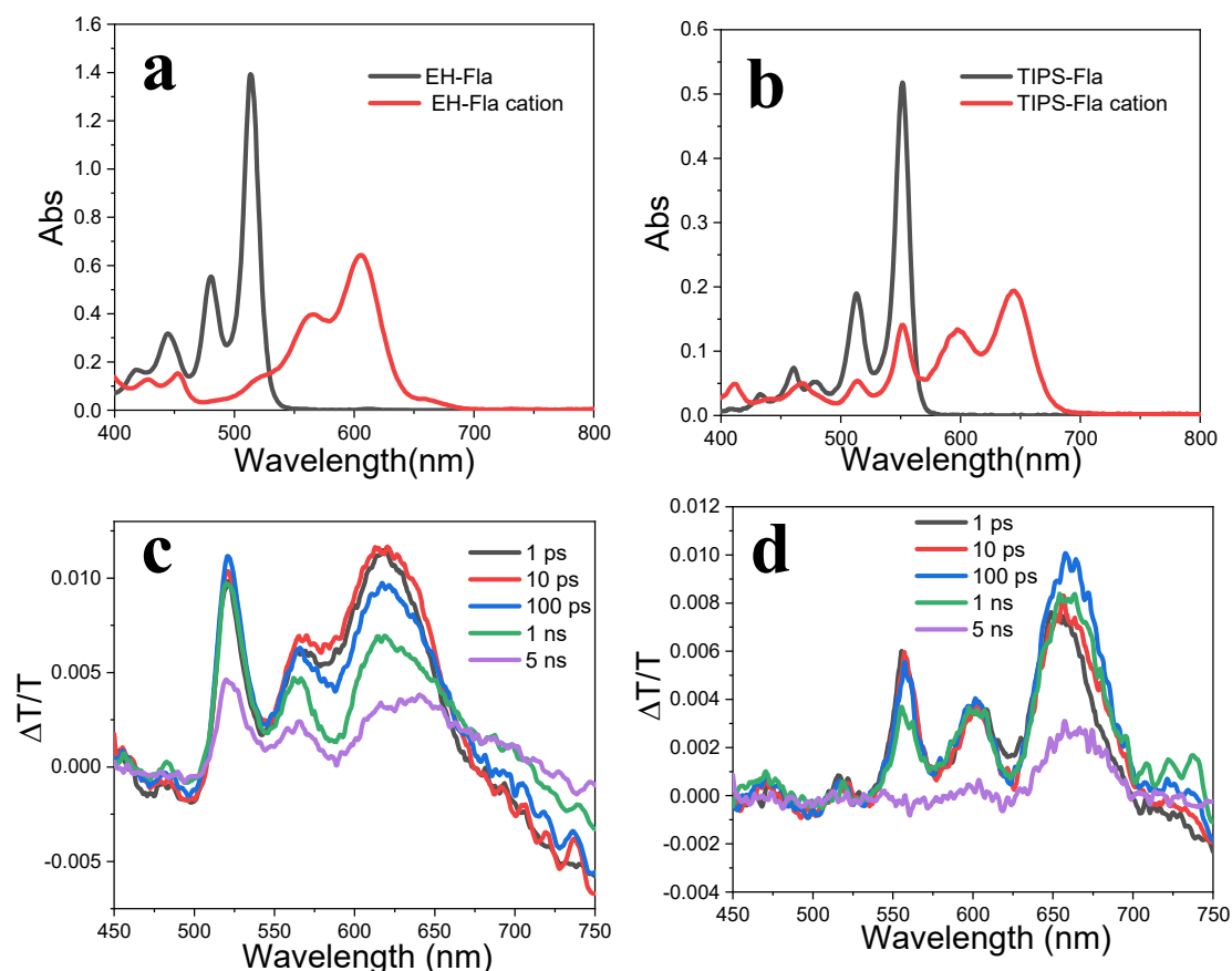
Figure S7. The absorption spectra of EH-Fla in dichloromethane and EH-Fla cation produced by adding hydrochloric acid. Figure b, the absorption spectra of TIPS-Fla in dichloromethane and TIPS-Fla cation produced by adding hydrochloric acid. Figure c, d. fs-TA of EH-Fla cations (c) and TIPS-Fla cations (d) excited at 400 nm in dichloromethane.
