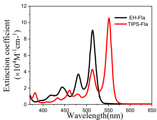
Figure S4. The steady-state absorption spectra of EH-Fla and TIPS-Fla in dichloromethane.
