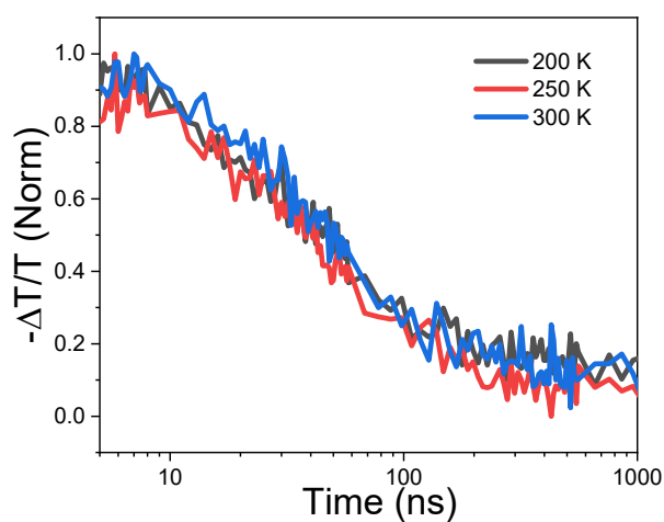
Figure S13. The kinetic curves of TIPS-Fla at 536 nm at different temperatures.
