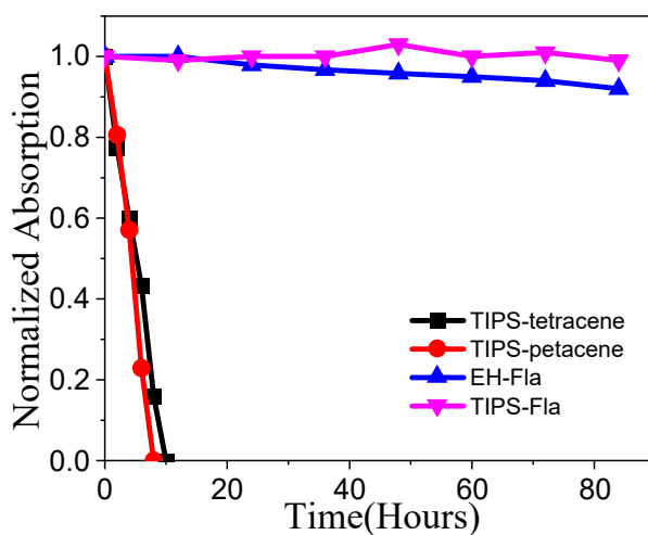
Figure S2. Normalized intensity of the absorbance at the maximum absorption wavelength ( \lambda_{\max} ) of the steady-state absorbance spectra of flavanhenre derivatives, TIPS-tetracene and TIPS-pentacene in toluene solutions under 365 nm 18 W UV lamp irradiation.
