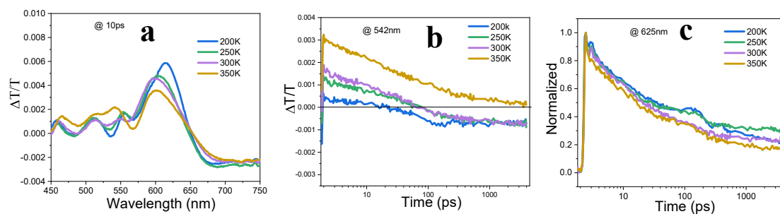
Figure S11. a) The fs-TA spectra of TIPS-Fla at 10 ps at different temperatures. b) The kinetic curves of TIPS-Fla at 542 nm at different temperatures. c) The kinetic curves of TIPS-Fla at 625 nm at different temperatures.
