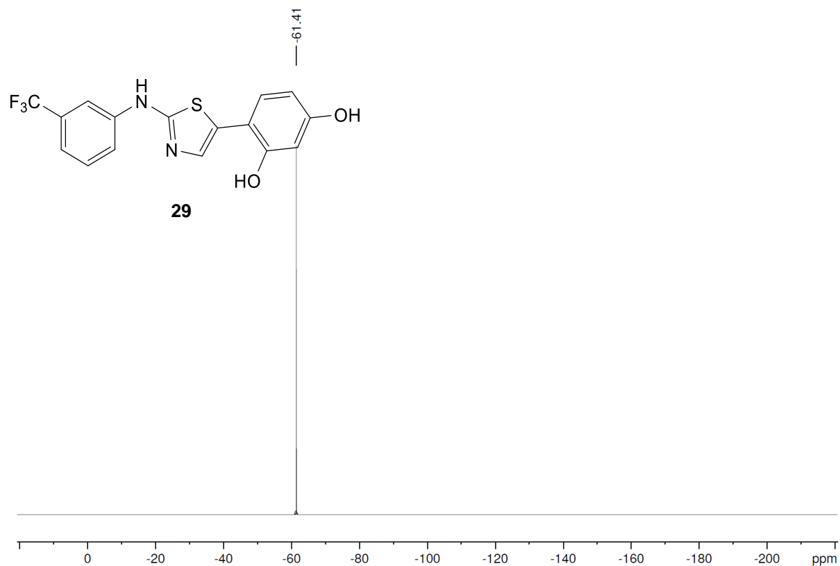
Spectrum 43: ^{19}\text{F} NMR of aminothiazole 29 .
