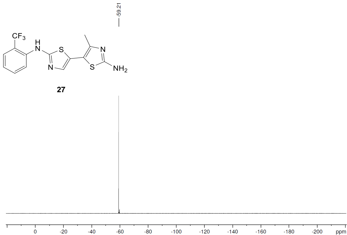
Spectrum 35: ^{19}\text{F} NMR of aminothiazole 27 .
