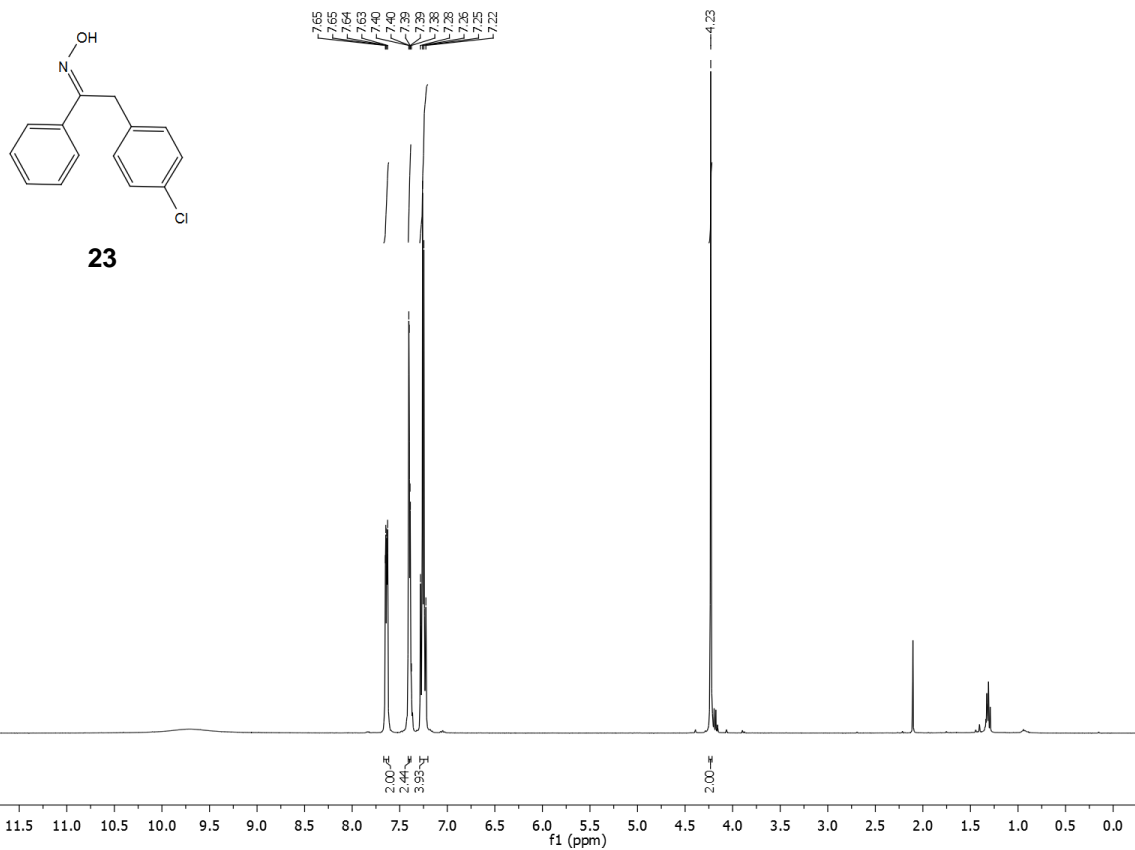
Spectrum 20: 1 H NMR of oxime 23 .
