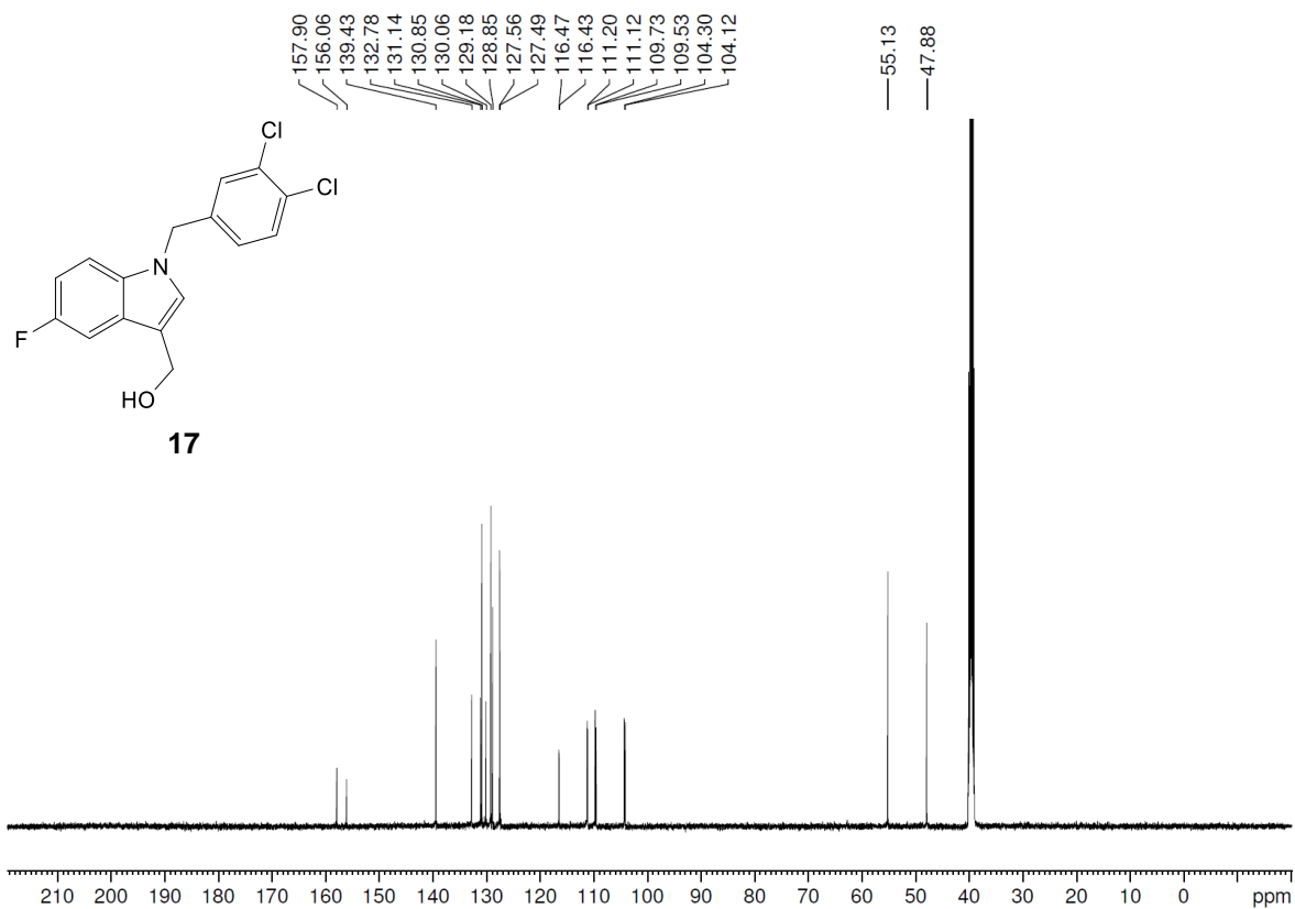
Spectrum 5: ^{13}\text{C} NMR of indole 17 .
