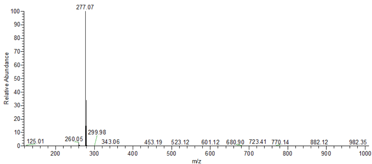
Spectrum 19: HR-ESI-MS spectrum of oxime 21 .
