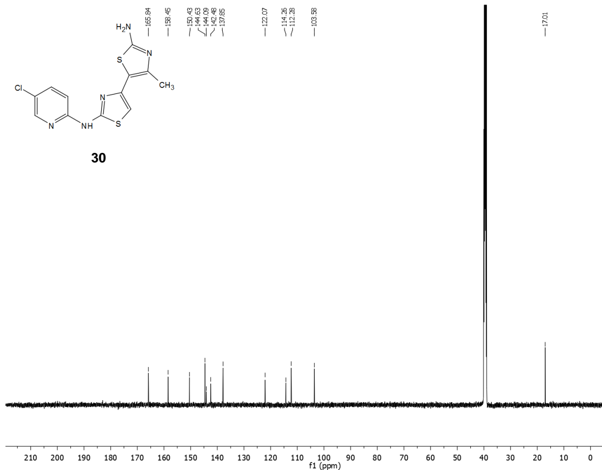
Spectrum 46: ^{13}\text{C} NMR of aminothiazole 30 .
