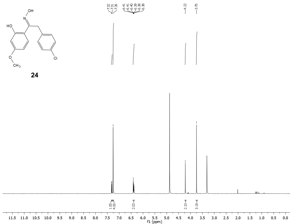
Spectrum 23: 1 H NMR of oxime 24 .
