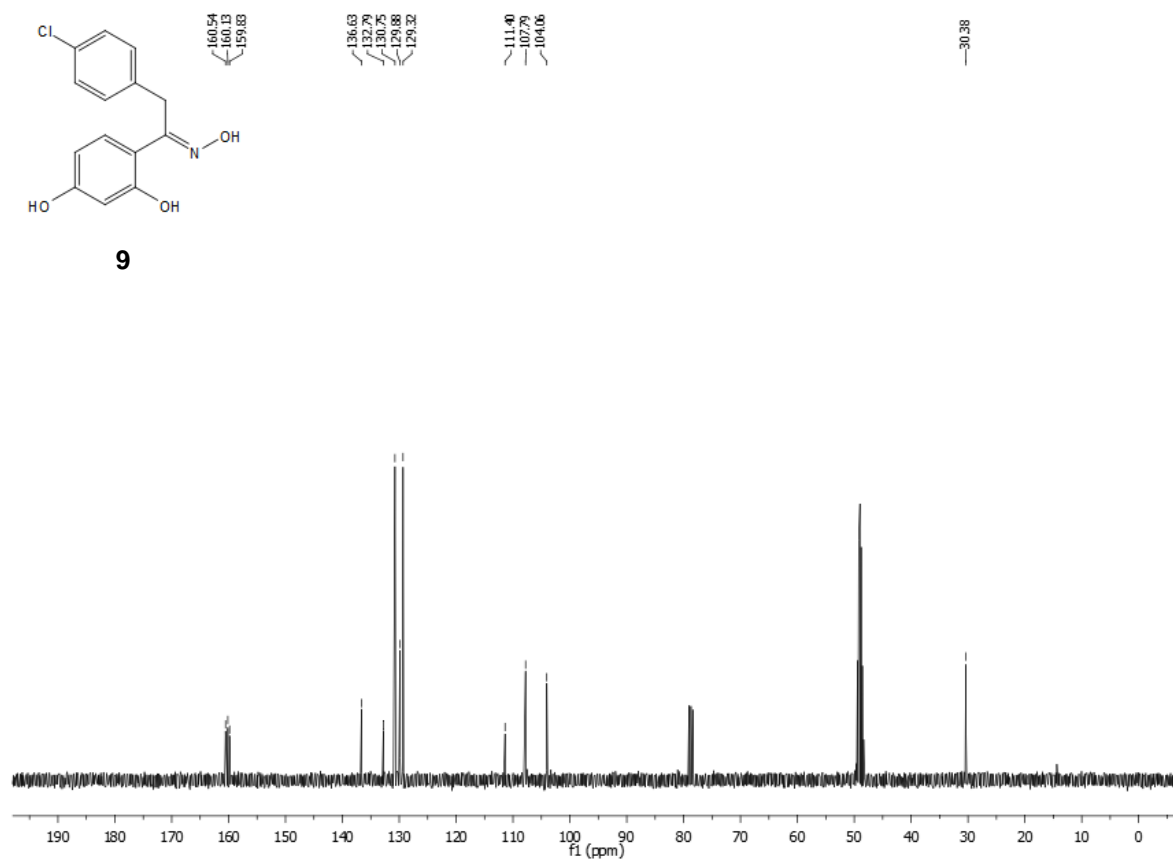
Spectrum 15: 13 C NMR of oxime 9.
