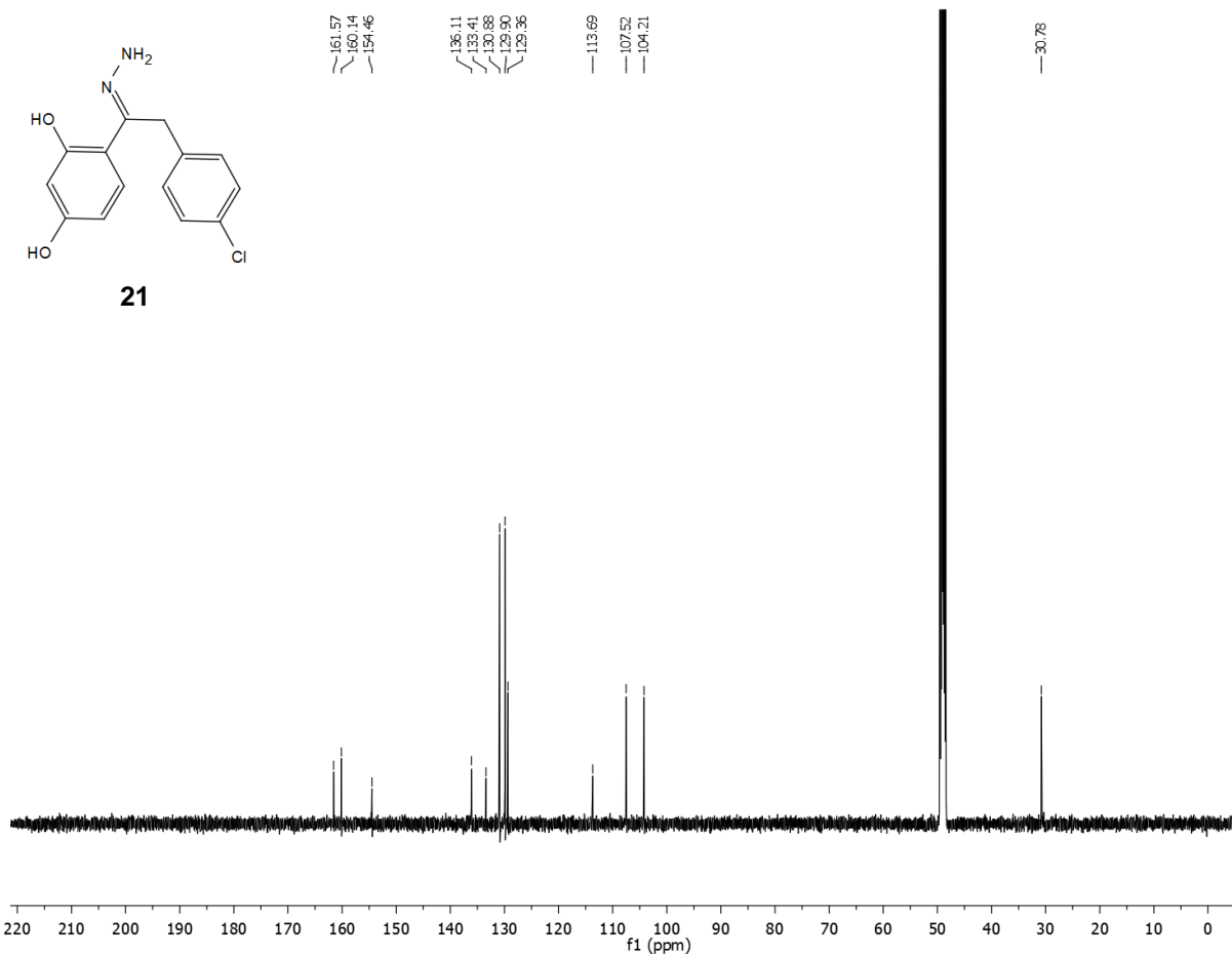
Spectrum 18: ^{13}\text{C} NMR of oxime 21 .
