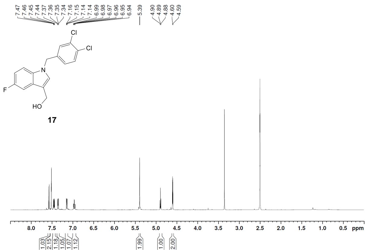
Spectrum 4: ^1H NMR of indole 17.
