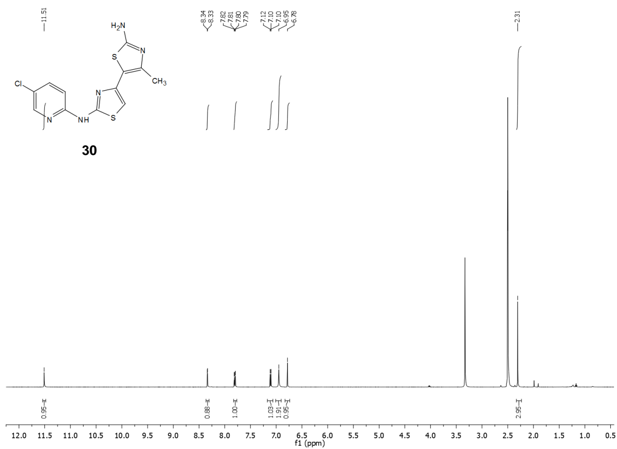
Spectrum 45: 1 H NMR of aminothiazole 30 .
