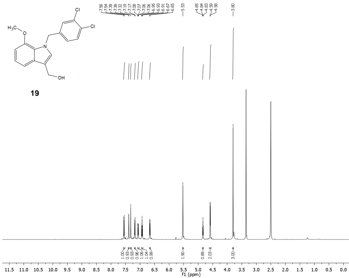
Spectrum 11: ^1\text{H} NMR of indole 19 .
