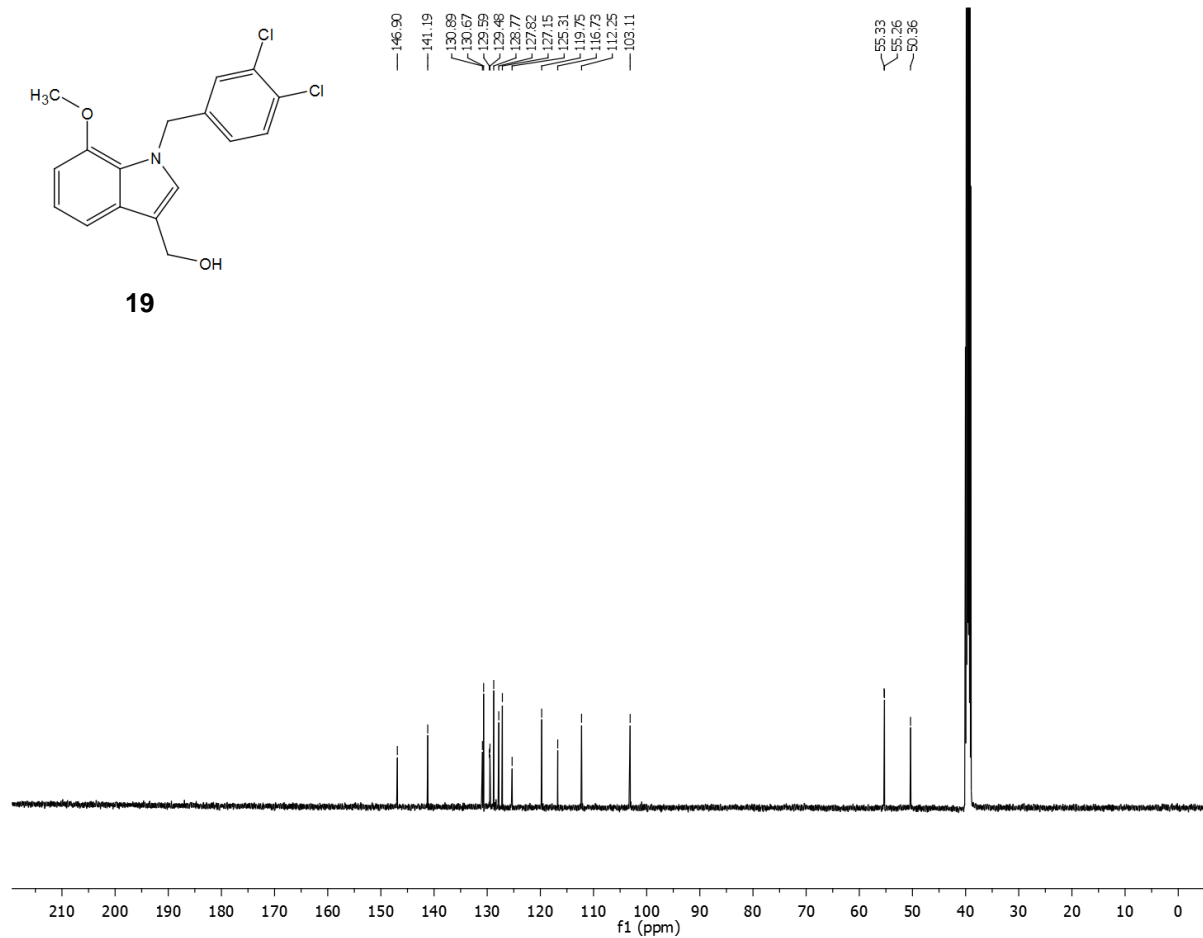
Spectrum 12: 13 C NMR of indole 19 .
