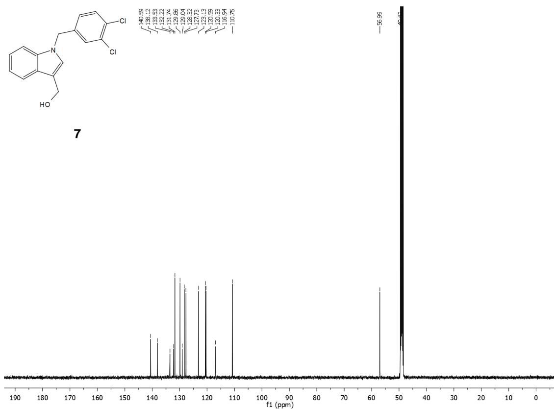
Spectrum 2: 13 C NMR of indole 7 .
