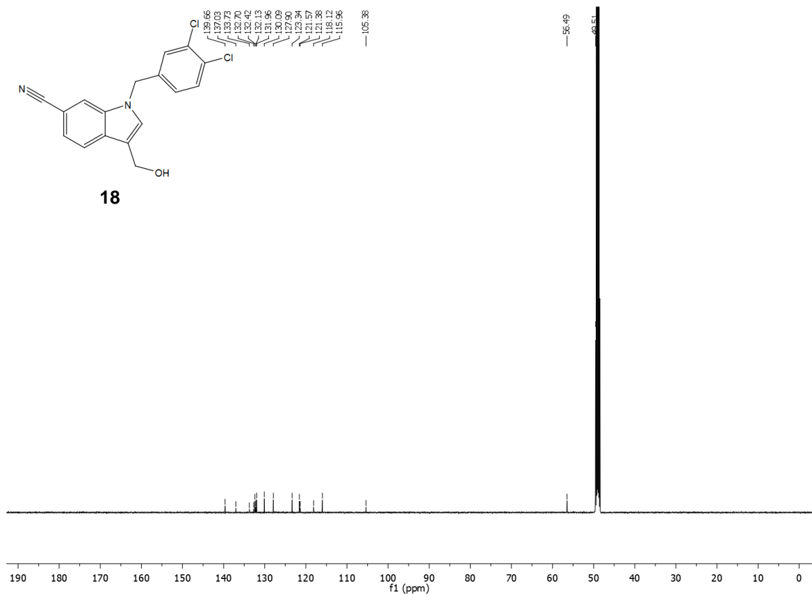
Spectrum 9: ^{13}\text{C} NMR of indole 18.
