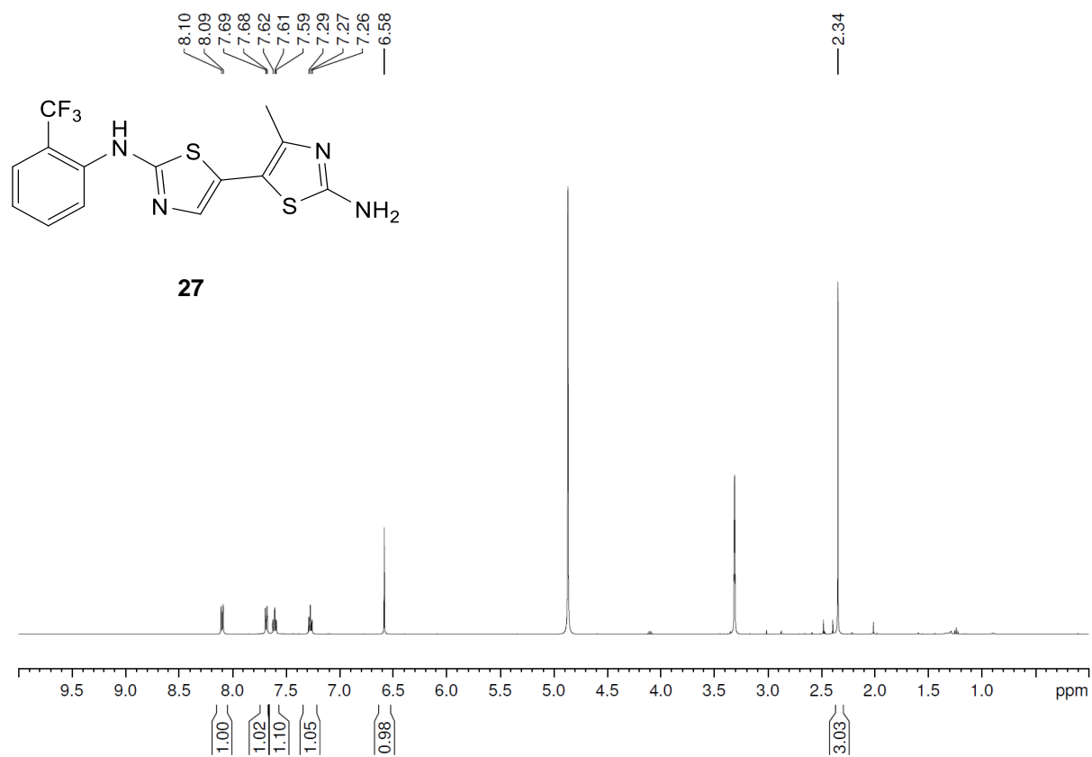
Spectrum 33: 1 H NMR of aminothiazole 27 .
