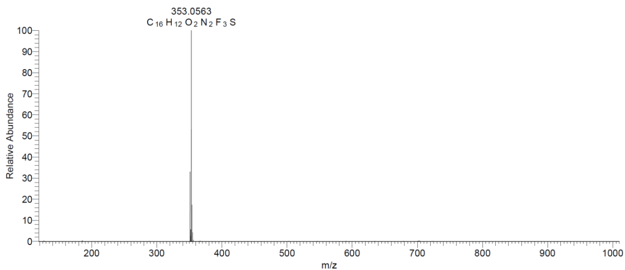
Spectrum 44: HR-ESI-MS spectrum of aminothiazole 29 .
