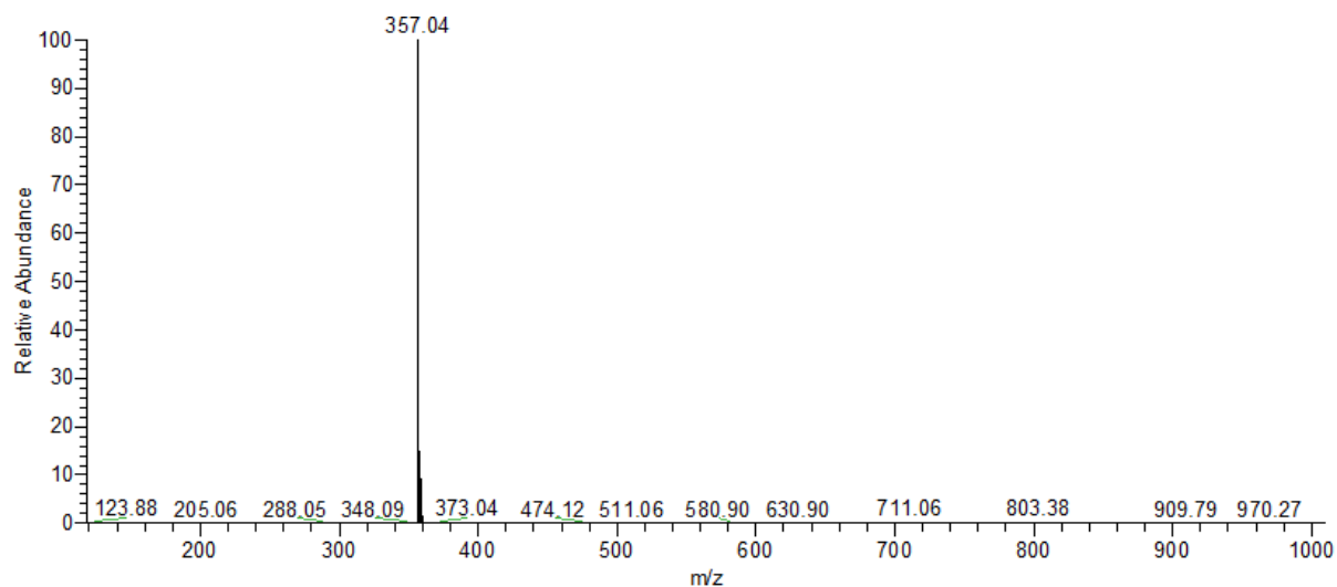
Spectrum 40: HR-ESI-MS spectrum of aminothiazole 28 .
