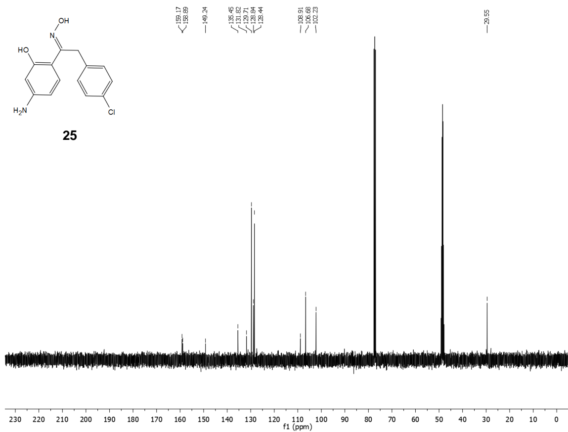
Spectrum 27: 13 C NMR of oxime 25 .
