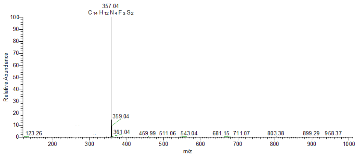
Spectrum 32: HR-ESI-MS spectrum of aminothiazole 10 .
