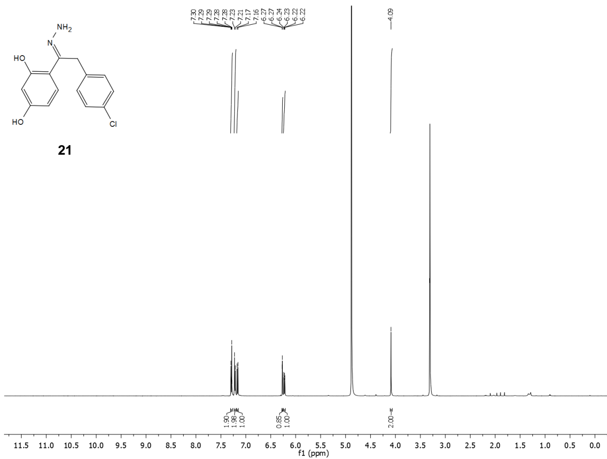
Spectrum 17: ^1\text{H} NMR of oxime 21 .
