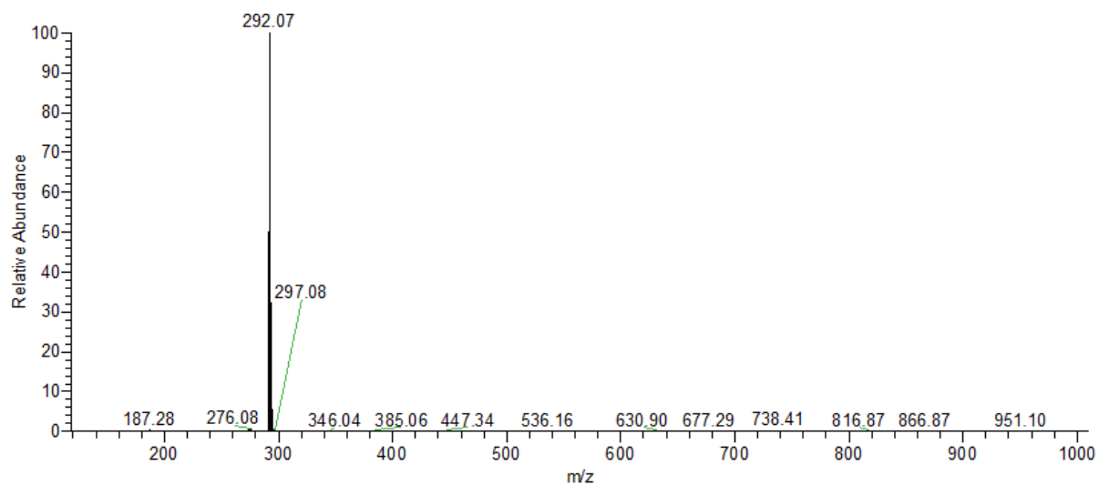
Spectrum 25: HR-ESI-MS spectrum of oxime 24 .
