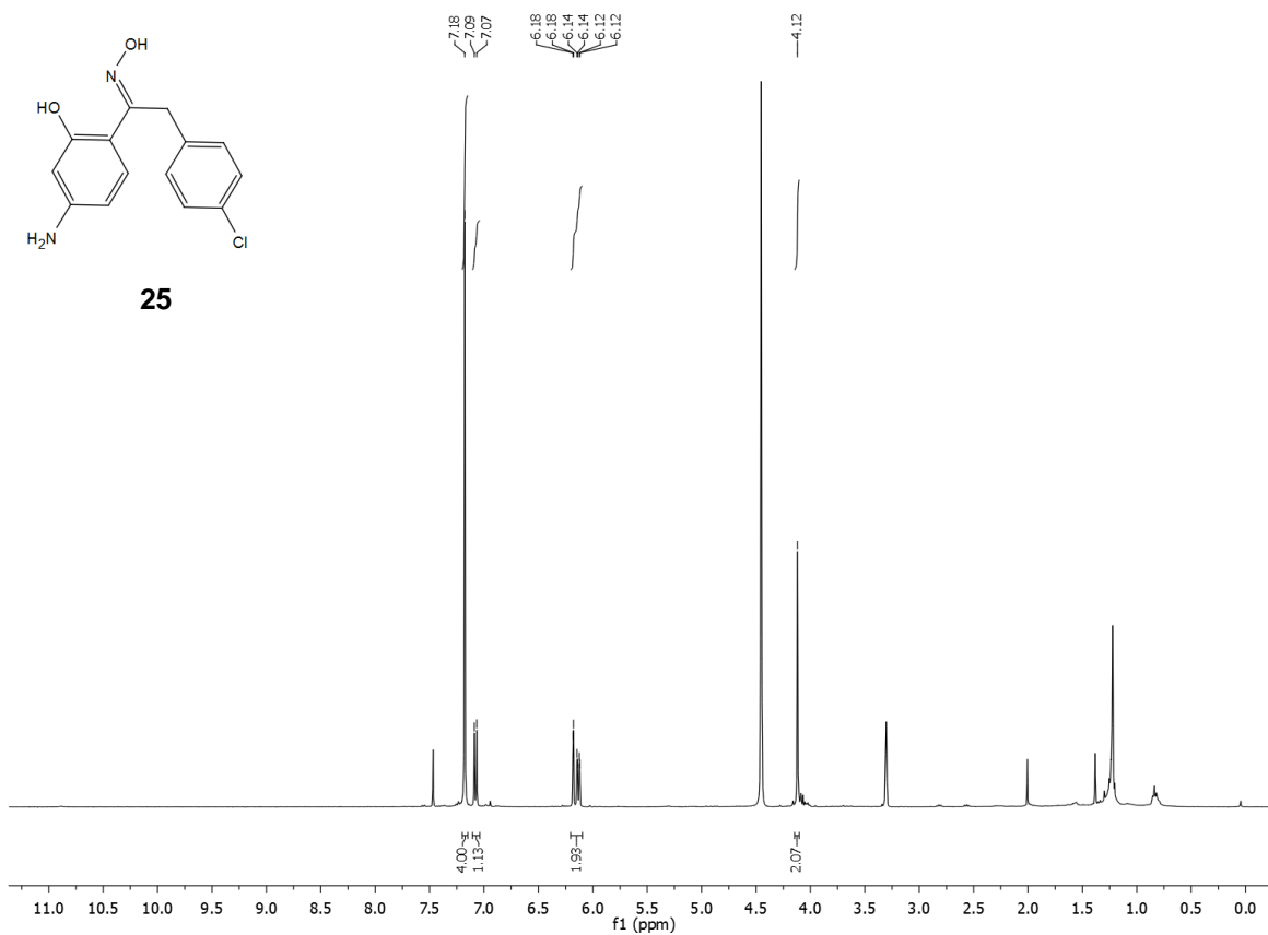
Spectrum 26: 1 H NMR of oxime 25 .
