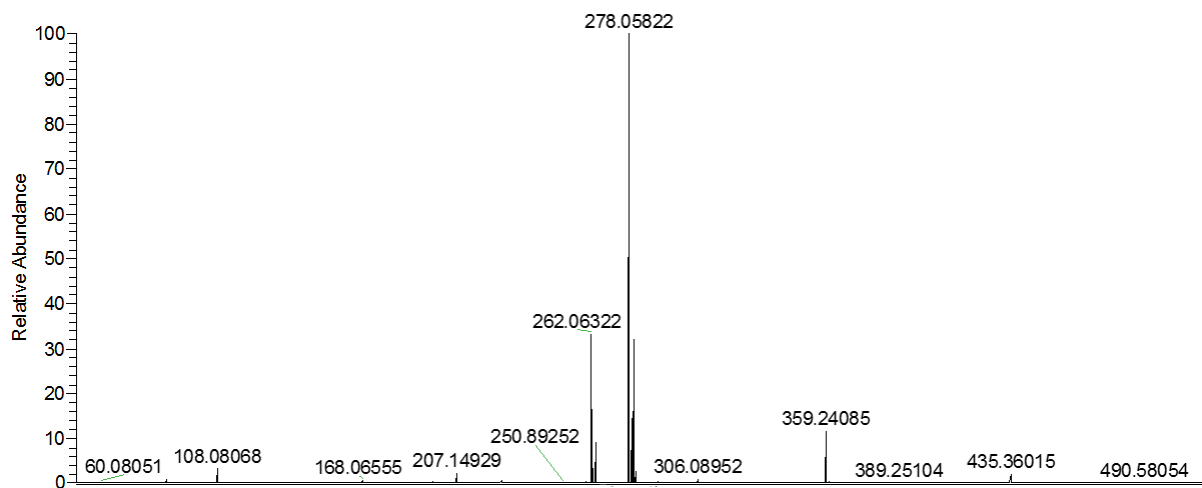
Spectrum 16: HR-ESI-MS spectrum of oxime 9 .
