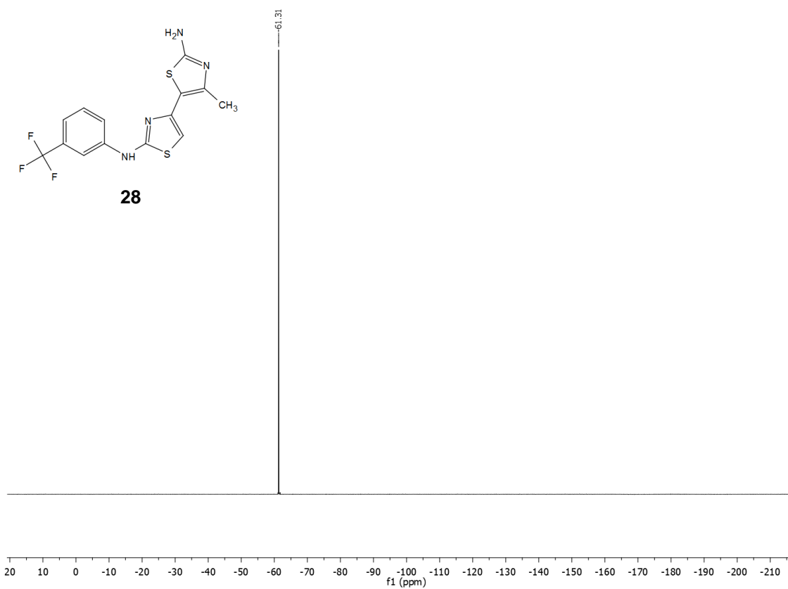
Spectrum 39: ^{19}\text{F} NMR of aminothiazole 28 .
