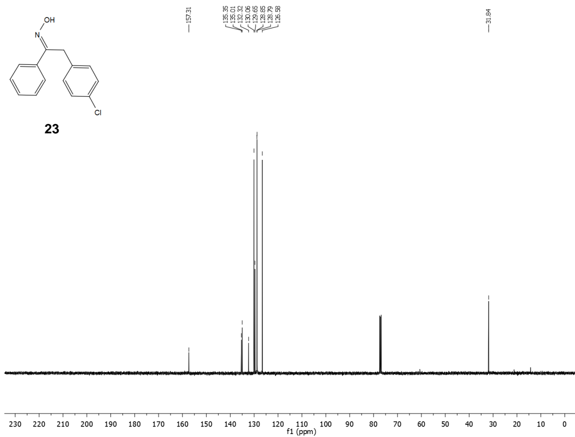
Spectrum 21: 13 C NMR of oxime 23 .
