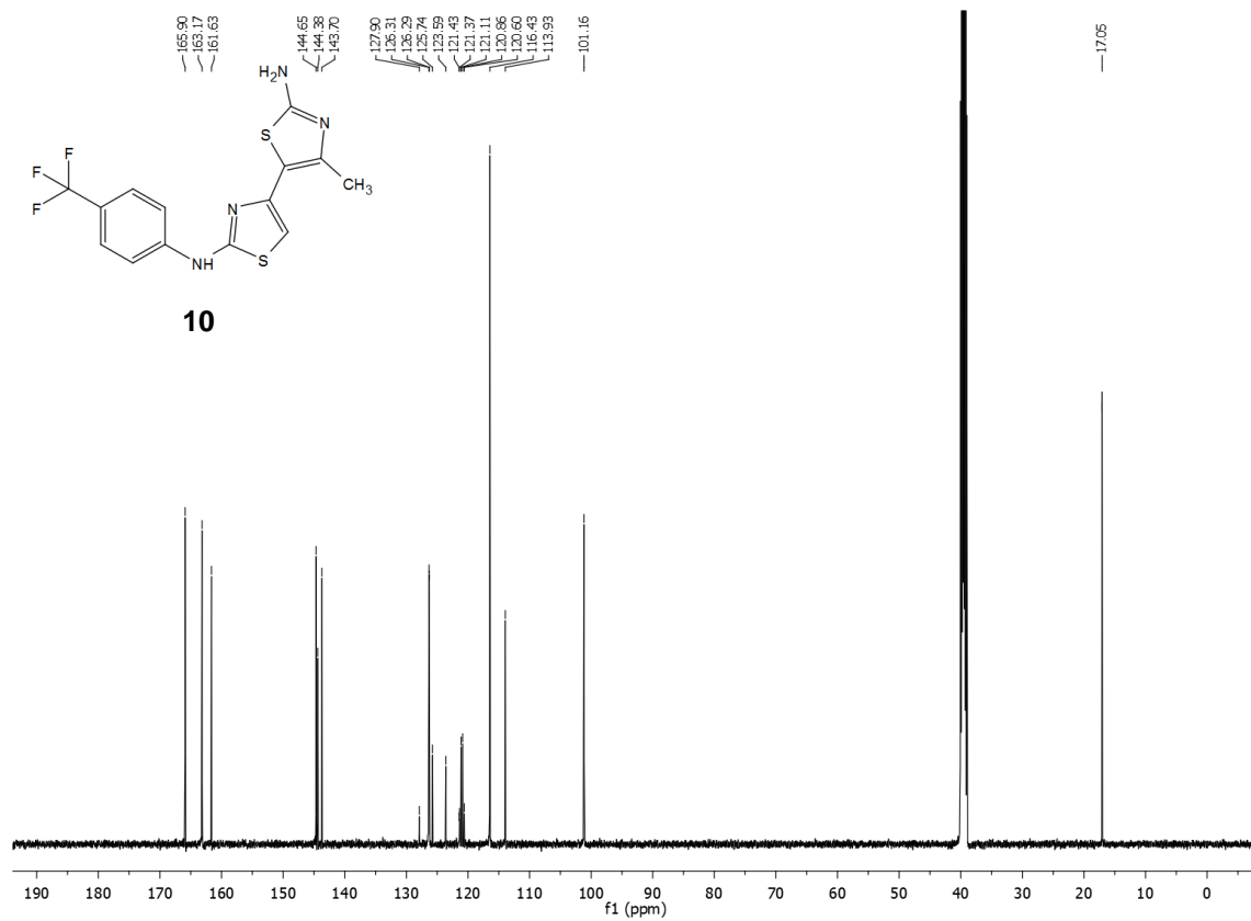
Spectrum 30: ^{13}\text{C} NMR of aminothiazole 10 .
