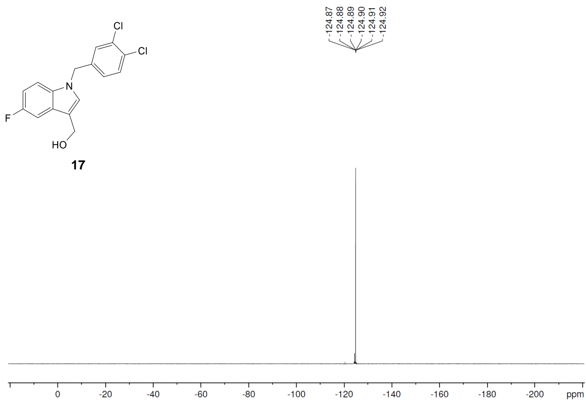
Spectrum 5: ^{13}\text{C} NMR of indole 17 .
