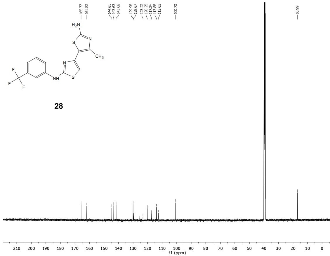
Spectrum 38: ^{13}\text{C} NMR of aminothiazole 28 .
