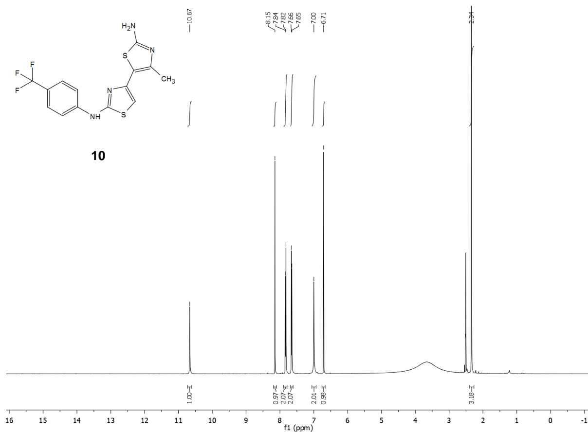
Spectrum 29: 1 H NMR of aminothiazole 10 .
