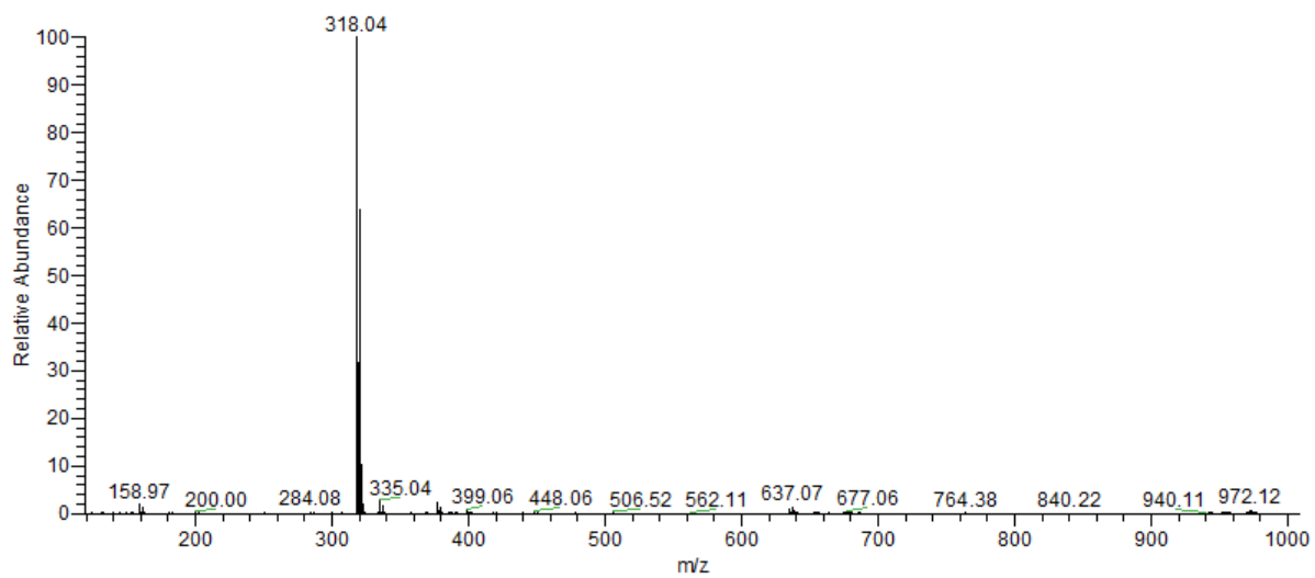
Spectrum 13: HR-ESI-MS spectrum of indole 19 .
