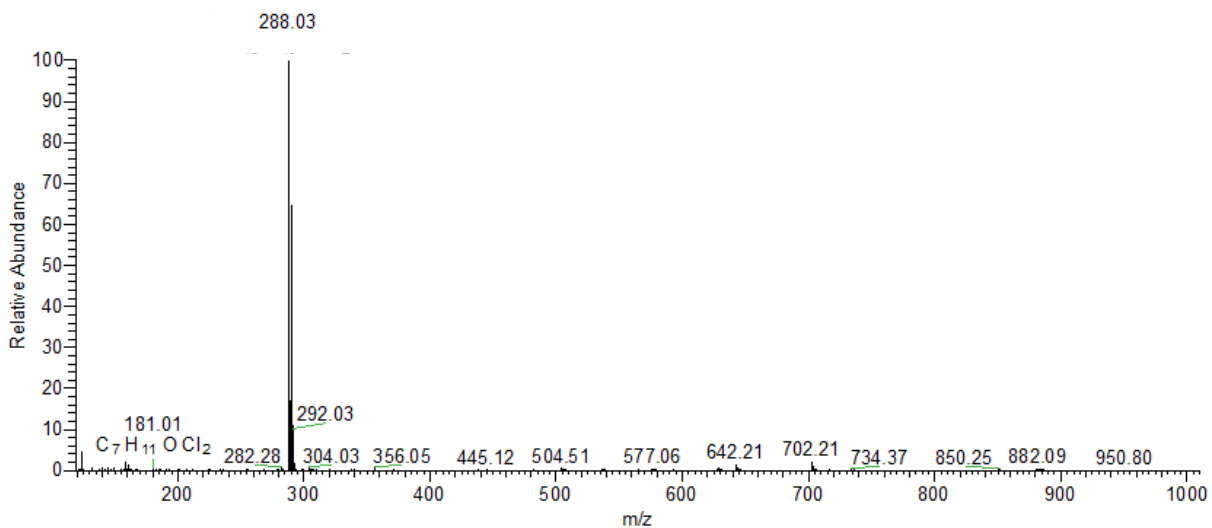
Spectrum 3: HR-ESI-MS spectrum of indole 7.
