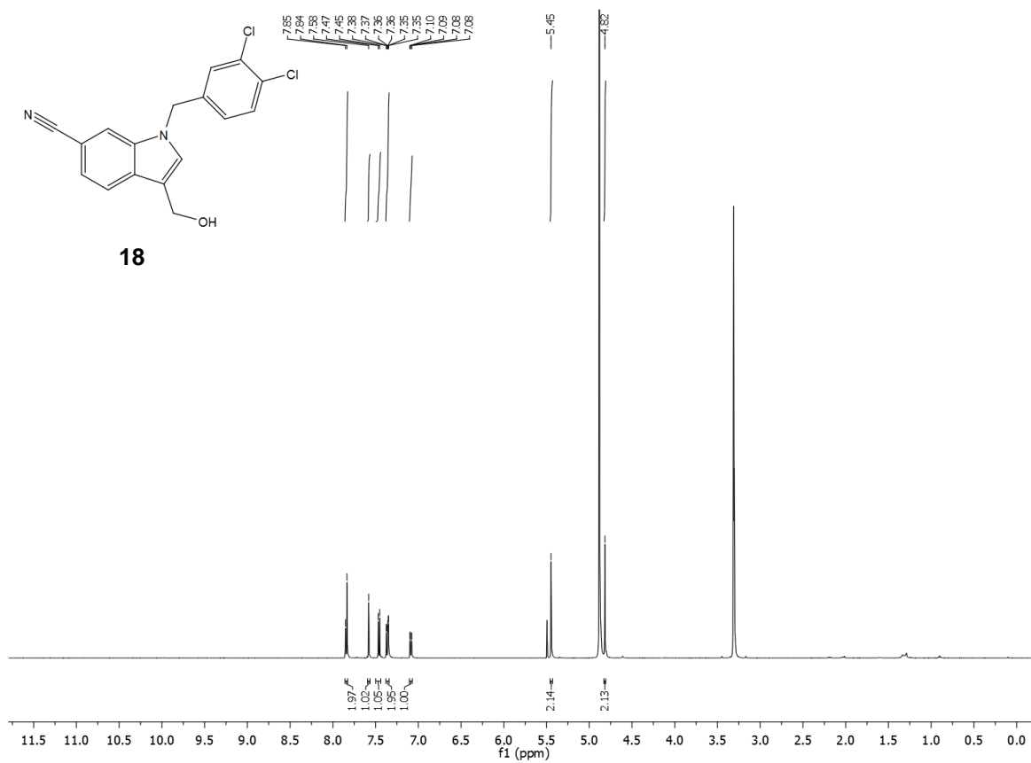
Spectrum 8: 1 H NMR of indole 18 .
