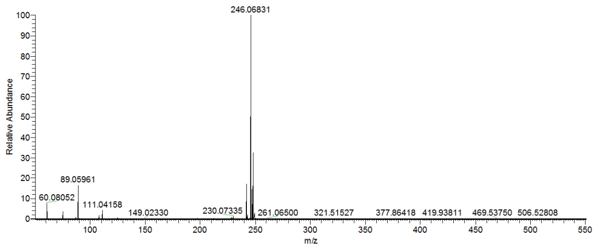
Spectrum 22: HR-ESI-MS spectrum of oxime 23 .
