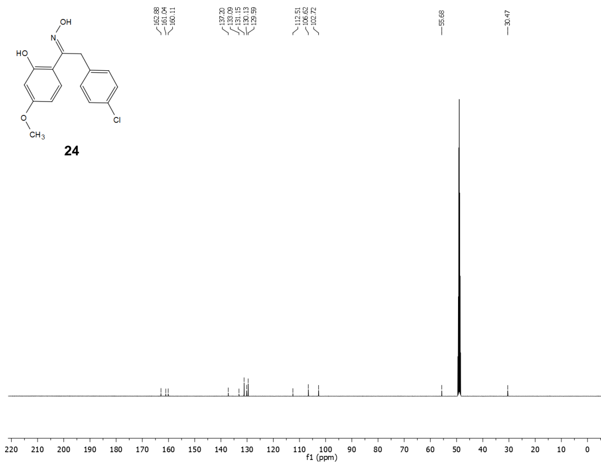
Spectrum 24: ^{13}\text{C} NMR of oxime 24 .
