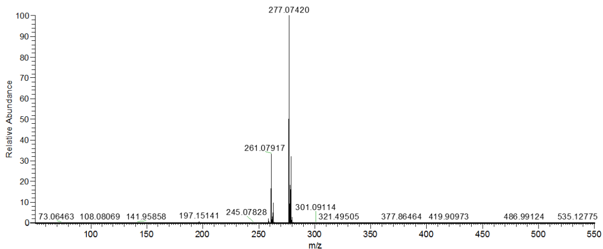
Spectrum 28: HR-ESI-MS spectrum of oxime 25 .
