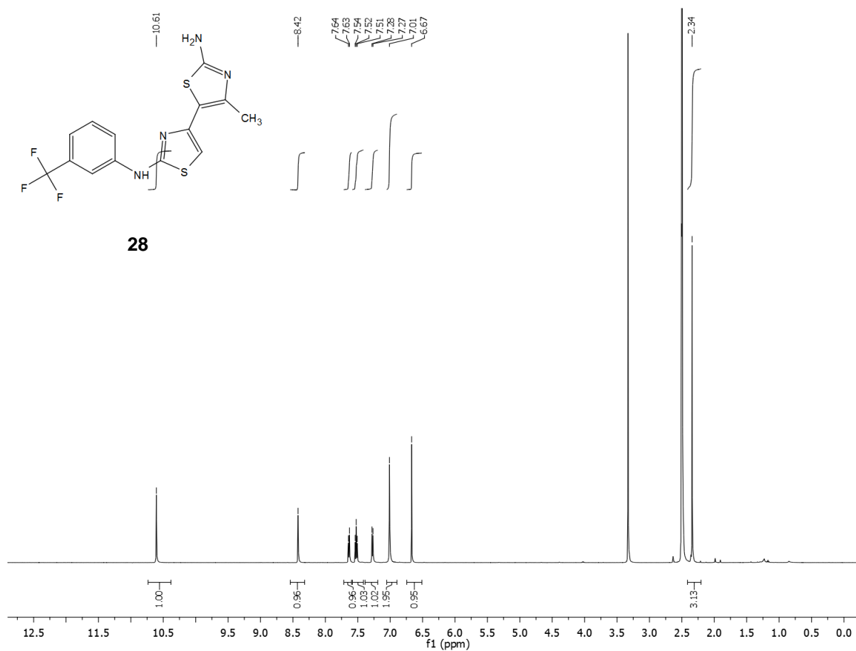
Spectrum 37: 1 H NMR of aminothiazole 28 .
