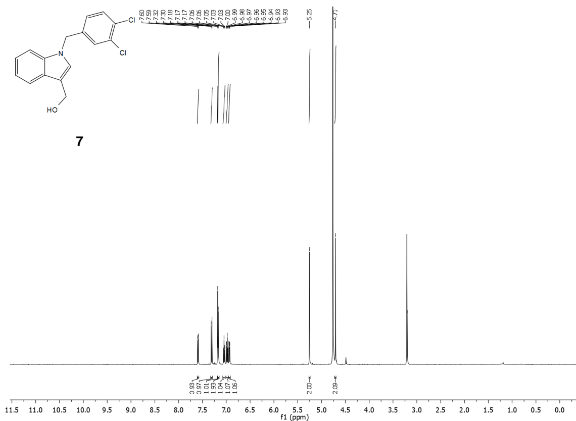
Spectrum 1: 1 H NMR of indole 7 .
