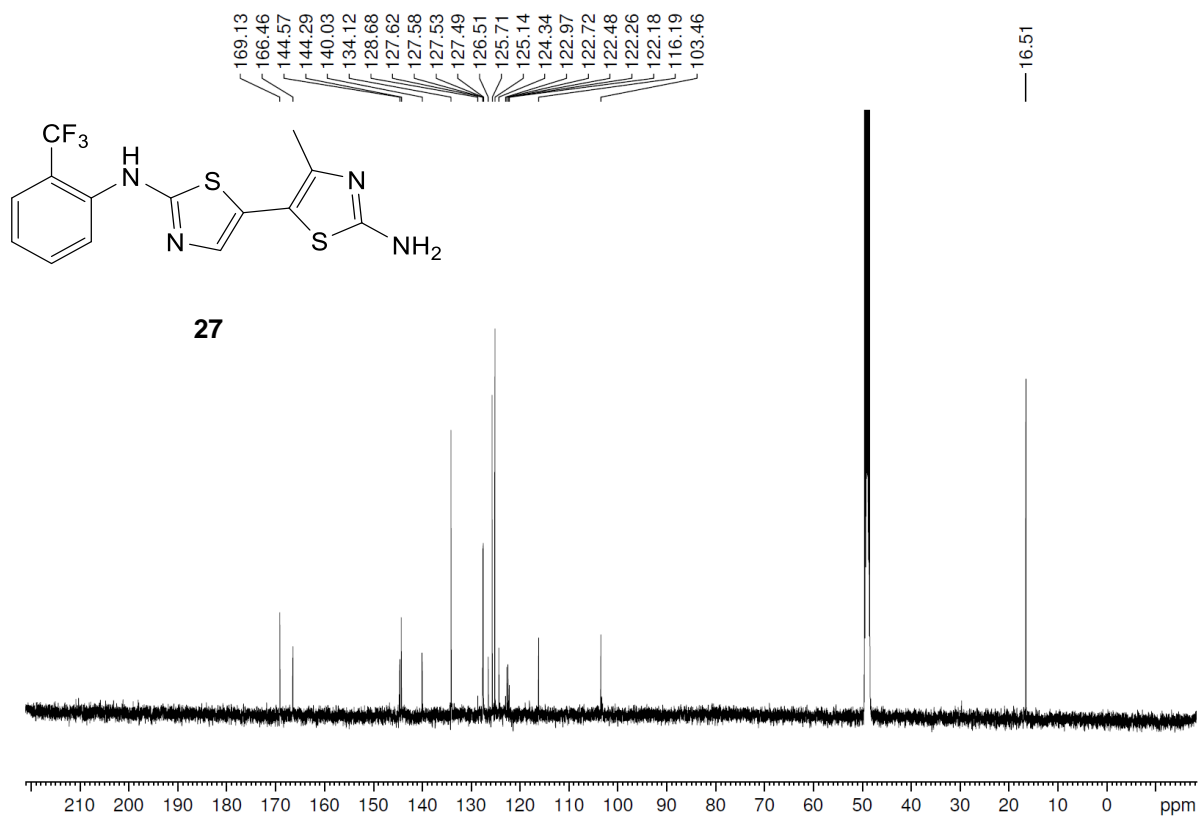
Spectrum 34: ^{13}\text{C} NMR of aminothiazole 27 .
