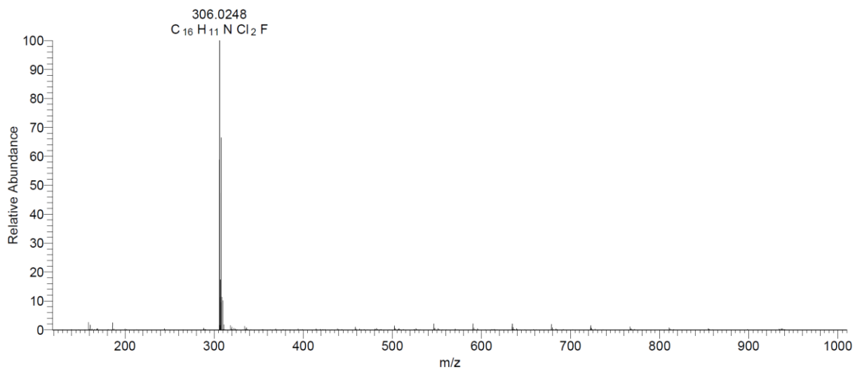
Spectrum 7: HR-ESI-MS spectrum of indole 17 .
