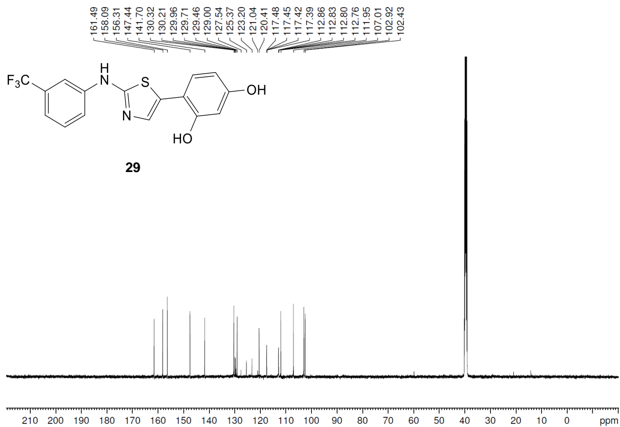
Spectrum 42: ^{13}\text{C} NMR of aminothiazole 29 .
