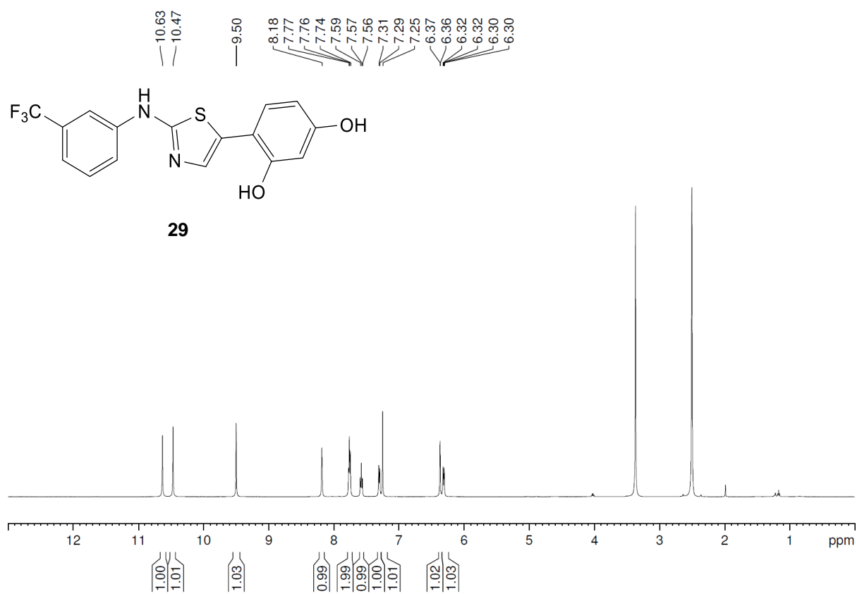
Spectrum 41: 1 H NMR of aminothiazole 29 .
