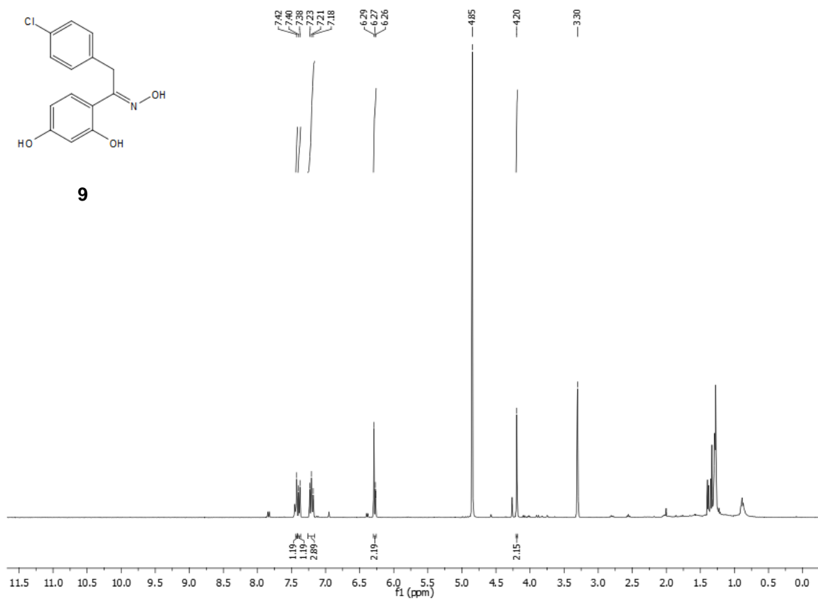
Spectrum 14: 1 H NMR of oxime 9.
