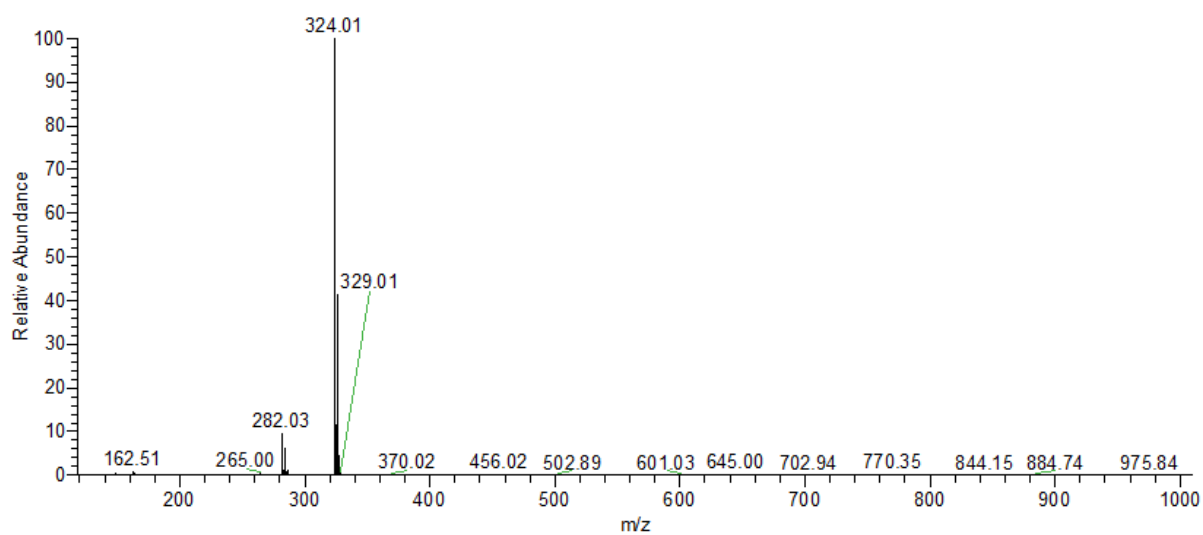
Spectrum 47: HR-ESI-MS spectrum of aminothiazole 30 .
