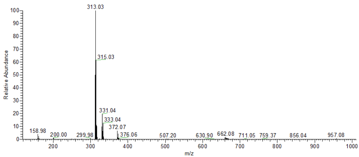
Spectrum 10: HR-ESI-MS spectrum of indole 18.
