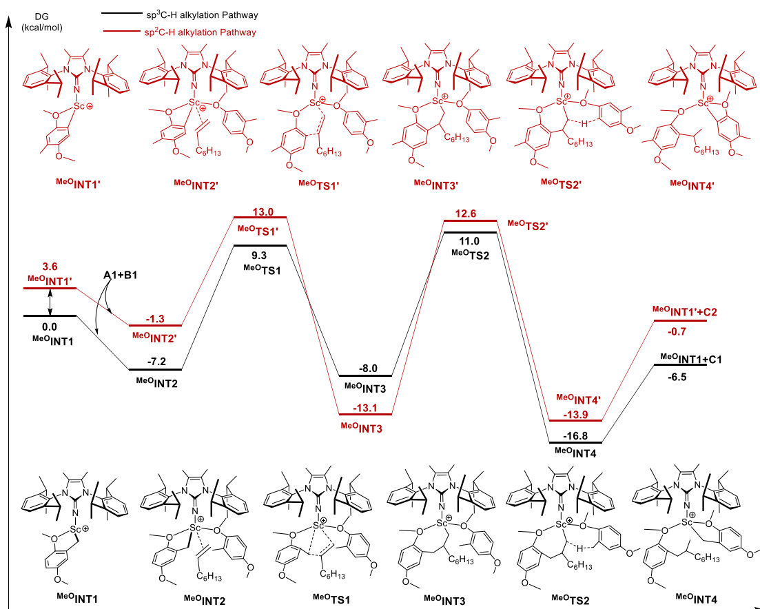
Figure S195. DFT-Calculated relative Gibbs free energies (in kcal/mol) of the \text{Csp}^3\text{-H} and \text{Csp}^2\text{-H} alkylation.
