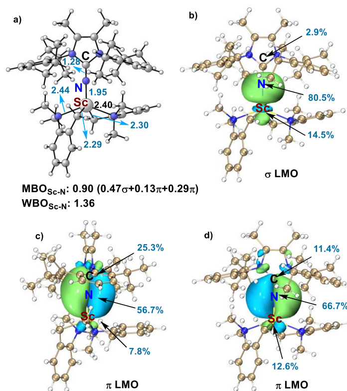
Figure S192. The Mayer bond order (MBO), Wiberg bond order (WBO) and the localized molecular orbitals of \sigma and \pi bond between the Sc and N atom (imidazolium) of the catalyst. (isovalue = 0.02)
