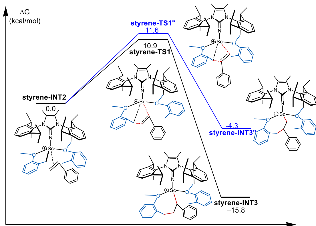
Figure S198. DFT-Calculated relative Gibbs free energies (in kcal/mol) of the reaction of 2-methylanisole with styrene.
