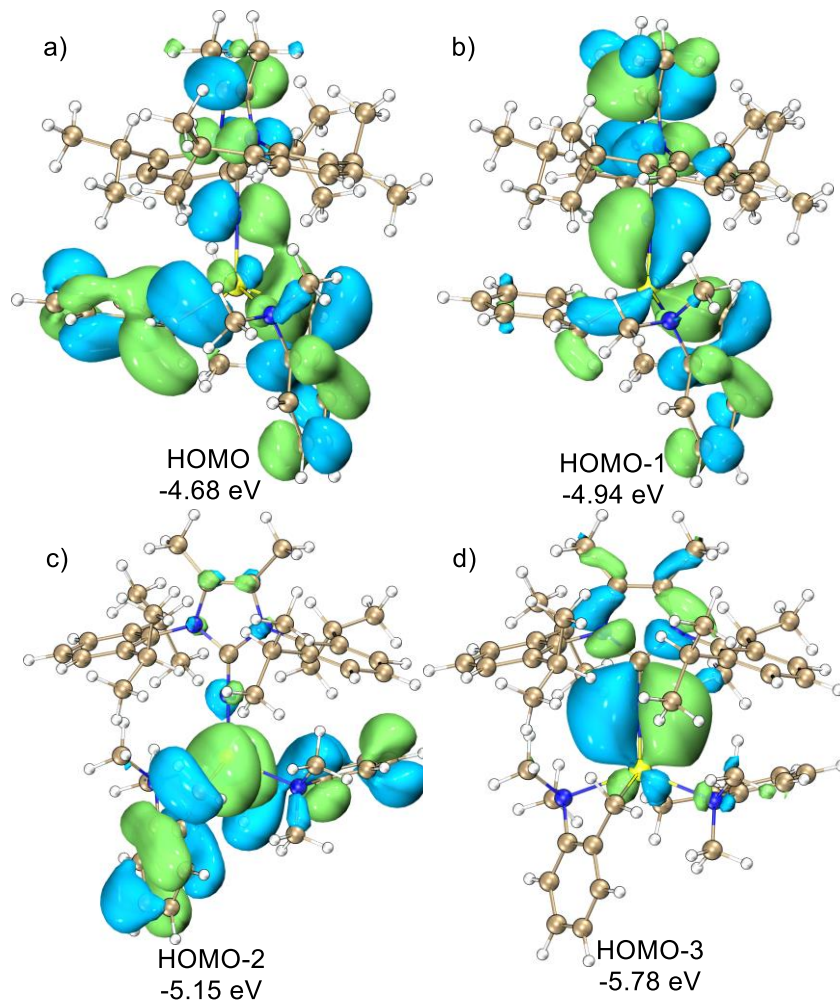
Figure S193. DFT calculated the four highest occupied molecular orbitals of the catalyst.
