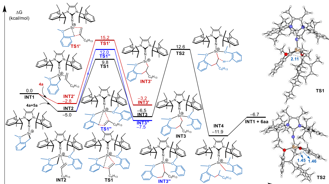
Figure S194. DFT-Calculated relative Gibbs free energies (in kcal/mol) of the anisole C–H alkylation.
