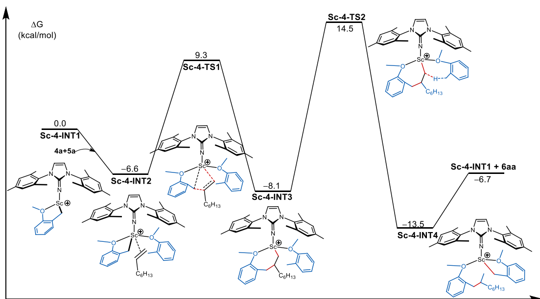
Figure S197. DFT-Calculated relative Gibbs free energies (in kcal/mol) of the Sc-4 catalyzed anisole C–H alkylation.
