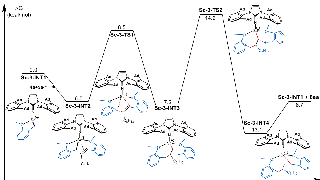
Figure S196. DFT-Calculated relative Gibbs free energies (in kcal/mol) of the Sc-3 catalyzed anisole C–H alkylation.
