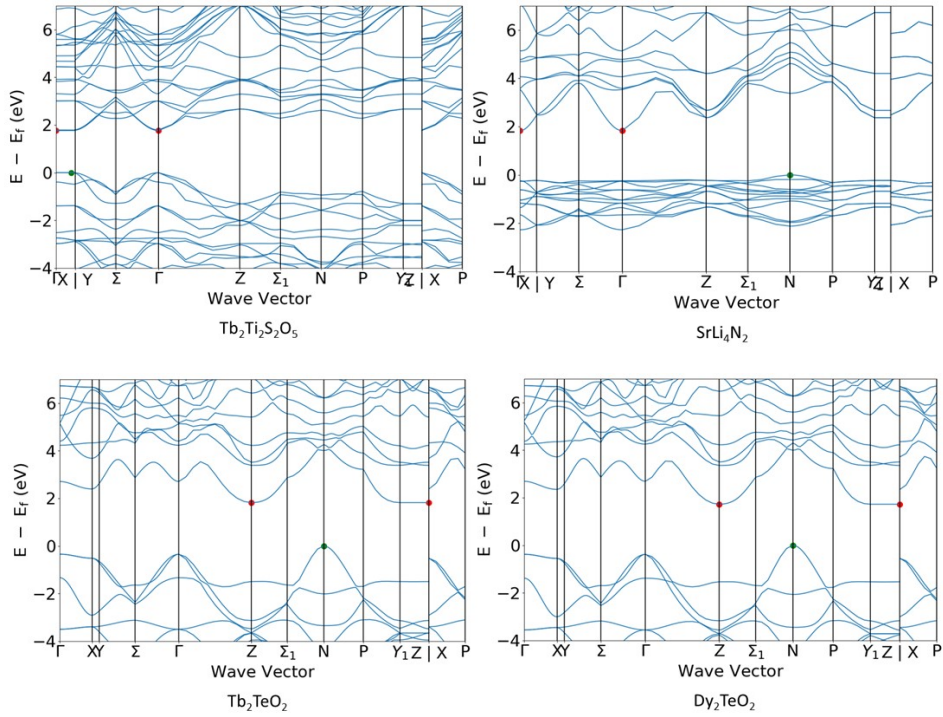
Figure S3. The band structures for the 11 final-candidate.
