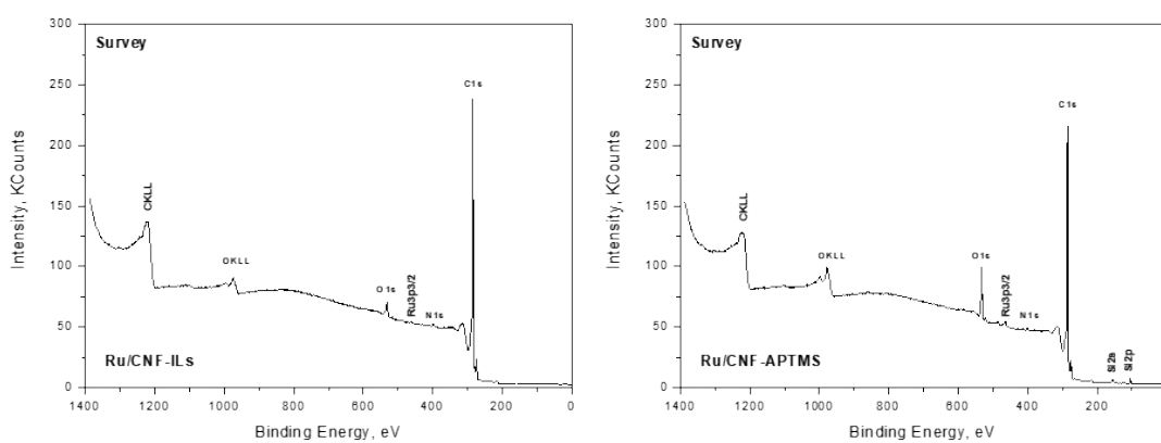
Figure S1. General XPS survey of Ru/CNF-ILs and Ru/CNF-APTMS
