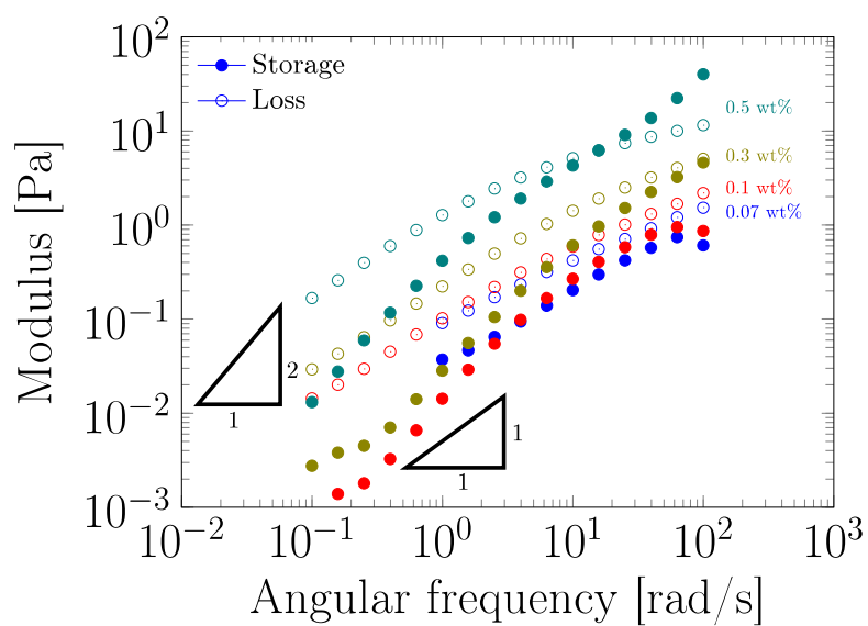
Fig. S1: Storage and loss modulus obtained via small amplitude oscillatory shear tests with an imposed deformation of 5%. The two slopes represent the scalings for the storage ( \propto \omega^2 ) and loss modulus ( \propto \omega ) in the terminal region.
