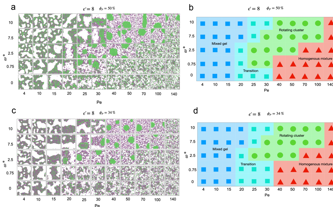
Figure S1. Comparison between two values of \phi_p = 50\% (a and b) and \phi_p = 34\% (c and d).
