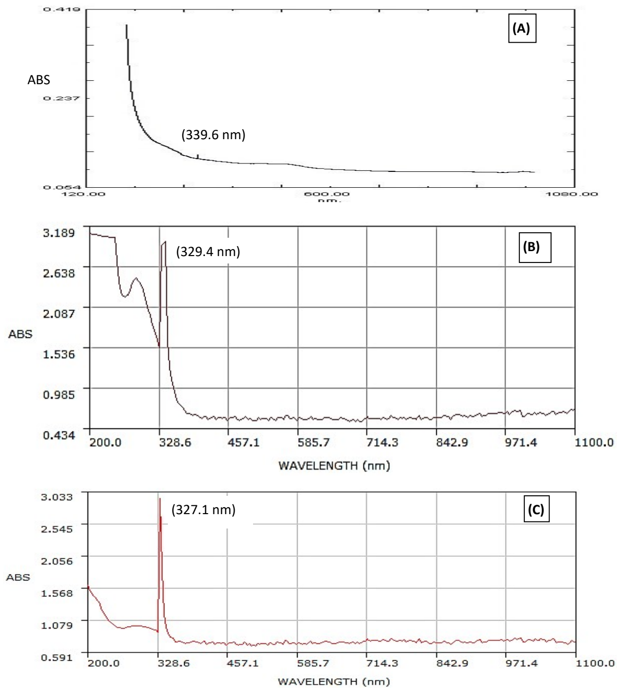
Fig. S1. UV-visible absorption spectra of \text{Co}_3\text{O}_4 QDs (A), PPy (B) and \text{Co}_3\text{O}_4@ PPy NCs (C).
