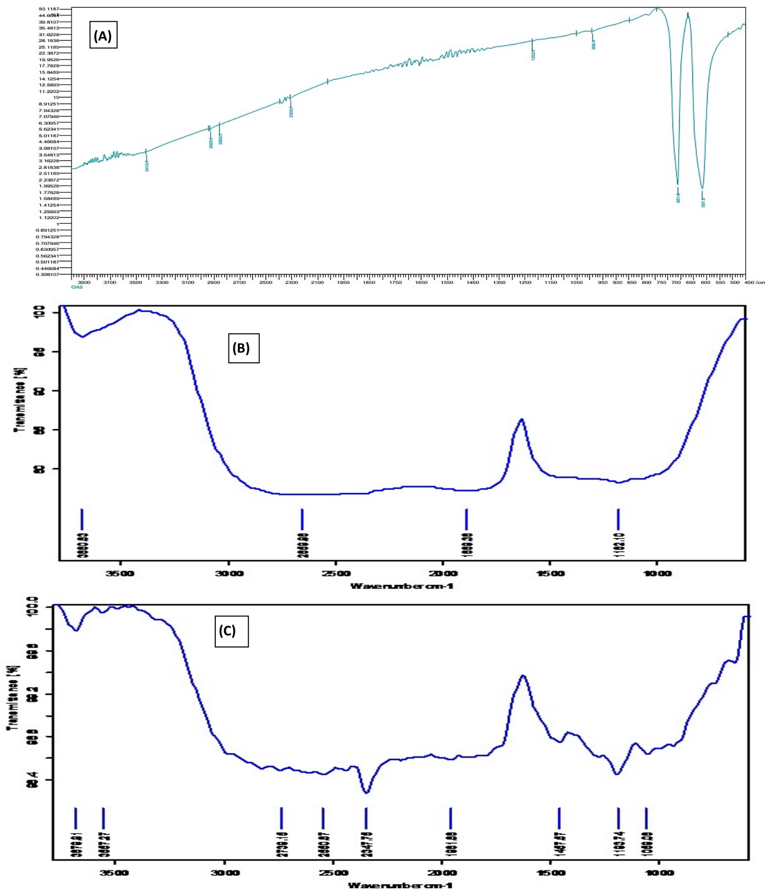
Fig. S3. FTIR spectra of Co 3 O 4 QDs (A), PPy (B), and Co 3 O 4 @PPy NCs (C).
